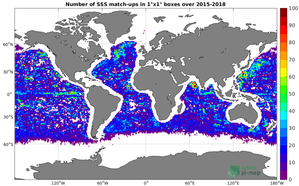
Figure 4: Number of SSS match-ups between Argo SSS and the SMAP-L3-RSS-V3-8DAY-RUNNING-70KM SSS product for the Global Ocean Pi-MEP region over 1°x1° boxes and for the full satellite product period.
