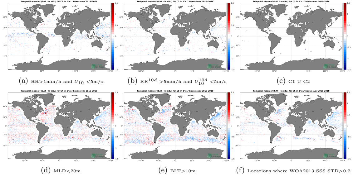
Figure 12: Temporal mean gridded over spatial boxes of size 1^\circ \times 1^\circ of \Delta\text{SSS} (SMAP-L3-RSS-V3-8DAY-RUNNING-70KM - Argo) for 6 different subdatasets corresponding to: RR > 1\text{mm/h} and U_{10} < 5\text{m/s} (a), RR^{10d} > 5\text{mm/h} and U_{10}^{10d} < 5\text{m/s} (b), C1 U C2 (c), MLD < 20\text{m} (d), BLT > 10\text{m} (e), Locations where WOA2013 SSS STD > 0.2 (f).
