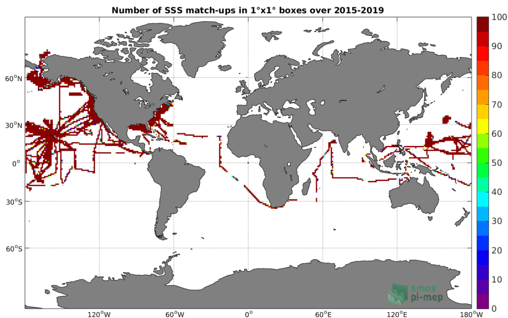
Figure 4: Number of SSS match-ups between TSG-SAMOS SSS and the SMAP-L3-RSS-V3-8DAY-RUNNING-40KM SSS product for the Global Ocean Pi-MEP region over 1^\circ \times 1^\circ boxes and for the full satellite product period.
