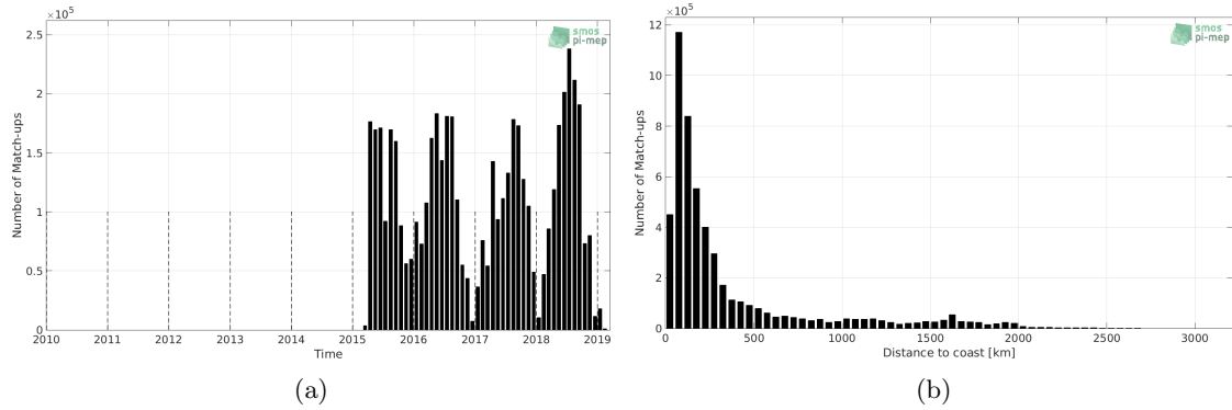
Figure 1: Number of match-ups between TSG-SAMOS and SMAP-L3-RSS-V3-8DAY-RUNNING-40KM SSS as a function of time (a) and as function of the distance to coast (b) over the Global Ocean Pi-MEP region and for the full satellite product period.
