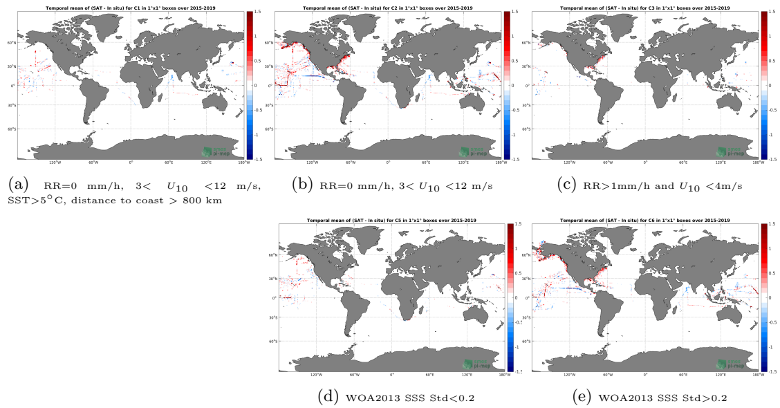
Figure 12: Temporal mean gridded over spatial boxes of size 1^\circ \times 1^\circ of \Delta SSS (SMAP-L3-RSS-V3-8DAY-RUNNING-40KM - TSG-SAMOS) for 5 different subdatasets corresponding to:RR=0 mm/h, 3 < U_{10} < 12 m/s, SST > 5^\circ\text{C} , distance to coast > 800 km (a), RR=0 mm/h, 3 < U_{10} < 12 m/s (b), RR > 1 mm/h and U_{10} < 4 m/s (c), WOA2013 SSS Std < 0.2 (d), WOA2013 SSS Std > 0.2 (e).
