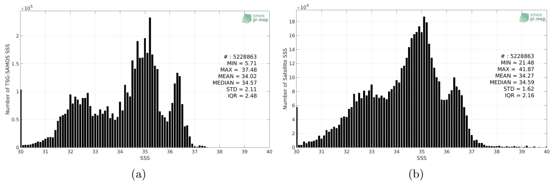
Figure 2: Histograms of SSS from TSG-SAMOS (a) and SMAP-L3-RSS-V3-8DAY-RUNNING-40KM (b) considering all match-up pairs per bins of 0.1 over the Global Ocean Pi-MEP region and for the full satellite product period.
