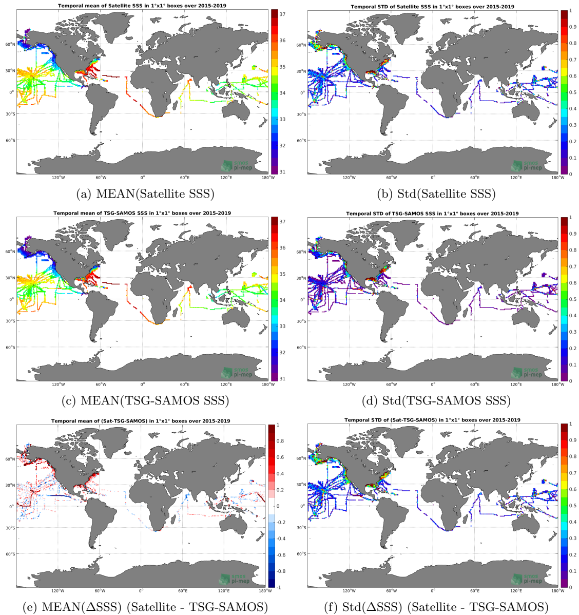
Figure 6: Temporal mean (left) and Std (right) of SSS from SMAP-L3-RSS-V3-8DAY-RUNNING-40KM (top), TSG-SAMOS (middle), and of \Delta SSS (Satellite - TSG-SAMOS). Only match-up pairs are used to generate these maps.
