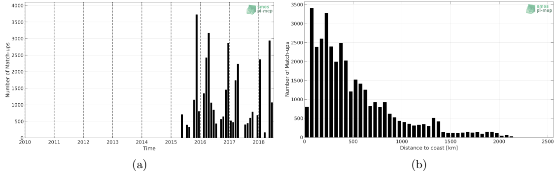
Figure 1: Number of match-ups between TSG-POLARSTERN and SMAP-L3-RSS-V3-8DAY-RUNNING-40KM SSS as a function of time (a) and as function of the distance to coast (b) over the Global Ocean Pi-MEP region and for the full satellite product period.
