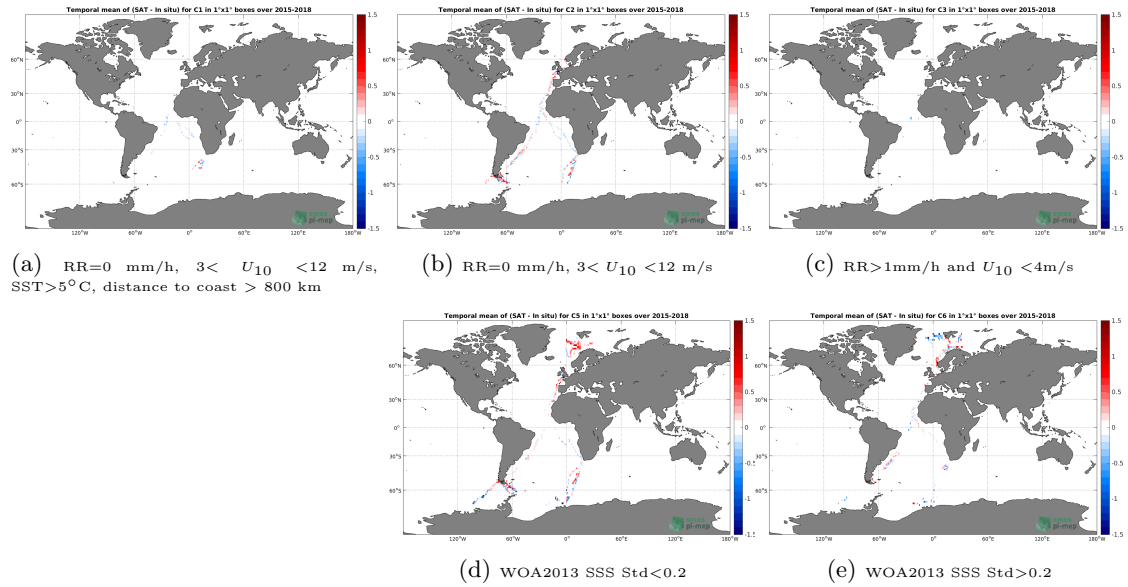
Figure 12: Temporal mean gridded over spatial boxes of size 1^\circ \times 1^\circ of \Delta SSS (SMAP-L3-RSS-V3-8DAY-RUNNING-40KM - TSG-POLARSTERN) for 5 different subdatasets corresponding to:RR=0 mm/h, 3 < U_{10} < 12 m/s, SST >5^\circ C, distance to coast > 800 km (a), RR=0 mm/h, 3 < U_{10} < 12 m/s (b), RR >1 mm/h and U_{10} < 4 m/s (c), WOA2013 SSS Std <0.2 (d), WOA2013 SSS Std >0.2 (e).
