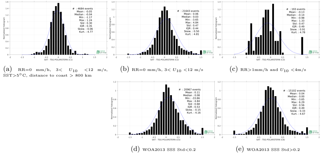
Figure 13: Normalized histogram of \Delta SSS (SMAP-L3-RSS-V3-8DAY-RUNNING-40KM - TSG-POLARSTERN) for 5 different subdatasets corresponding to: RR=0 mm/h, 3 < U_{10} < 12 m/s, SST>5°C, distance to coast > 800 km (a), RR=0 mm/h, 3 < U_{10} < 12 m/s (b), RR>1mm/h and U_{10} < 4 m/s (c), WOA2013 SSS Std<0.2 (d), WOA2013 SSS Std>0.2 (e).
