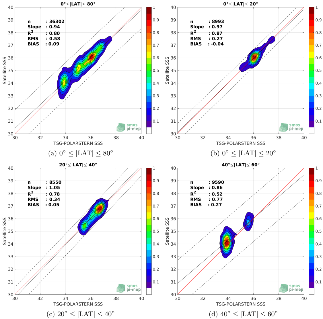
Figure 9: Contour maps of the concentration of SMAP-L3-RSS-V3-8DAY-RUNNING-40KM SSS (y-axis) versus TSG-POLARSTERN SSS (x-axis) at match-up pairs for different latitude bands. For each plot, the red line shows x=y . The black thin and dashed lines indicate a linear fit through the data cloud and the \pm 95\% confidence levels, respectively. The number match-up pairs n , the slope and R^2 coefficient of the linear fit, the root mean square (RMS) and the mean bias between satellite and in situ data are indicated for each latitude band in each plots.
