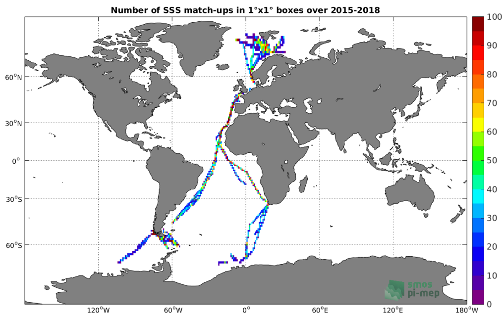
Figure 4: Number of SSS match-ups between TSG-POLARSTERN SSS and the SMAP-L3-RSS-V3-8DAY-RUNNING-40KM SSS product for the Global Ocean Pi-MEP region over 1^\circ \times 1^\circ boxes and for the full satellite product period.
