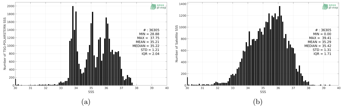
Figure 2: Histograms of SSS from TSG-POLARSTERN (a) and SMAP-L3-RSS-V3-8DAY-RUNNING-40KM (b) considering all match-up pairs per bins of 0.1 over the Global Ocean Pi-MEP region and for the full satellite product period.
