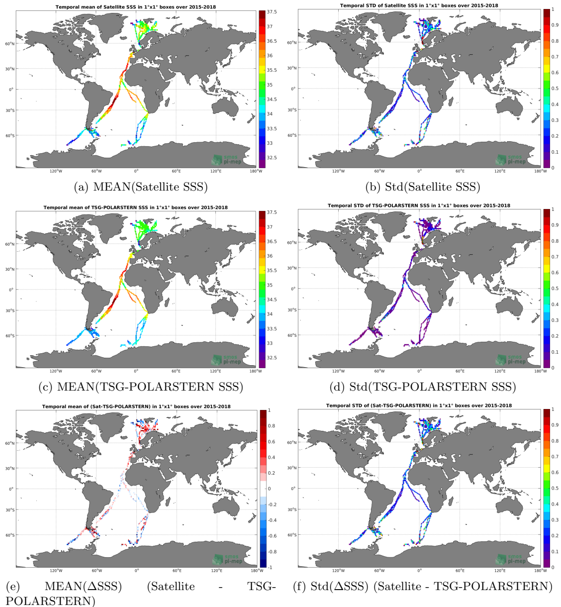
Figure 6: Temporal mean (left) and Std (right) of SSS from SMAP-L3-RSS-V3-8DAY-RUNNING-40KM (top), TSG-POLARSTERN (middle), and of \Delta SSS (Satellite - TSG-POLARSTERN). Only match-up pairs are used to generate these maps.
