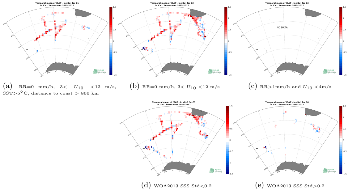
Figure 12: Temporal mean gridded over spatial boxes of size 1^\circ \times 1^\circ of \Delta SSS (SMAP-L3-RSS-V3-8DAY-RUNNING-40KM - TSG-NCEI-0170743) for 5 different subdatasets corresponding to:RR=0 mm/h, 3 < U_{10} < 12 m/s, SST >5^\circ C, distance to coast > 800 km (a), RR=0 mm/h, 3 < U_{10} < 12 m/s (b), RR >1 mm/h and U_{10} < 4 m/s (c), WOA2013 SSS Std <0.2 (d), WOA2013 SSS Std >0.2 (e).
