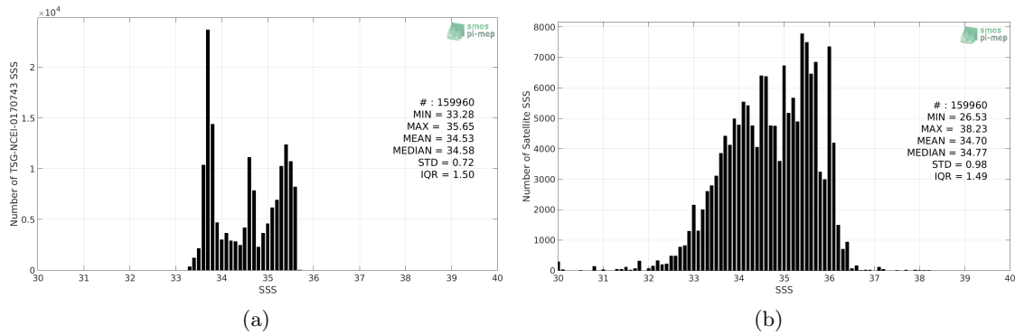
Figure 2: Histograms of SSS from TSG-NCEI-0170743 (a) and SMAP-L3-RSS-V3-8DAY-RUNNING-40KM (b) considering all match-up pairs per bins of 0.1 over the Global Ocean Pi-MEP region and for the full satellite product period.
