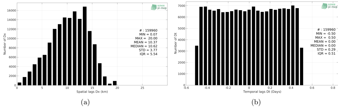
Figure 5: Histograms of the spatial (a) and temporal (b) lags between the time of the TSG-NCEI-0170743 measurements and the date of the corresponding SMAP-L3-RSS-V3-8DAY-RUNNING-40KM SSS product.
