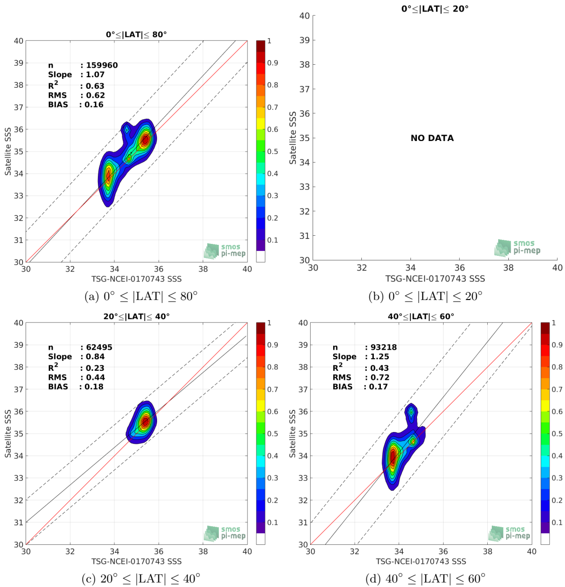
Figure 9: Contour maps of the concentration of SMAP-L3-RSS-V3-8DAY-RUNNING-40KM SSS (y-axis) versus TSG-NCEI-0170743 SSS (x-axis) at match-up pairs for different latitude bands. For each plot, the red line shows x=y . The black thin and dashed lines indicate a linear fit through the data cloud and the \pm 95\% confidence levels, respectively. The number match-up pairs n , the slope and R^2 coefficient of the linear fit, the root mean square (RMS) and the mean bias between satellite and in situ data are indicated for each latitude band in each plots.
