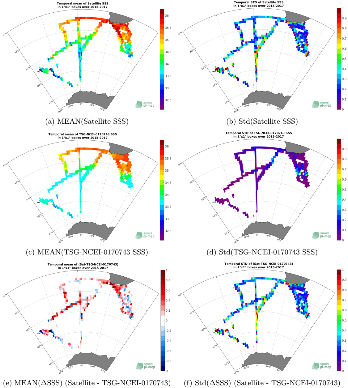
Figure 6: Temporal mean (left) and Std (right) of SSS from SMAP-L3-RSS-V3-8DAY-RUNNING-40KM (top), TSG-NCEI-0170743 (middle), and of \Delta SSS (Satellite - TSG-NCEI-0170743). Only match-up pairs are used to generate these maps.
