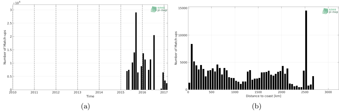
Figure 1: Number of match-ups between TSG-NCEI-0170743 and SMAP-L3-RSS-V3-8DAY-RUNNING-40KM SSS as a function of time (a) and as function of the distance to coast (b) over the Global Ocean Pi-MEP region and for the full satellite product period.
