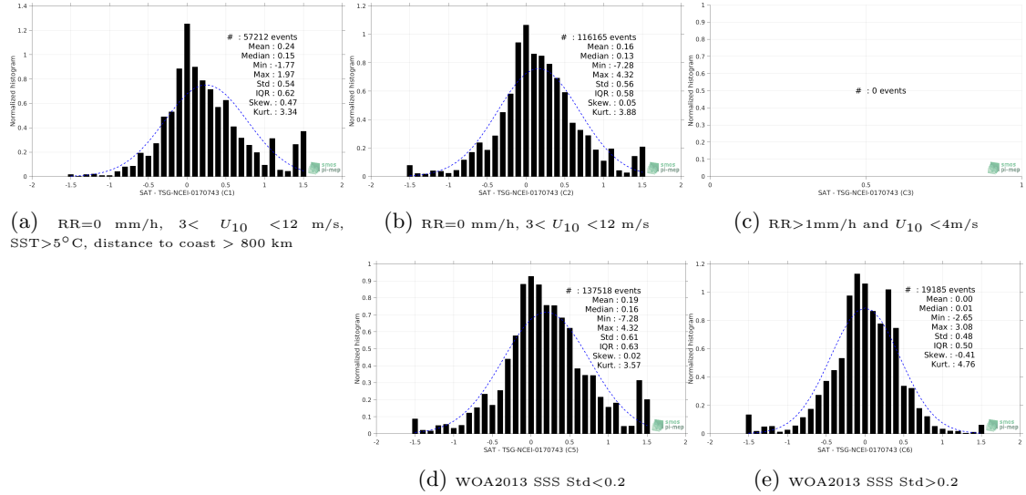
Figure 13: Normalized histogram of \Delta SSS (SMAP-L3-RSS-V3-8DAY-RUNNING-40KM - TSG-NCEI-0170743) for 5 different subdatasets corresponding to: RR=0 mm/h, 3 < U_{10} < 12 m/s, SST > 5°C, distance to coast > 800 km (a), RR=0 mm/h, 3 < U_{10} < 12 m/s (b), RR > 1mm/h and U_{10} < 4 m/s (c), WOA2013 SSS Std < 0.2 (d), WOA2013 SSS Std > 0.2 (e).
