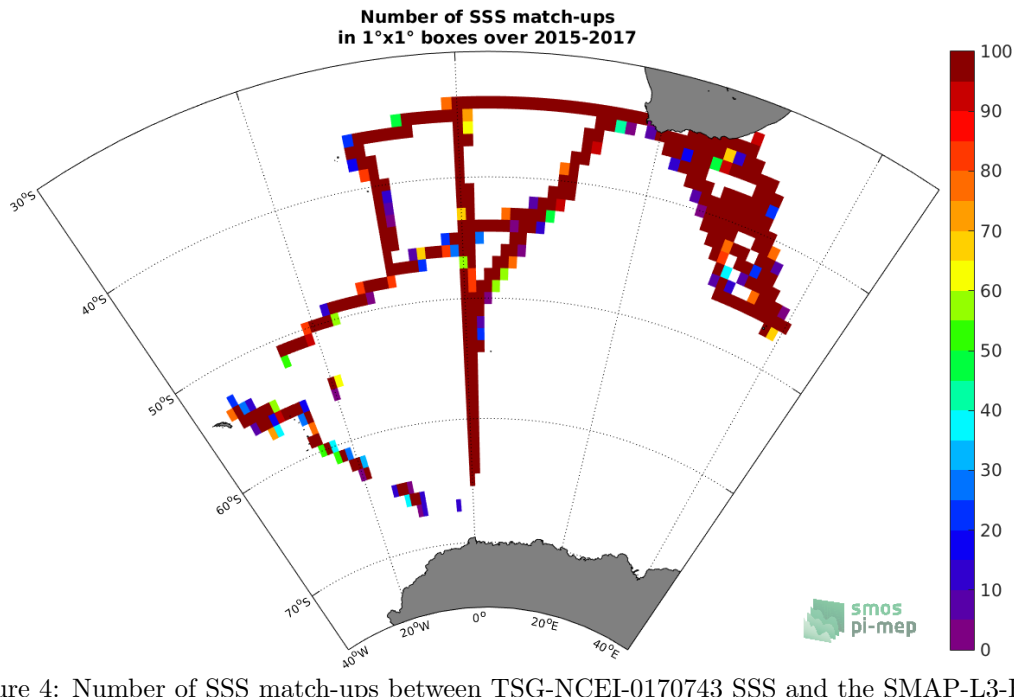
Figure 4: Number of SSS match-ups between TSG-NCEI-0170743 SSS and the SMAP-L3-RSS-V3-8DAY-RUNNING-40KM SSS product for the Global Ocean Pi-MEP region over 1^\circ \times 1^\circ boxes and for the full satellite product period.
