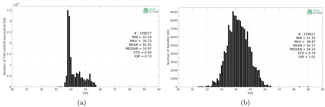
Figure 2: Histograms of SSS from TSG-LEGOS-Survostral (a) and SMAP-L3-RSS-V3-8DAY-RUNNING-40KM (b) considering all match-up pairs per bins of 0.1 over the Global Ocean Pi-MEP region and for the full satellite product period.
