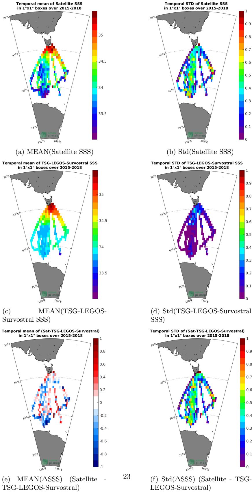
Figure 6: Temporal mean (left) and Std (right) of SSS from SMAP-L3-RSS-V3-8DAY-RUNNING-40KM (top), TSG-LEGOS-Survostral (middle), and of \Delta SSS (Satellite - TSG-LEGOS-Survostral). Only match-up pairs are used to generate these maps.
