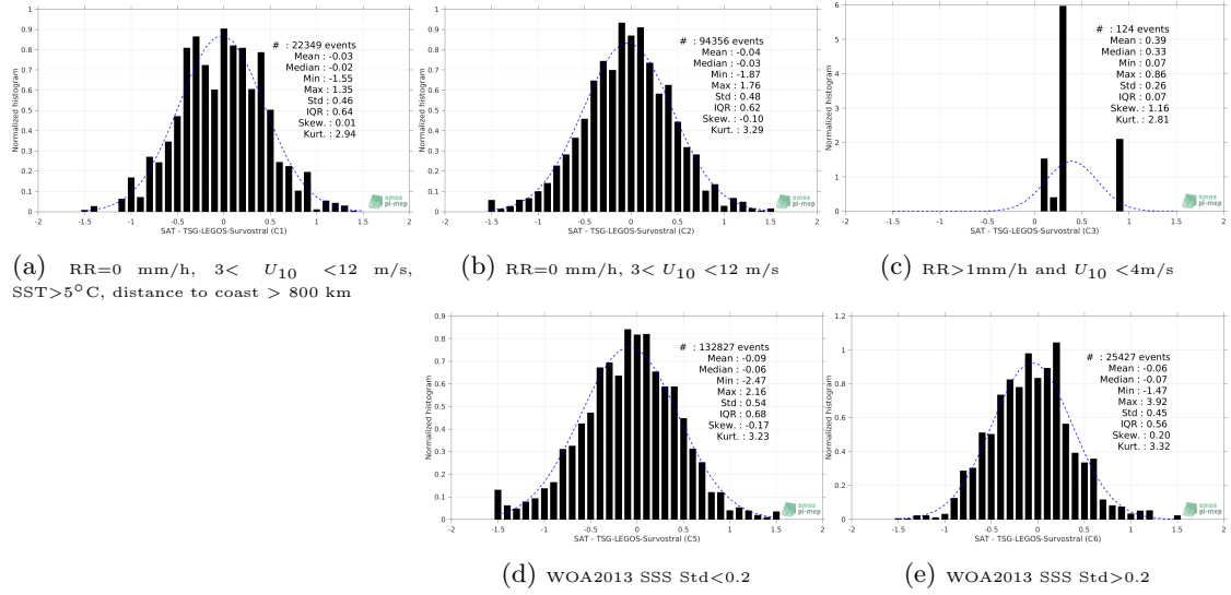
Figure 13: Normalized histogram of \Delta\text{SSS} (SMAP-L3-RSS-V3-8DAY-RUNNING-40KM - TSG-LEGOS-Survostral) for 5 different subdatasets corresponding to: RR=0 mm/h, 3 < U_{10} < 12 m/s, SST>5°C, distance to coast > 800 km (a), RR=0 mm/h, 3 < U_{10} < 12 m/s (b), RR>1mm/h and U_{10} < 4 m/s (c), WOA2013 SSS Std<0.2 (d), WOA2013 SSS Std>0.2 (e).
