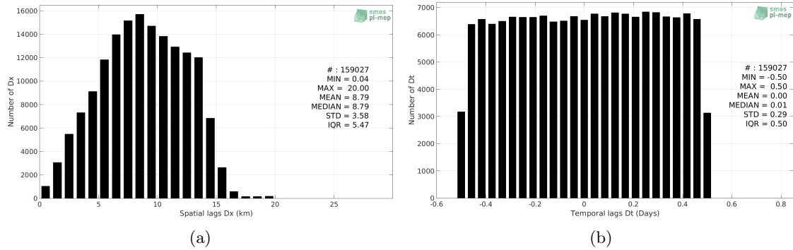
Figure 5: Histograms of the spatial (a) and temporal (b) lags between the time of the TSG-LEGOS-Survostral measurements and the date of the corresponding SMAP-L3-RSS-V3-8DAY-RUNNING-40KM SSS product.
