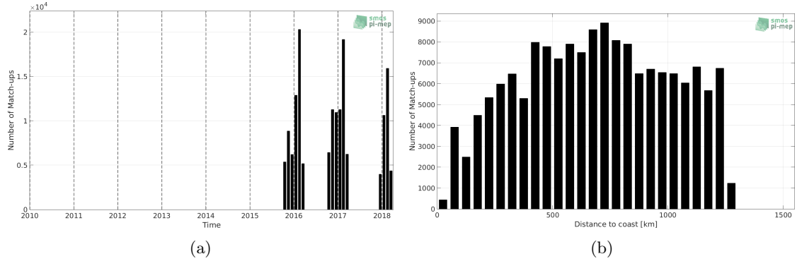
Figure 1: Number of match-ups between TSG-LEGOS-Survostral and SMAP-L3-RSS-V3-8DAY-RUNNING-40KM SSS as a function of time (a) and as function of the distance to coast (b) over the Global Ocean Pi-MEP region and for the full satellite product period.
