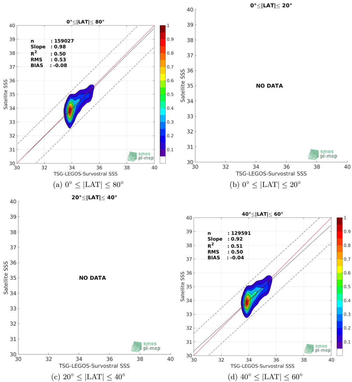
Figure 9: Contour maps of the concentration of SMAP-L3-RSS-V3-8DAY-RUNNING-40KM SSS (y-axis) versus TSG-LEGOS-Survostral SSS (x-axis) at match-up pairs for different latitude bands. For each plot, the red line shows x=y . The black thin and dashed lines indicate a linear fit through the data cloud and the \pm 95\% confidence levels, respectively. The number match-up pairs n , the slope and R^2 coefficient of the linear fit, the root mean square (RMS) and the mean bias between satellite and in situ data are indicated for each latitude band in each plots.
