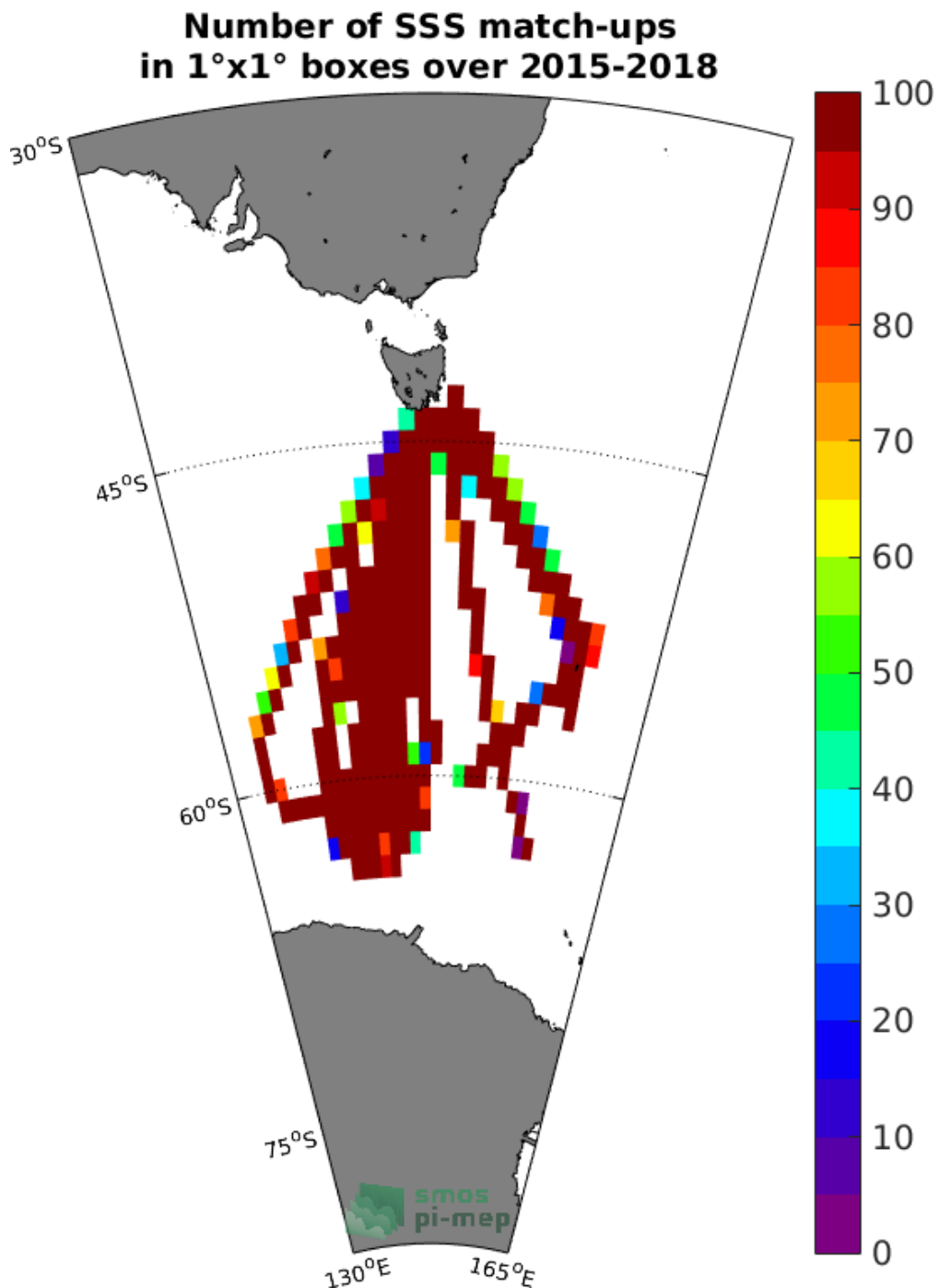
Figure 4: Number of SSS match-ups between TSG-LEGOS-Survostral SSS and the SMAP-L3-RSS-V3-8DAY-RUNNING-40KM SSS product for the Global Ocean Pi-MEP region over 1°x1° boxes and for the full satellite product period.
