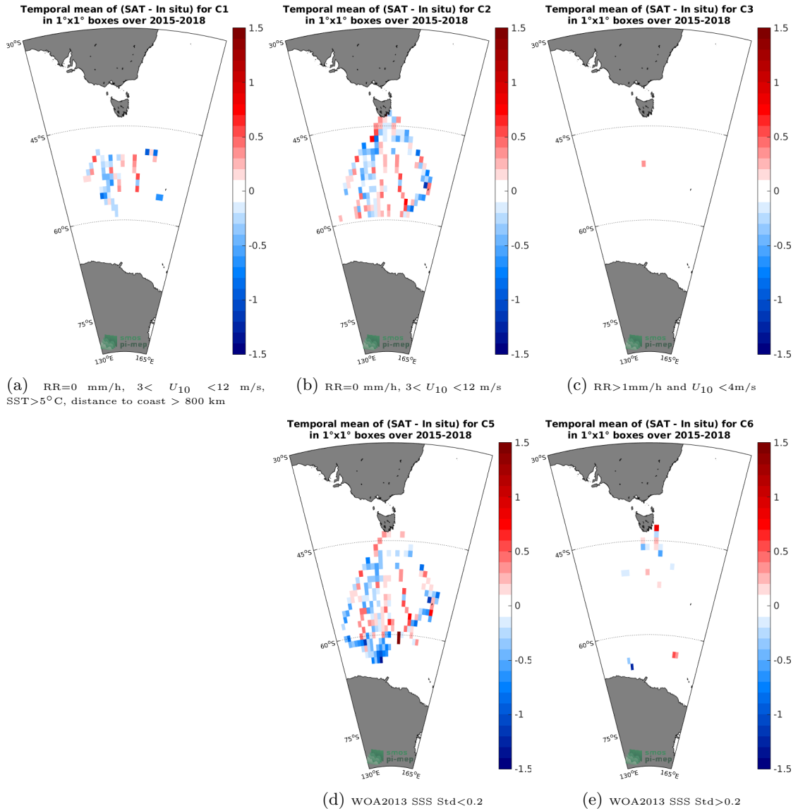
Figure 12: Temporal mean gridded over spatial boxes of size 1°x1° of \Delta SSS (SMAP-L3-RSS-V3-8DAY-RUNNING-40KM - TSG-LEGOS-Survostral) for 5 different subdatasets corresponding to:RR=0 mm/h, 3 < U_{10} < 12 m/s, SST>5°C, distance to coast > 800 km (a), RR=0 mm/h, 3 < U_{10} < 12 m/s (b), RR>1mm/h and U_{10} < 4 m/s (c), WOA2013 SSS Std<0.2 (d), WOA2013 SSS Std>0.2 (e).
