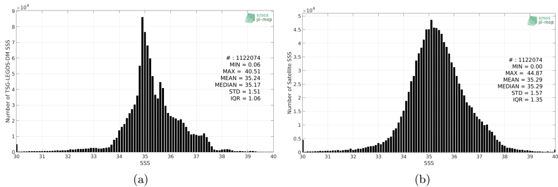
Figure 2: Histograms of SSS from TSG-LEGOS-DM (a) and SMAP-L3-RSS-V3-8DAY-RUNNING-40KM (b) considering all match-up pairs per bins of 0.1 over the Global Ocean Pi-MEP region and for the full satellite product period.
