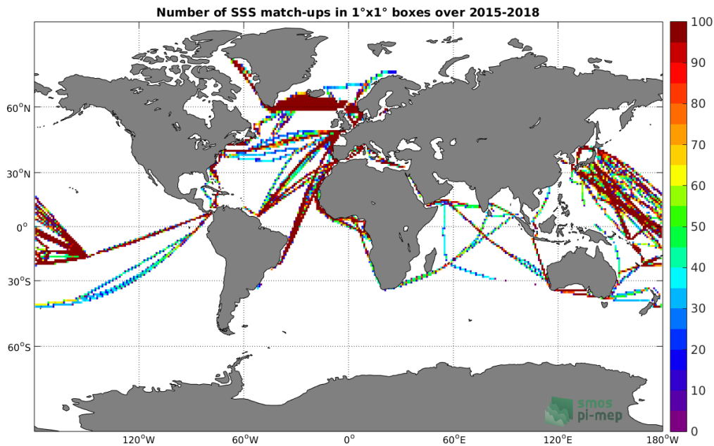
Figure 4: Number of SSS match-ups between TSG-LEGOS-DM SSS and the SMAP-L3-RSS-V3-8DAY-RUNNING-40KM SSS product for the Global Ocean Pi-MEP region over 1^\circ \times 1^\circ boxes and for the full satellite product period.
