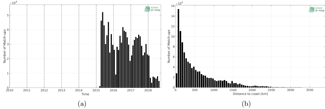
Figure 1: Number of match-ups between TSG-LEGOS-DM and SMAP-L3-RSS-V3-8DAY-RUNNING-40KM SSS as a function of time (a) and as function of the distance to coast (b) over the Global Ocean Pi-MEP region and for the full satellite product period.
