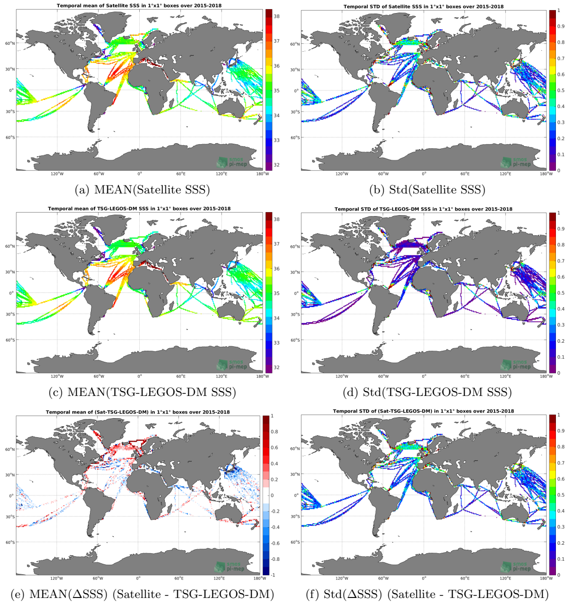
Figure 6: Temporal mean (left) and Std (right) of SSS from SMAP-L3-RSS-V3-8DAY-RUNNING-40KM (top), TSG-LEGOS-DM (middle), and of \Delta SSS (Satellite - TSG-LEGOS-DM). Only match-up pairs are used to generate these maps.
