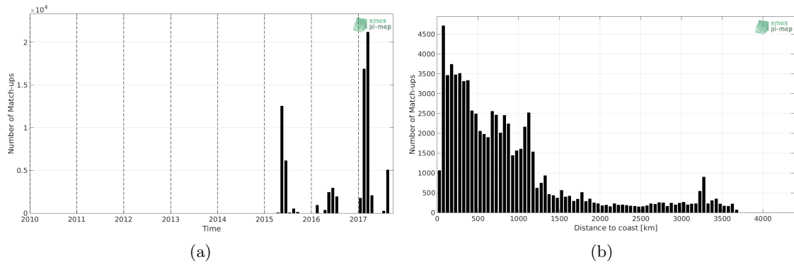
Figure 1: Number of match-ups between TSG-GOSUD-Sailing-ship and SMAP-L3-RSS-V3-8DAY-RUNNING-40KM SSS as a function of time (a) and as function of the distance to coast (b) over the Global Ocean Pi-MEP region and for the full satellite product period.
