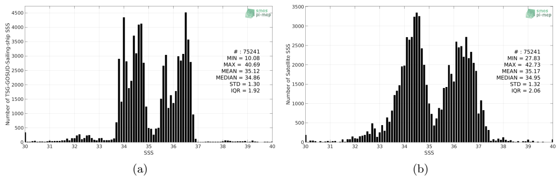
Figure 2: Histograms of SSS from TSG-GOSUD-Sailing-ship (a) and SMAP-L3-RSS-V3-8DAY-RUNNING-40KM (b) considering all match-up pairs per bins of 0.1 over the Global Ocean Pi-MEP region and for the full satellite product period.
