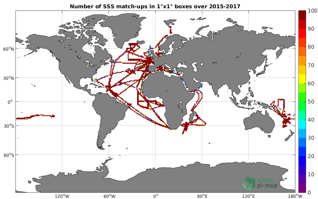
Figure 4: Number of SSS match-ups between TSG-GOSUD-Research-vessel SSS and the SMAP-L3-RSS-V3-8DAY-RUNNING-40KM SSS product for the Global Ocean Pi-MEP region over 1°x1° boxes and for the full satellite product period.
