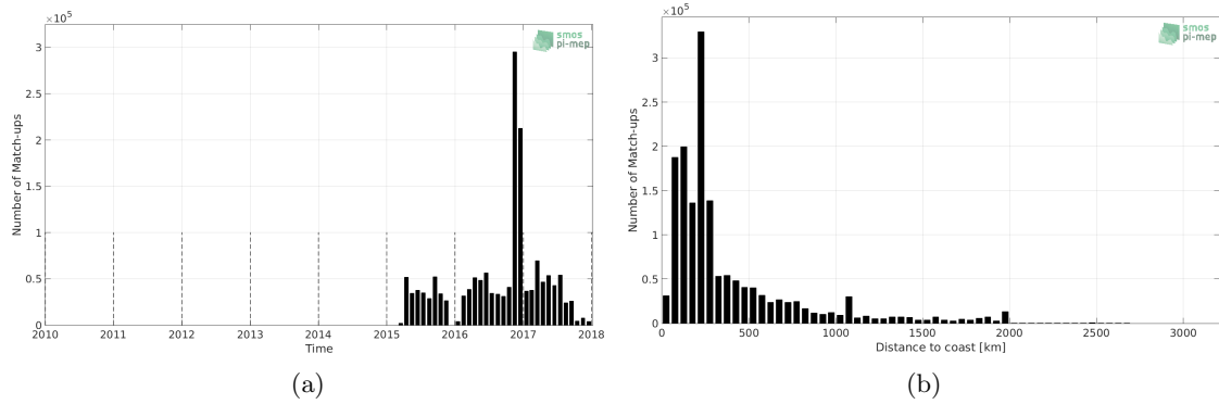
Figure 1: Number of match-ups between TSG-GOSUD-Research-vessel and SMAP-L3-RSS-V3-8DAY-RUNNING-40KM SSS as a function of time (a) and as function of the distance to coast (b) over the Global Ocean Pi-MEP region and for the full satellite product period.
