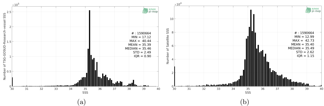
Figure 2: Histograms of SSS from TSG-GOSUD-Research-vessel (a) and SMAP-L3-RSS-V3-8DAY-RUNNING-40KM (b) considering all match-up pairs per bins of 0.1 over the Global Ocean Pi-MEP region and for the full satellite product period.
