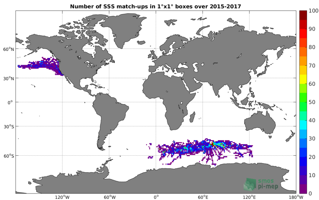
Figure 4: Number of SSS match-ups between Sea mammals SSS and the SMAP-L3-RSS-V3-8DAY-RUNNING-40KM SSS product for the Global Ocean Pi-MEP region over 1^\circ \times 1^\circ boxes and for the full satellite product period.
