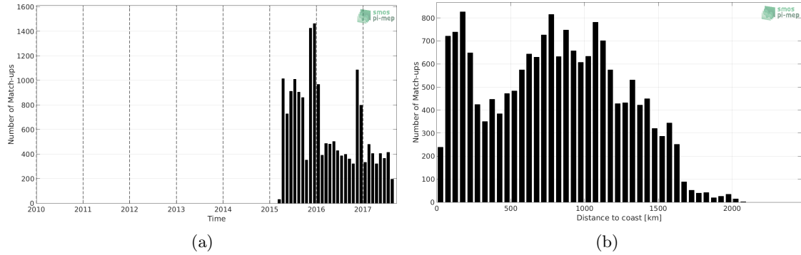
Figure 1: Number of match-ups between Sea mammals and SMAP-L3-RSS-V3-8DAY-RUNNING-40KM SSS as a function of time (a) and as function of the distance to coast (b) over the Global Ocean Pi-MEP region and for the full satellite product period.
