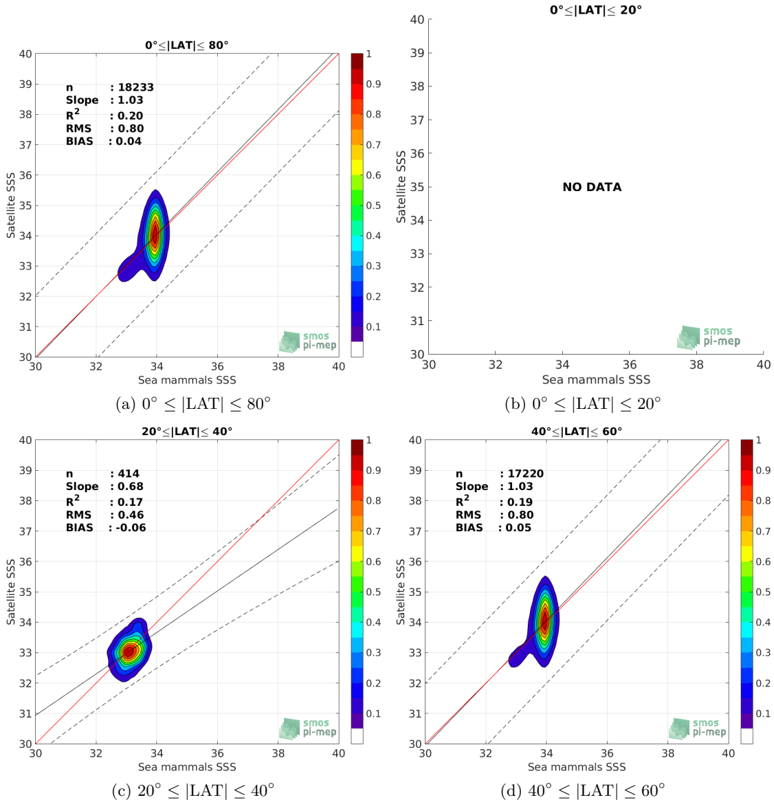
Figure 9: Contour maps of the concentration of SMAP-L3-RSS-V3-8DAY-RUNNING-40KM SSS (y-axis) versus Sea mammals SSS (x-axis) at match-up pairs for different latitudinal bands. For each plot, the red line shows x=y . The black thin and dashed lines indicate a linear fit through the data cloud and the \pm 95\% confidence levels, respectively. The number match-up pairs n , the slope and R^2 coefficient of the linear fit, the root mean square (RMS) and the mean bias between satellite and in situ data are indicated for each latitude band in each plots.
