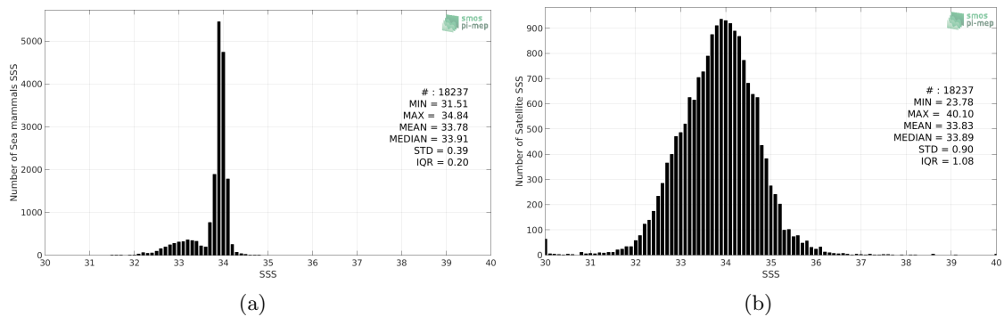
Figure 2: Histograms of SSS from Sea mammals (a) and SMAP-L3-RSS-V3-8DAY-RUNNING-40KM (b) considering all match-up pairs per bins of 0.1 over the Global Ocean Pi-MEP region and for the full satellite product period.
