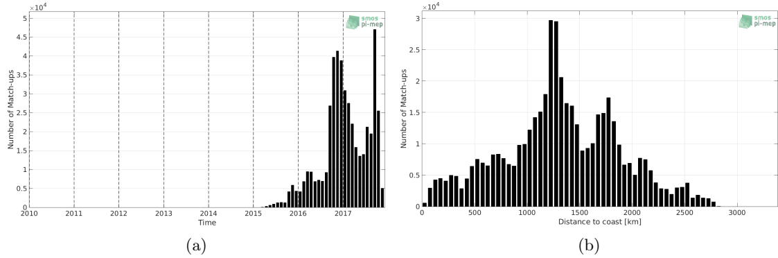
Figure 1: Number of match-ups between Surface drifters and SMAP-L3-RSS-V3-8DAY-RUNNING-40KM SSS as a function of time (a) and as function of the distance to coast (b) over the Global Ocean Pi-MEP region and for the full satellite product period.
