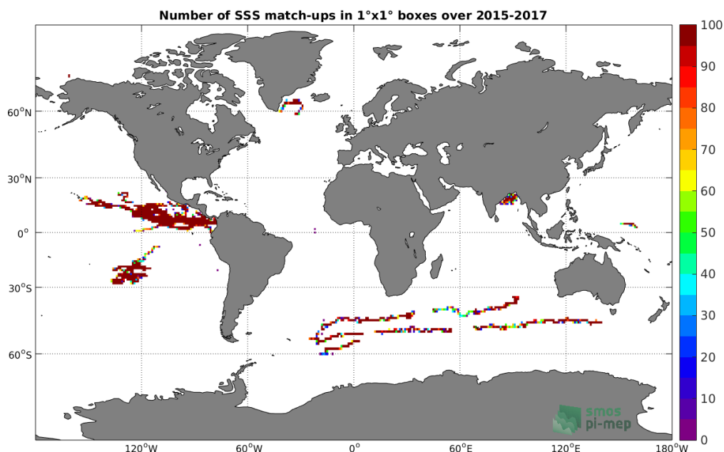
Figure 3: Number of SSS match-ups between Surface drifters SSS and the SMAP-L3-RSS-V3-8DAY-RUNNING-40KM SSS product for the Global Ocean Pi-MEP region over 1°x1° boxes and for the full satellite product period.
