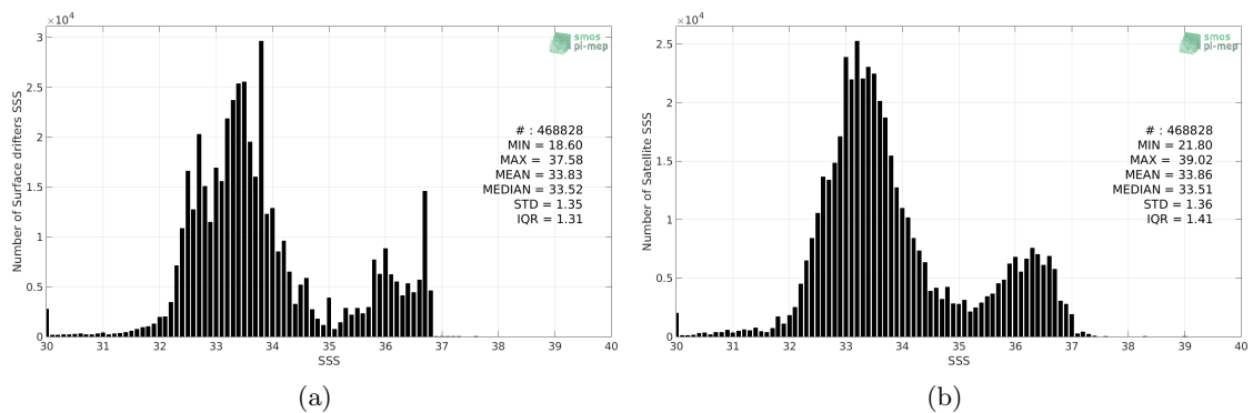
Figure 2: Histograms of SSS from Surface drifters (a) and SMAP-L3-RSS-V3-8DAY-RUNNING-40KM (b) considering all match-up pairs per bins of 0.1 over the Global Ocean Pi-MEP region and for the full satellite product period.
