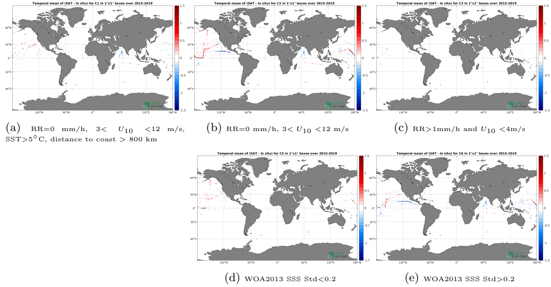
Figure 12: Temporal mean gridded over spatial boxes of size 1^\circ \times 1^\circ of \Delta SSS (SMAP-L3-RSS-V3-MONTHLY-70KM - TSG-SAMOS) for 5 different subdatasets corresponding to: RR=0 mm/h, 3 < U_{10} < 12 m/s, SST > 5^\circ C , distance to coast > 800 km (a), RR=0 mm/h, 3 < U_{10} < 12 m/s (b), RR > 1 mm/h and U_{10} < 4 m/s (c), WOA2013 SSS Std < 0.2 (d), WOA2013 SSS Std > 0.2 (e).
