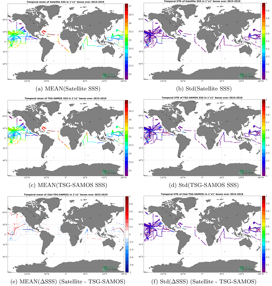
Figure 6: Temporal mean (left) and Std (right) of SSS from SMAP-L3-RSS-V3-MONTHLY-70KM (top), TSG-SAMOS (middle), and of \Delta SSS (Satellite - TSG-SAMOS). Only match-up pairs are used to generate these maps.
