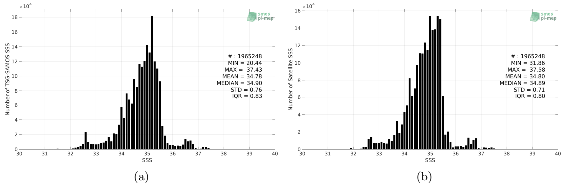
Figure 2: Histograms of SSS from TSG-SAMOS (a) and SMAP-L3-RSS-V3-MONTHLY-70KM (b) considering all match-up pairs per bins of 0.1 over the Global Ocean Pi-MEP region and for the full satellite product period.
