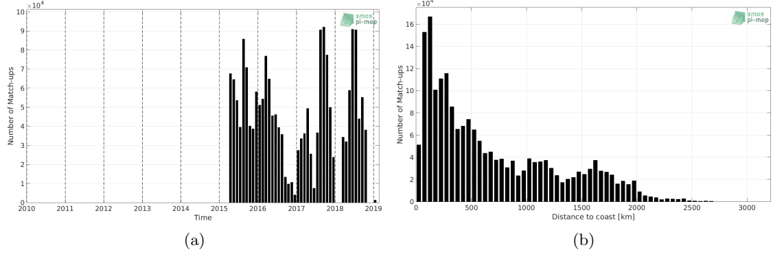
Figure 1: Number of match-ups between TSG-SAMOS and SMAP-L3-RSS-V3-MONTHLY-70KM SSS as a function of time (a) and as function of the distance to coast (b) over the Global Ocean Pi-MEP region and for the full satellite product period.
