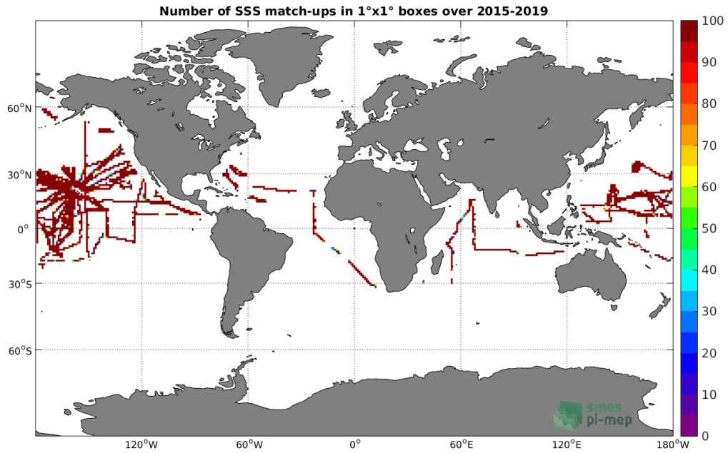
Figure 4: Number of SSS match-ups between TSG-SAMOS SSS and the SMAP-L3-RSS-V3-MONTHLY-70KM SSS product for the Global Ocean Pi-MEP region over 1°x1° boxes and for the full satellite product period.
