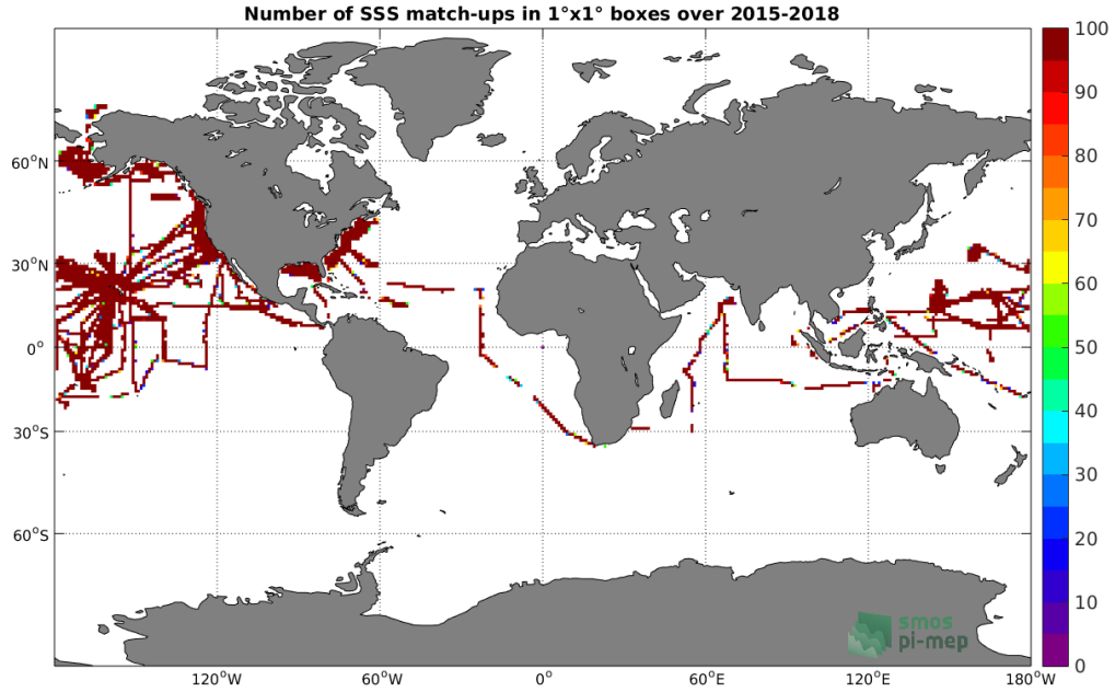
Figure 4: Number of SSS match-ups between TSG-SAMOS SSS and the SMAP-L3-RSS-V3-MONTHLY-70KM SSS product for the Global Ocean Pi-MEP region over 1^\circ \times 1^\circ boxes and for the full satellite product period.
