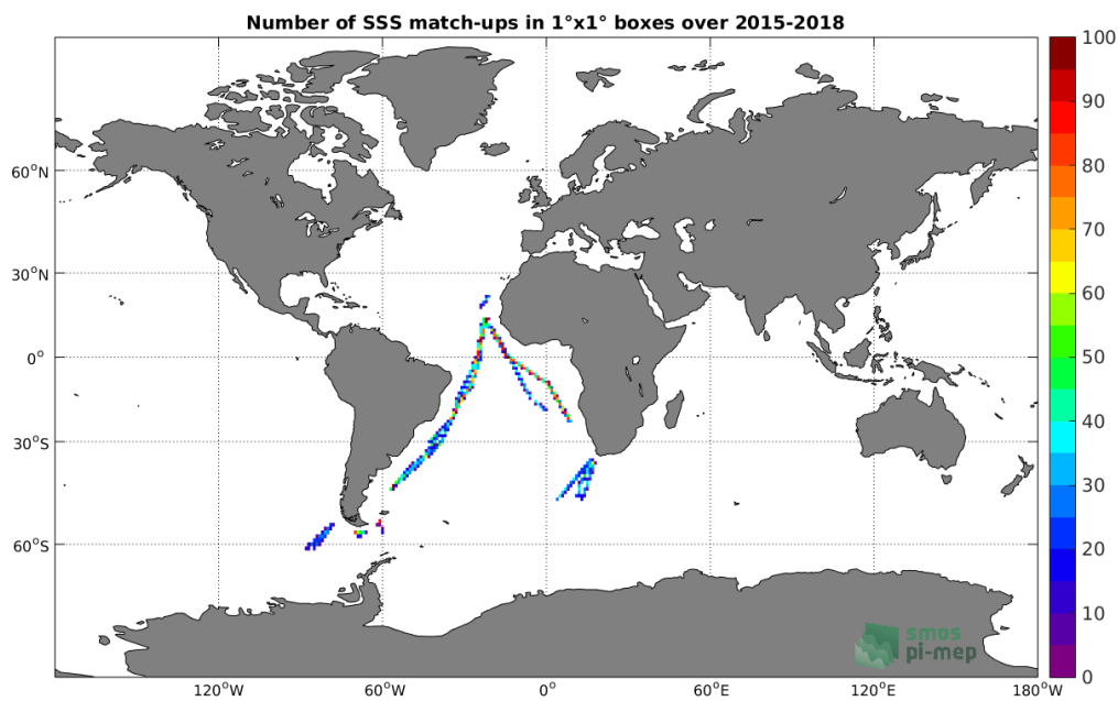
Figure 4: Number of SSS match-ups between TSG-POLARSTERN SSS and the SMAP-L3-RSS-V3-MONTHLY-70KM SSS product for the Global Ocean Pi-MEP region over 1^\circ \times 1^\circ boxes and for the full satellite product period.
