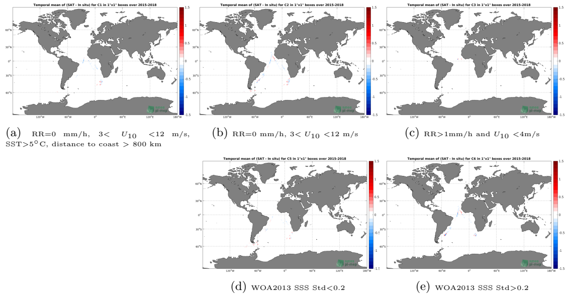
Figure 12: Temporal mean gridded over spatial boxes of size 1^\circ \times 1^\circ of \Delta SSS (SMAP-L3-RSS-V3-MONTHLY-70KM - TSG-POLARSTERN) for 5 different subdatasets corresponding to:RR=0 mm/h, 3 < U_{10} < 12 m/s, SST >5^\circ C, distance to coast > 800 km (a), RR=0 mm/h, 3 < U_{10} < 12 m/s (b), RR >1 mm/h and U_{10} < 4 m/s (c), WOA2013 SSS Std <0.2 (d), WOA2013 SSS Std >0.2 (e).
