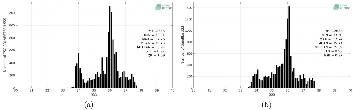
Figure 2: Histograms of SSS from TSG-POLARSTERN (a) and SMAP-L3-RSS-V3-MONTHLY-70KM (b) considering all match-up pairs per bins of 0.1 over the Global Ocean Pi-MEP region and for the full satellite product period.
