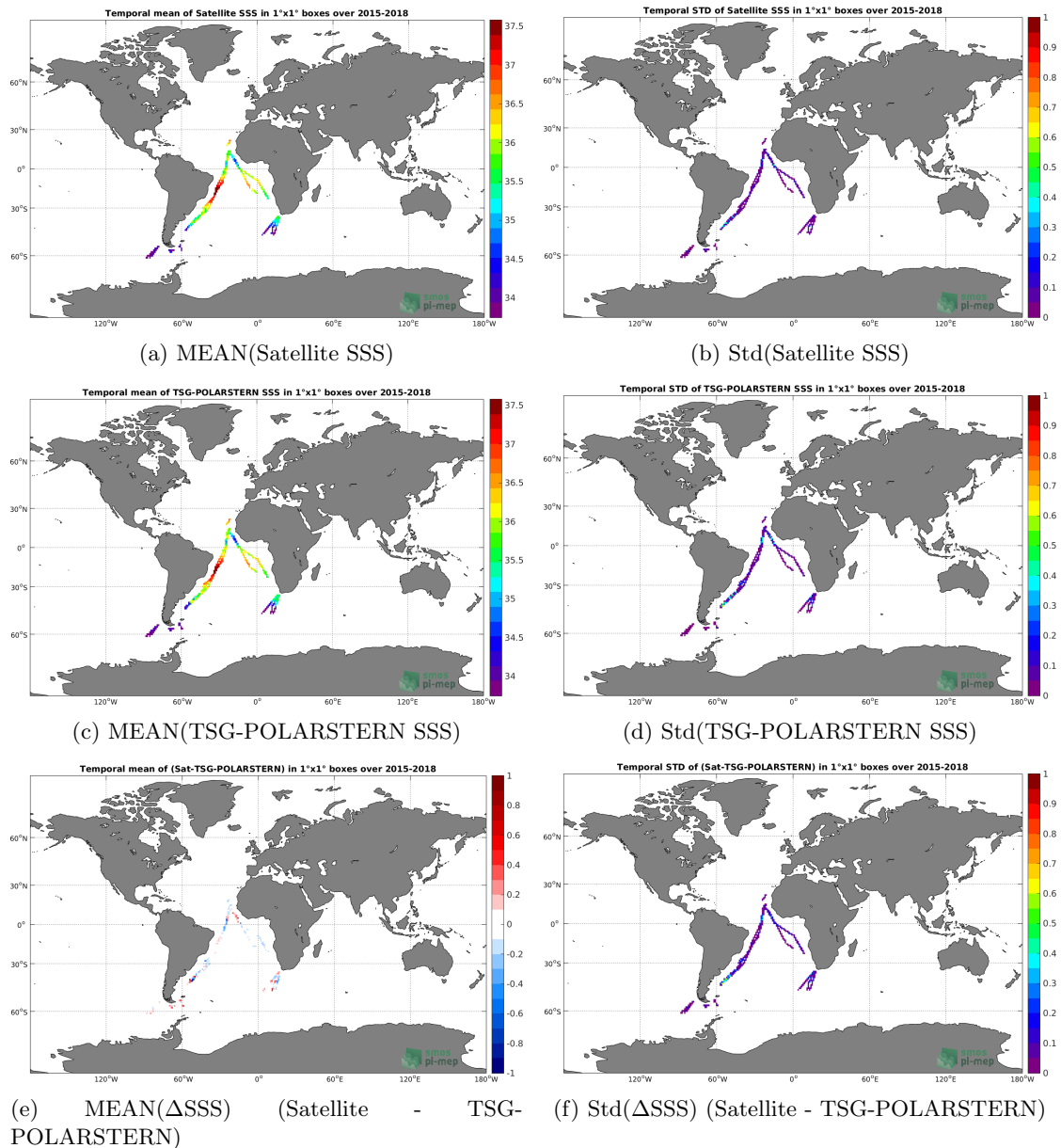
Figure 6: Temporal mean (left) and Std (right) of SSS from SMAP-L3-RSS-V3-MONTHLY-70KM (top), TSG-POLARSTERN (middle), and of \Delta SSS (Satellite - TSG-POLARSTERN). Only match-up pairs are used to generate these maps.
