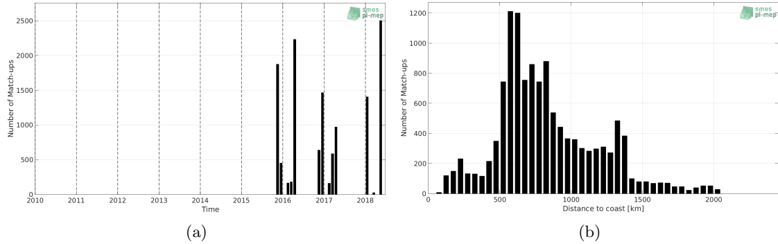
Figure 1: Number of match-ups between TSG-POLARSTERN and SMAP-L3-RSS-V3-MONTHLY-70KM SSS as a function of time (a) and as function of the distance to coast (b) over the Global Ocean Pi-MEP region and for the full satellite product period.
