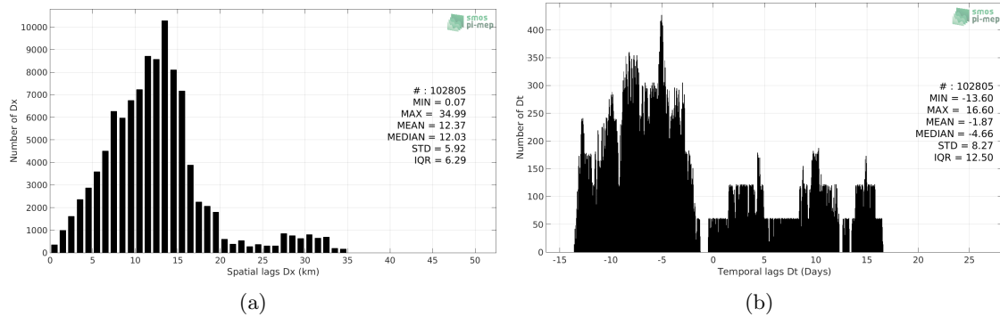
Figure 5: Histograms of the spatial (a) and temporal (b) lags between the time of the TSG-NCEI-0170743 measurements and the date of the corresponding SMAP-L3-RSS-V3-MONTHLY-70KM SSS product.
