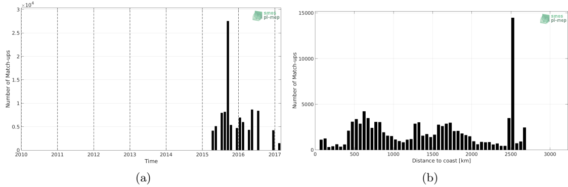
Figure 1: Number of match-ups between TSG-NCEI-0170743 and SMAP-L3-RSS-V3-MONTHLY-70KM SSS as a function of time (a) and as function of the distance to coast (b) over the Global Ocean Pi-MEP region and for the full satellite product period.
