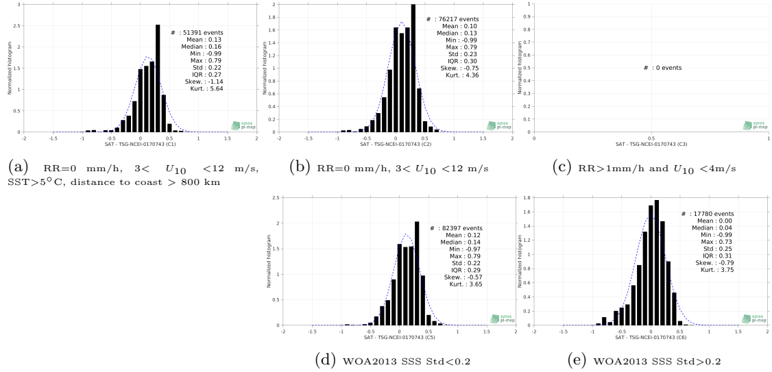
Figure 13: Normalized histogram of \Delta SSS (SMAP-L3-RSS-V3-MONTHLY-70KM - TSG-NCEI-0170743) for 5 different subdatasets corresponding to: RR=0 mm/h, 3 < U_{10} < 12 m/s, SST>5°C, distance to coast > 800 km (a), RR=0 mm/h, 3 < U_{10} < 12 m/s (b), RR>1mm/h and U_{10} < 4 m/s (c), WOA2013 SSS Std<0.2 (d), WOA2013 SSS Std>0.2 (e).
