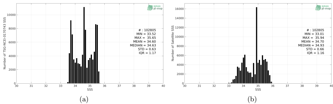
Figure 2: Histograms of SSS from TSG-NCEI-0170743 (a) and SMAP-L3-RSS-V3-MONTHLY-70KM (b) considering all match-up pairs per bins of 0.1 over the Global Ocean Pi-MEP region and for the full satellite product period.
