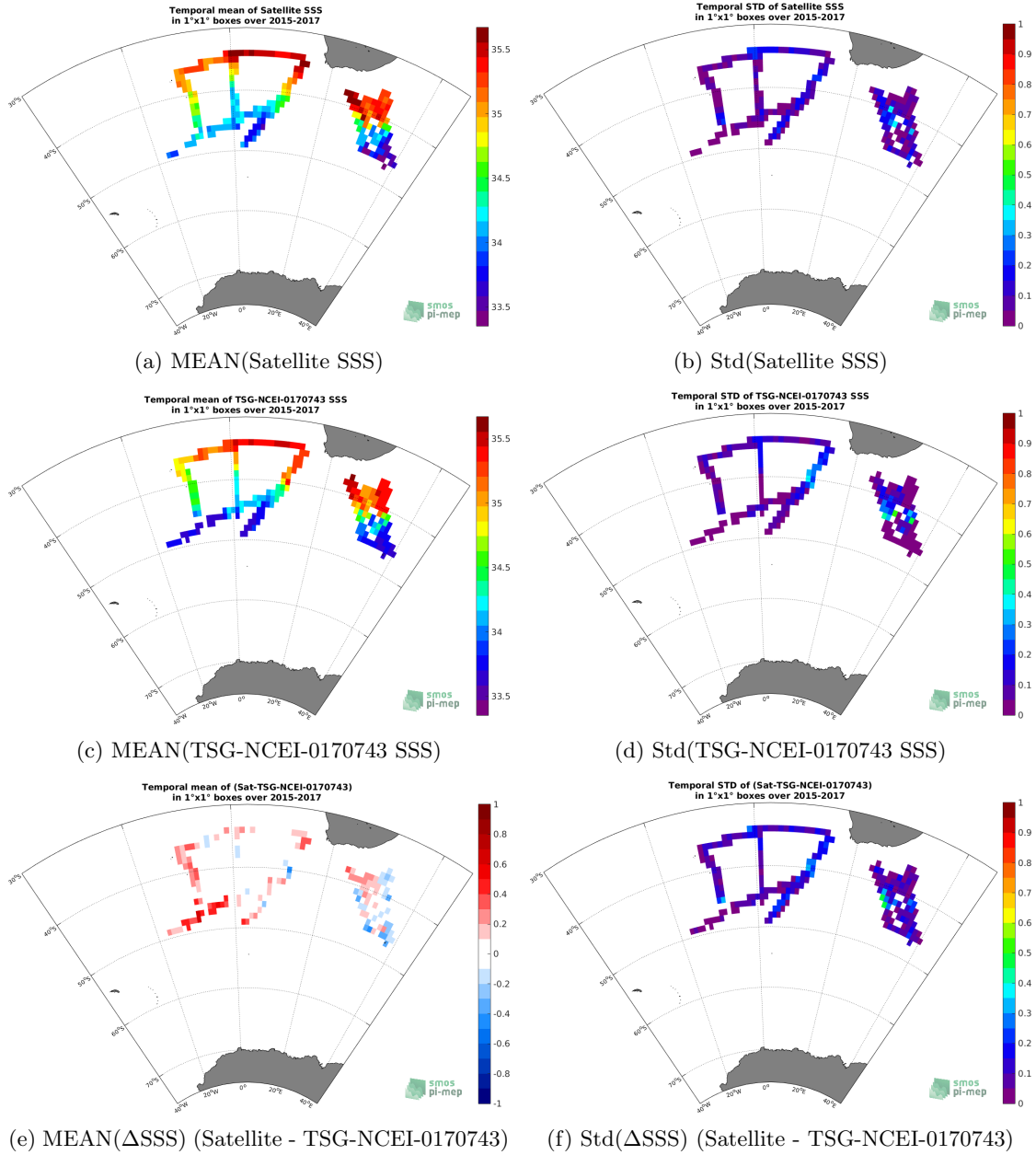
Figure 6: Temporal mean (left) and Std (right) of SSS from SMAP-L3-RSS-V3-MONTHLY-70KM (top), TSG-NCEI-0170743 (middle), and of \Delta SSS (Satellite - TSG-NCEI-0170743). Only match-up pairs are used to generate these maps.
