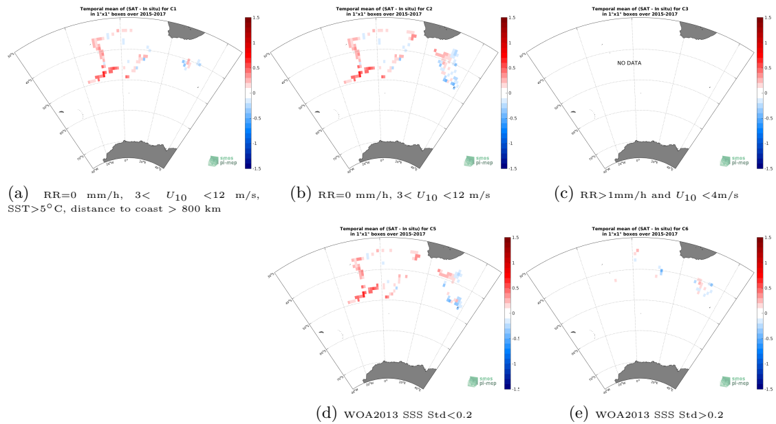
Figure 12: Temporal mean gridded over spatial boxes of size 1^\circ \times 1^\circ of \Delta SSS (SMAP-L3-RSS-V3-MONTHLY-70KM - TSG-NCEI-0170743) for 5 different subdatasets corresponding to:RR=0 mm/h, 3 < U_{10} < 12 m/s, SST >5^\circ\text{C} , distance to coast > 800 km (a), RR=0 mm/h, 3 < U_{10} < 12 m/s (b), RR >1 mm/h and U_{10} < 4 m/s (c), WOA2013 SSS Std <0.2 (d), WOA2013 SSS Std >0.2 (e).
