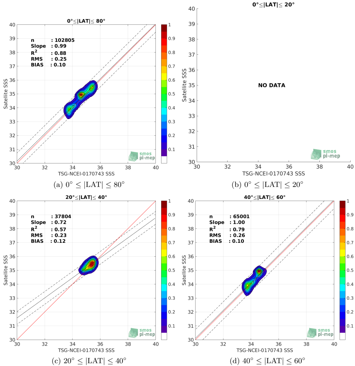
Figure 9: Contour maps of the concentration of SMAP-L3-RSS-V3-MONTHLY-70KM SSS (y-axis) versus TSG-NCEI-0170743 SSS (x-axis) at match-up pairs for different latitude bands. For each plot, the red line shows x=y . The black thin and dashed lines indicate a linear fit through the data cloud and the \pm 95\% confidence levels, respectively. The number match-up pairs n , the slope and R^2 coefficient of the linear fit, the root mean square (RMS) and the mean bias between satellite and in situ data are indicated for each latitude band in each plots.
