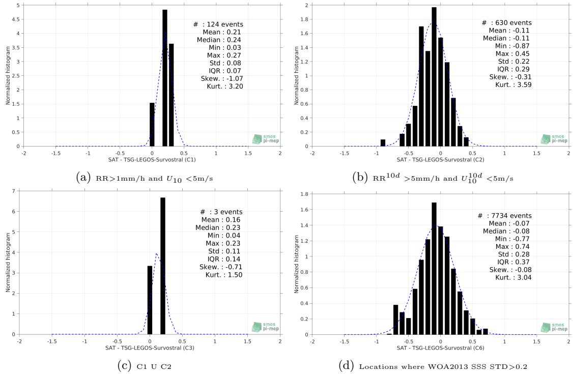
Figure 13: Normalized histogram of \Delta SSS (SMAP-L3-RSS-V3-MONTHLY-70KM - TSG-LEGOS-Survostral) for 6 different subdatasets corresponding to: RR > 1mm/h and U_{10} < 5 m/s (a), RR^{10d} > 5 mm/h and U_{10}^{10d} < 5 m/s (b), C1 U C2 (c), Locations where WOA2013 SSS STD > 0.2 (d).
