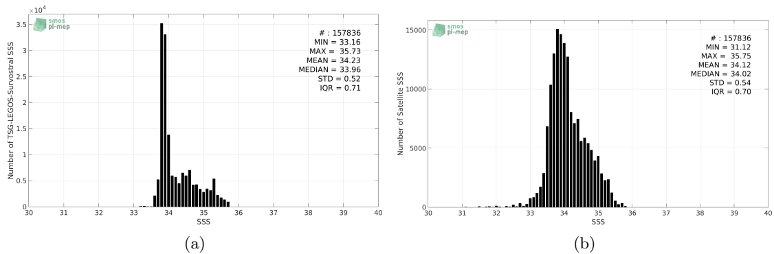
Figure 2: Histograms of SSS from TSG-LEGOS-Survostral (a) and SMAP-L3-RSS-V3-MONTHLY-70KM (b) considering all match-up pairs per bins of 0.1 over the Global Ocean Pi-MEP region and for the full satellite product period.
