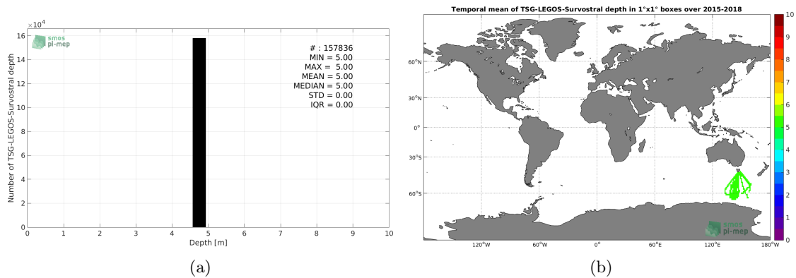
Figure 3: Histograms of the depth of the upper level SSS measurements from TSG-LEGOS-Survostral in the Match-up DataBase for the Global Ocean Pi-MEP region (a) and temporal mean spatial distribution of pressure of the in situ SSS data over 1^\circ \times 1^\circ boxes and for the full satellite product period (b).
