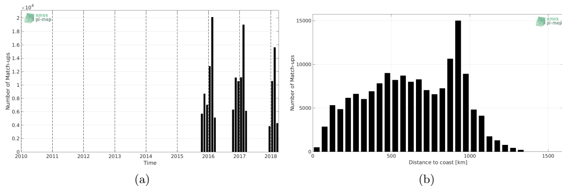
Figure 1: Number of match-ups between TSG-LEGOS-Survostral and SMAP-L3-RSS-V3-MONTHLY-70KM SSS as a function of time (a) and as function of the distance to coast (b) over the Global Ocean Pi-MEP region and for the full satellite product period.
