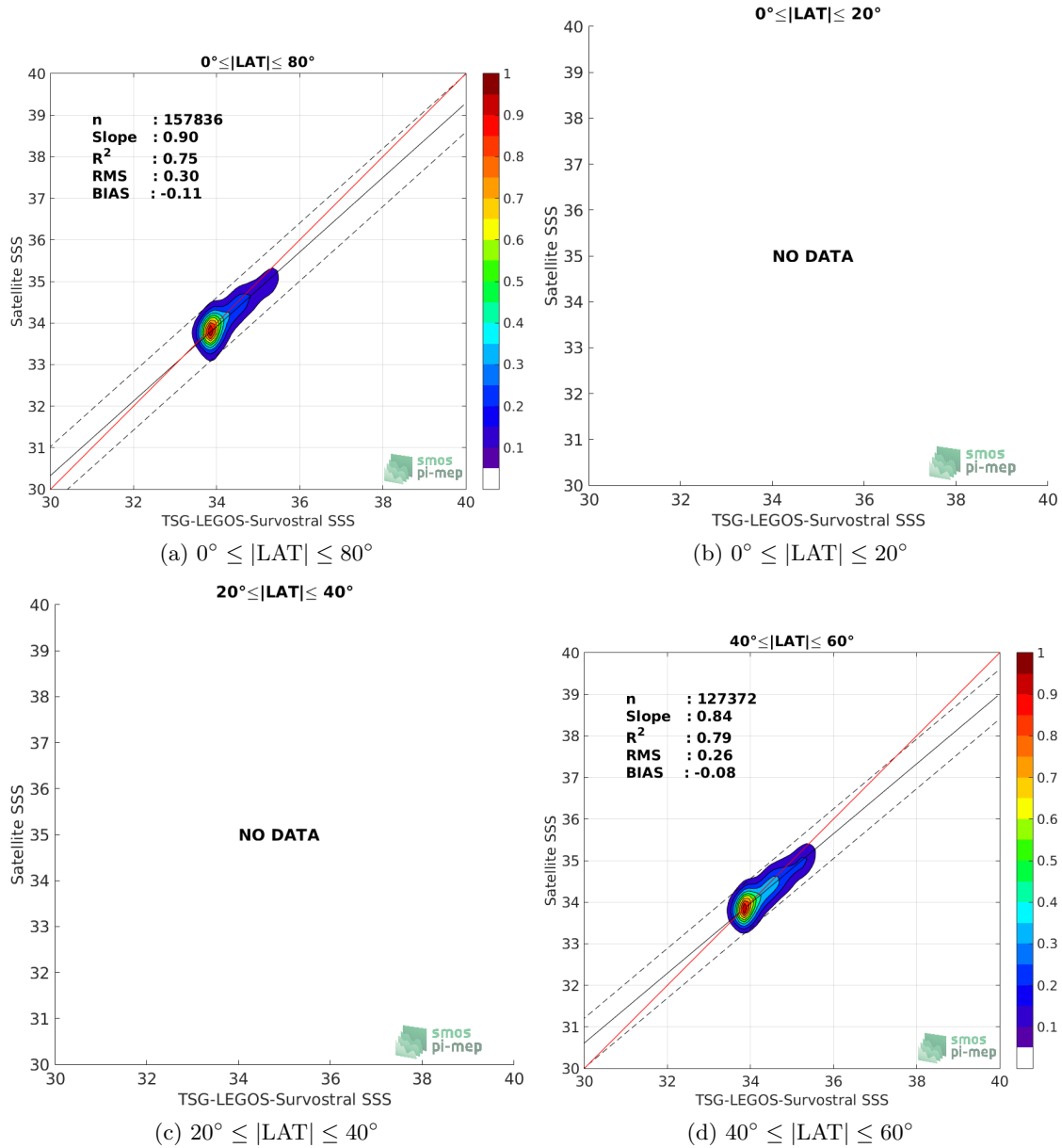
Figure 9: Contour maps of the concentration of SMAP-L3-RSS-V3-MONTHLY-70KM SSS (y-axis) versus TSG-LEGOS-Survostral SSS (x-axis) at match-up pairs for different latitude bands. For each plot, the red line shows x=y . The black thin and dashed lines indicate a linear fit through the data cloud and the \pm 95\% confidence levels, respectively. The number match-up pairs n , the slope and R^2 coefficient of the linear fit, the root mean square (RMS) and the mean bias between satellite and in situ data are indicated for each latitude band in each plots.
