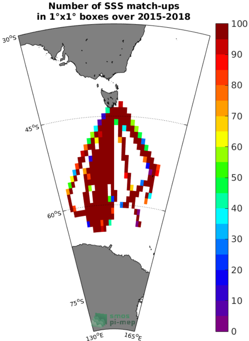
Figure 4: Number of SSS match-ups between TSG-LEGOS-Survostral SSS and the SMAP-L3-RSS-V3-MONTHLY-70KM SSS product for the Global Ocean Pi-MEP region over 1°x1° boxes and for the full satellite product period.
