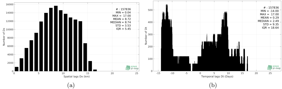
Figure 5: Histograms of the spatial (a) and temporal (b) lags between the time of the TSG-LEGOS-Survostral measurements and the date of the corresponding SMAP-L3-RSS-V3-MONTHLY-70KM SSS product.
