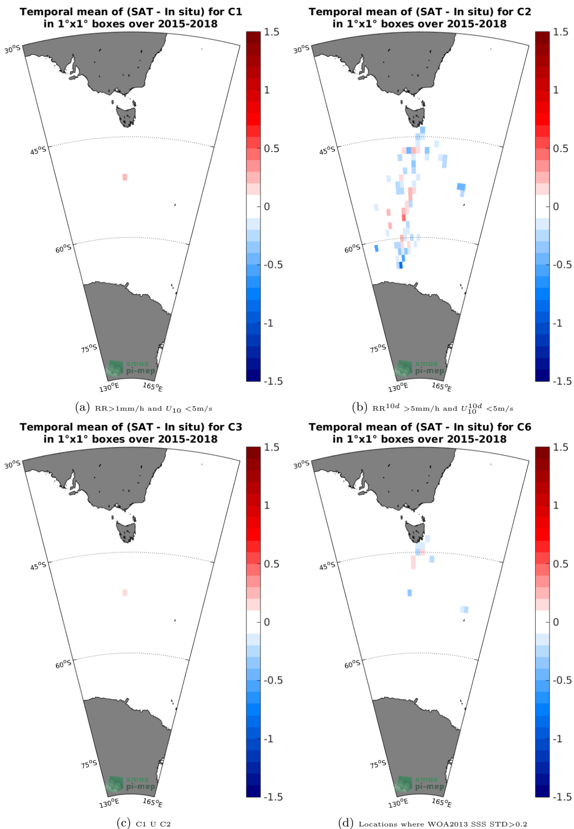
Figure 12: Temporal mean gridded over spatial boxes of size 1°x1° of \Delta\text{SSS} (SMAP-L3-RSS-V3-MONTHLY-70KM - TSG-LEGOS-Survostral) for 4 different subdatasets corresponding to: RR > 1\text{mm/h} and U_{10} < 5\text{m/s} (a), RR^{10d} > 5\text{mm/h} and U_{10}^{10d} < 5\text{m/s} (b), C1 U C2 (c), Locations where WOA2013 SSS STD > 0.2 (d).
