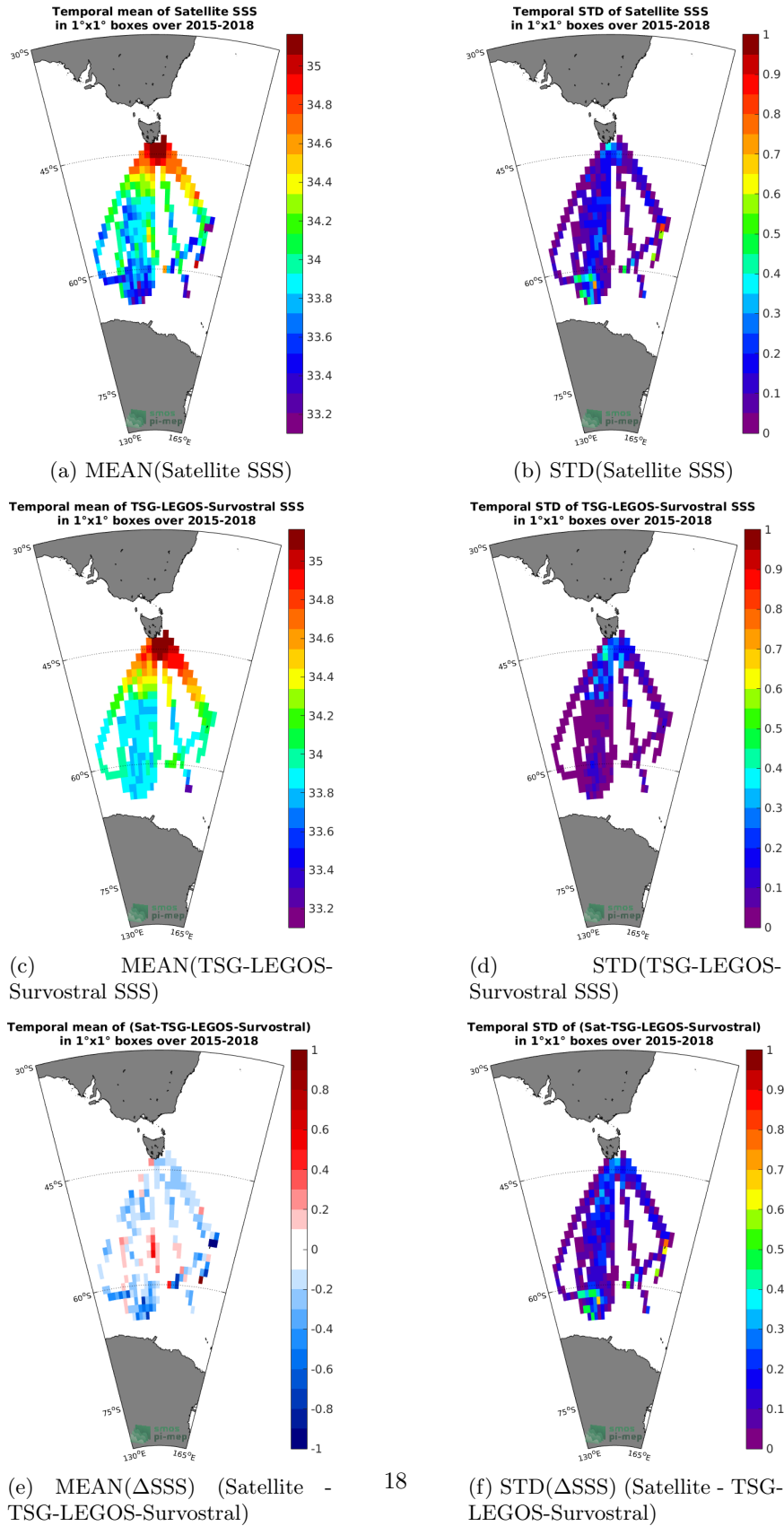
Figure 6: Temporal mean (left) and STD (right) of SSS from SMAP-L3-RSS-V3-MONTHLY-70KM (top), TSG-LEGOS-Survostral (middle), and of \Delta SSS (Satellite - TSG-LEGOS-Survostral). Only match-up pairs are used to generate these maps.
