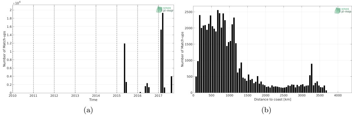
Figure 1: Number of match-ups between TSG-GOSUD-Sailing-ship and SMAP-L3-RSS-V3-MONTHLY-70KM SSS as a function of time (a) and as function of the distance to coast (b) over the Global Ocean Pi-MEP region and for the full satellite product period.
