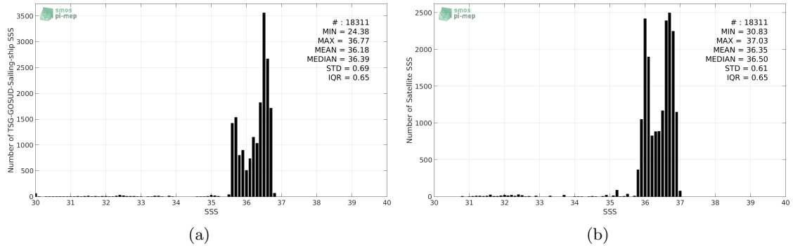
Figure 2: Histograms of SSS from TSG-GOSUD-Sailing-ship (a) and SMAP-L3-RSS-V3-MONTHLY-70KM (b) considering all match-up pairs per bins of 0.1 over the Global Ocean Pi-MEP region and for the full satellite product period.
