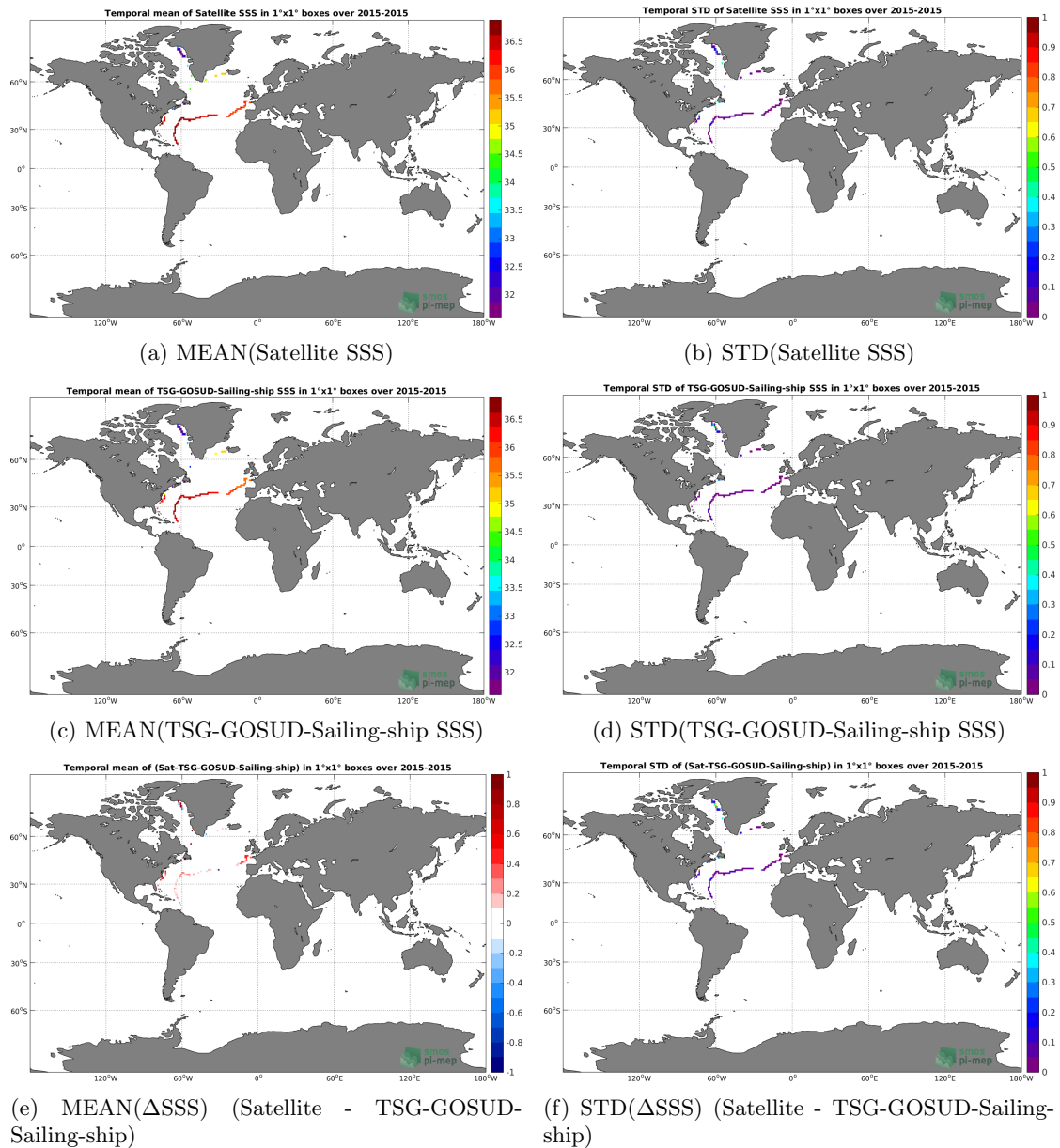
Figure 6: Temporal mean (left) and STD (right) of SSS from SMAP-L3-RSS-V3-MONTHLY-70KM (top), TSG-GOSUD-Sailing-ship (middle), and of \Delta SSS (Satellite - TSG-GOSUD-Sailing-ship). Only match-up pairs are used to generate these maps.
