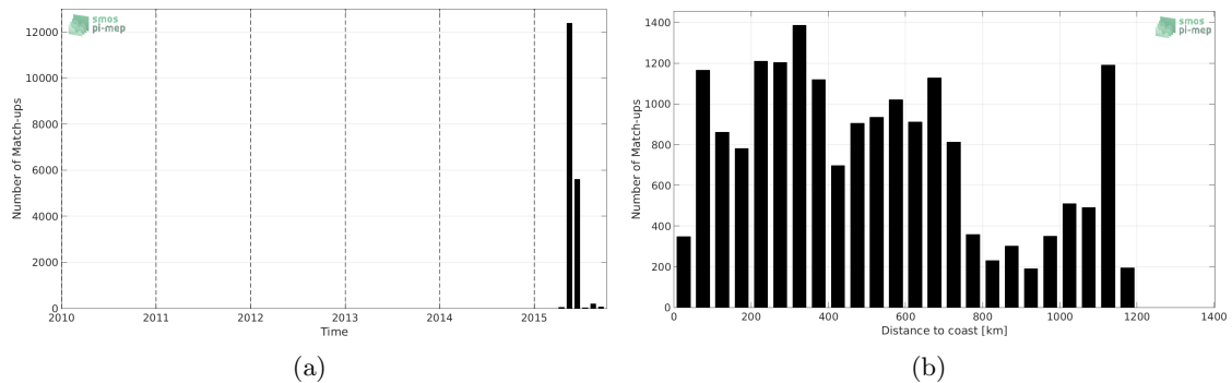
Figure 1: Number of match-ups between TSG-GOSUD-Sailing-ship and SMAP-L3-RSS-V3-MONTHLY-70KM SSS as a function of time (a) and as function of the distance to coast (b) over the Global Ocean Pi-MEP region and for the full satellite product period.
