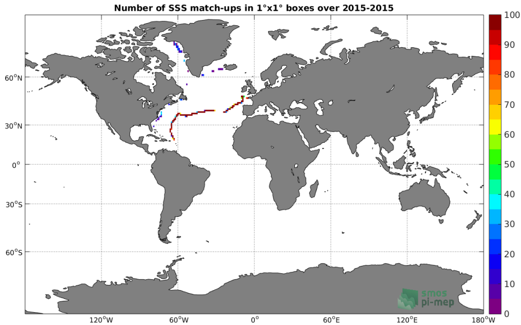
Figure 4: Number of SSS match-ups between TSG-GOSUD-Sailing-ship SSS and the SMAP-L3-RSS-V3-MONTHLY-70KM SSS product for the Global Ocean Pi-MEP region over 1°x1° boxes and for the full satellite product period.
