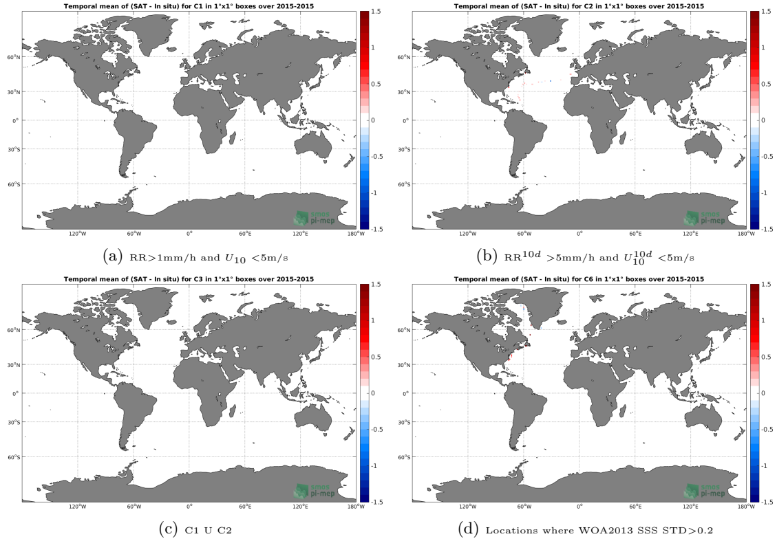
Figure 12: Temporal mean gridded over spatial boxes of size 1^\circ \times 1^\circ of \Delta SSS (SMAP-L3-RSS-V3-MONTHLY-70KM - TSG-GOSUD-Sailing-ship) for 4 different subdatasets corresponding to: RR > 1\text{mm/h} and U_{10} < 5\text{m/s} (a), RR^{10d} > 5\text{mm/h} and U_{10}^{10d} < 5\text{m/s} (b), C1 U C2 (c), Locations where WOA2013 SSS STD > 0.2 (d).
