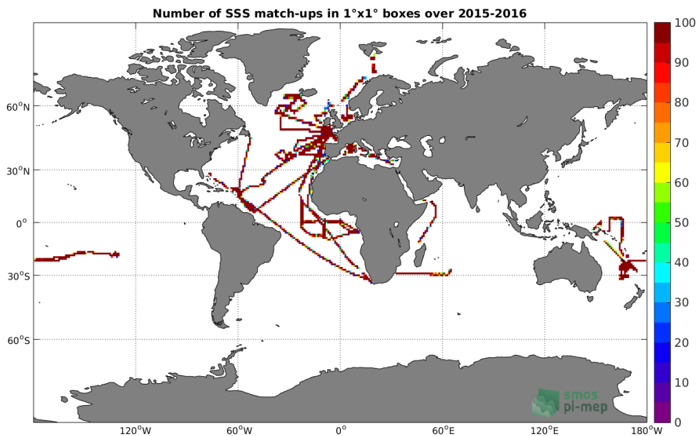
Figure 4: Number of SSS match-ups between TSG-GOSUD-Research-vessel SSS and the SMAP-L3-RSS-V3-MONTHLY-70KM SSS product for the Global Ocean Pi-MEP region over 1°x1° boxes and for the full satellite product period.
