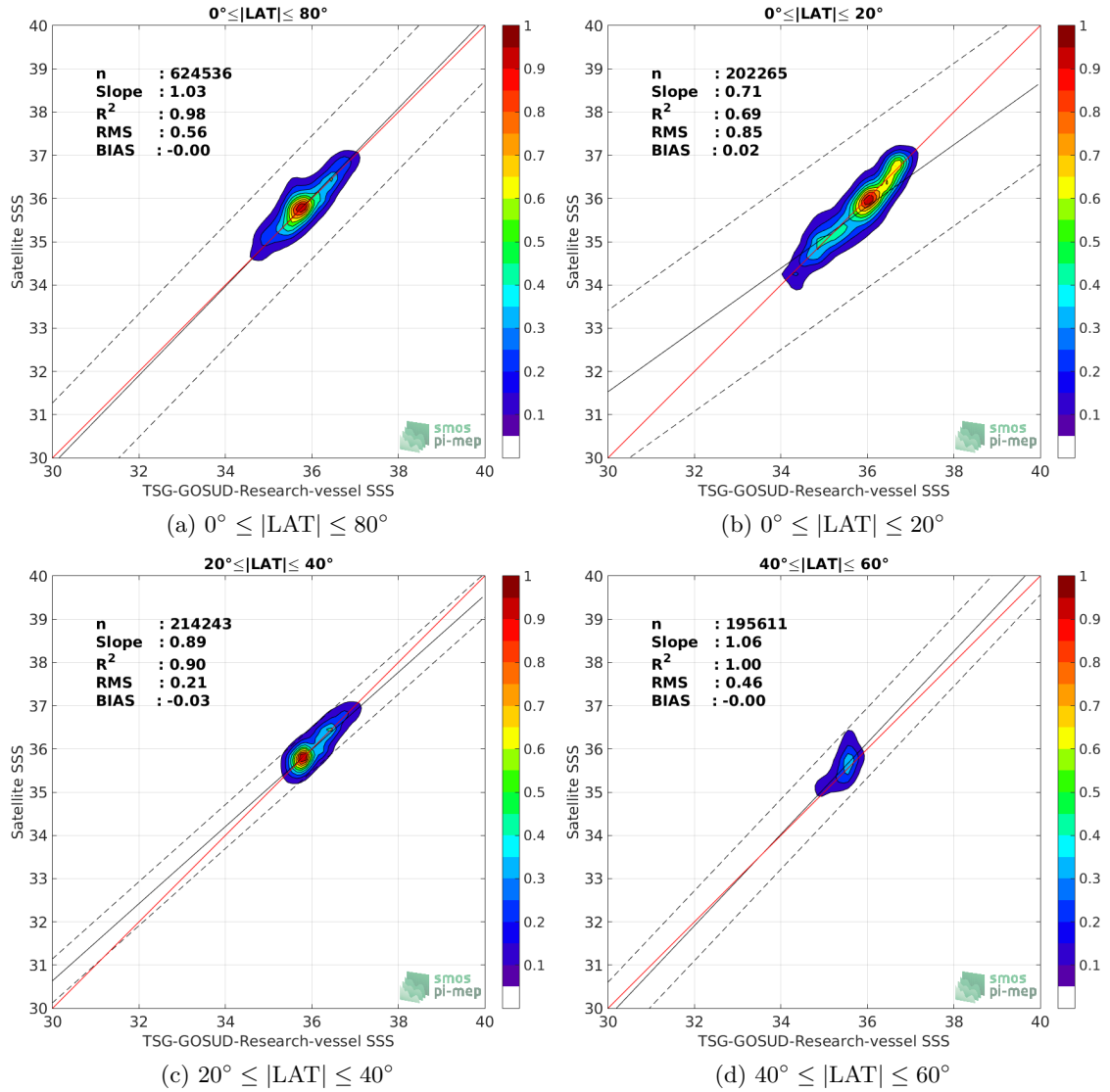
Figure 9: Contour maps of the concentration of SMAP-L3-RSS-V3-MONTHLY-70KM SSS (y-axis) versus TSG-GOSUD-Research-vessel SSS (x-axis) at match-up pairs for different latitudinal bands. For each plot, the red line shows x=y . The black thin and dashed lines indicate a linear fit through the data cloud and the \pm 95\% confidence levels, respectively. The number match-up pairs n , the slope and R^2 coefficient of the linear fit, the root mean square (RMS) and the mean bias between satellite and in situ data are indicated for each latitude band in each plots.
