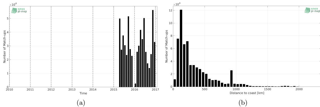
Figure 1: Number of match-ups between TSG-GOSUD-Research-vessel and SMAP-L3-RSS-V3-MONTHLY-70KM SSS as a function of time (a) and as function of the distance to coast (b) over the Global Ocean Pi-MEP region and for the full satellite product period.
