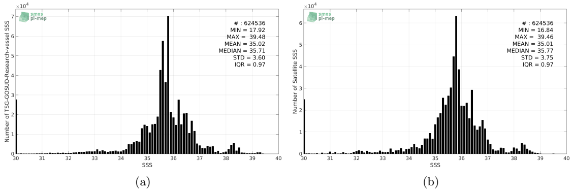
Figure 2: Histograms of SSS from TSG-GOSUD-Research-vessel (a) and SMAP-L3-RSS-V3-MONTHLY-70KM (b) considering all match-up pairs per bins of 0.1 over the Global Ocean Pi-MEP region and for the full satellite product period.
