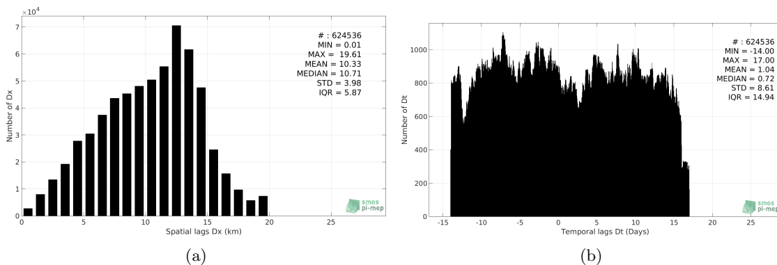
Figure 5: Histograms of the spatial (a) and temporal (b) lags between the time of the TSG-GOSUD-Research-vessel measurements and the date of the corresponding SMAP-L3-RSS-V3-MONTHLY-70KM SSS product.
