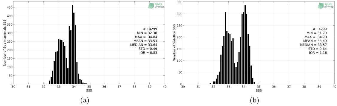
Figure 2: Histograms of SSS from Sea mammals (a) and SMAP-L3-RSS-V3-MONTHLY-70KM (b) considering all match-up pairs per bins of 0.1 over the Global Ocean Pi-MEP region and for the full satellite product period.
