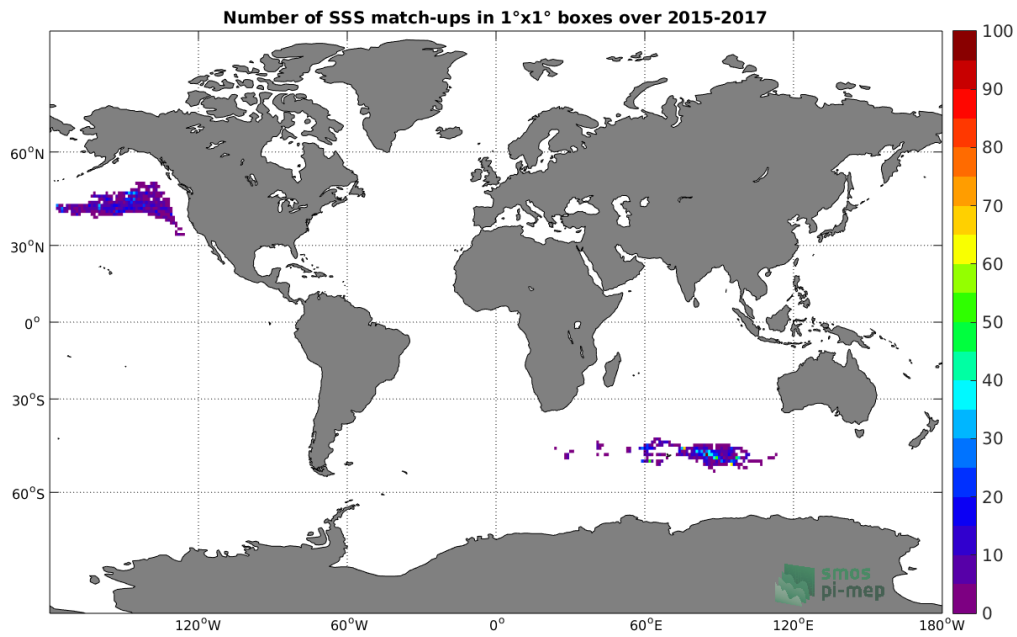
Figure 4: Number of SSS match-ups between Sea mammals SSS and the SMAP-L3-RSS-V3-MONTHLY-70KM SSS product for the Global Ocean Pi-MEP region over 1^\circ \times 1^\circ boxes and for the full satellite product period.
