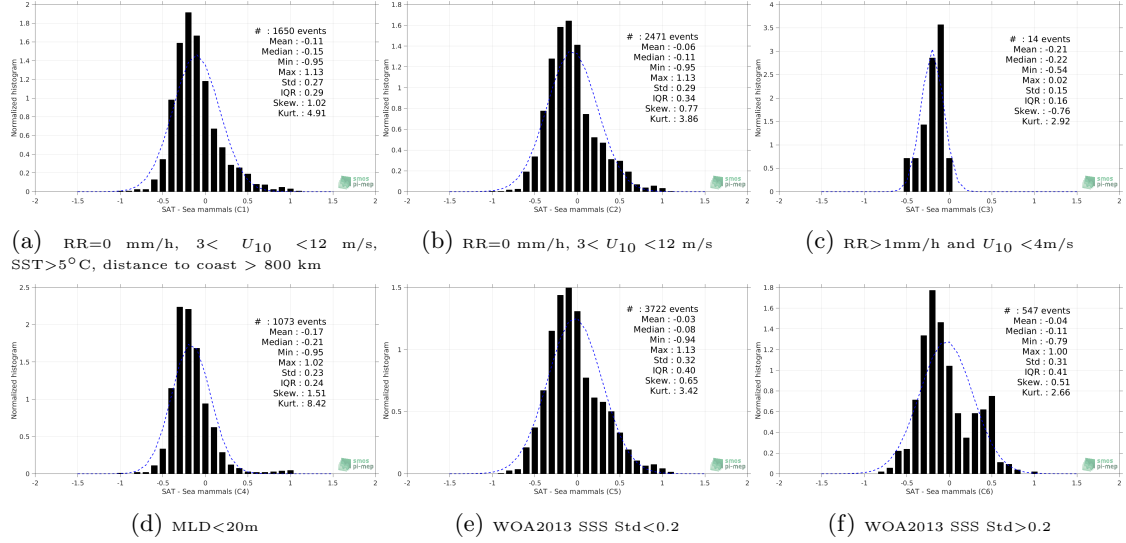
Figure 13: Normalized histogram of \Delta SSS (SMAP-L3-RSS-V3-MONTHLY-70KM - Sea mammals) for 6 different subdatasets corresponding to: RR=0 mm/h, 3 < U_{10} < 12 m/s, SST>5°C, distance to coast > 800 km (a), RR=0 mm/h, 3 < U_{10} < 12 m/s (b), RR>1mm/h and U_{10} < 4 m/s (c), MLD<20m (d), WOA2013 SSS Std<0.2 (e), WOA2013 SSS Std>0.2 (f).
