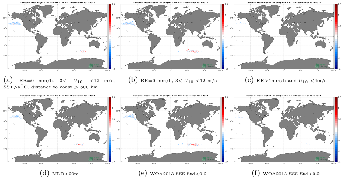
Figure 12: Temporal mean gridded over spatial boxes of size 1^\circ \times 1^\circ of \Delta SSS (SMAP-L3-RSS-V3-MONTHLY-70KM - Sea mammals) for 6 different subdatasets corresponding to: RR=0 mm/h, 3 < U_{10} < 12 m/s, SST > 5^\circ C , distance to coast > 800 km (a), RR=0 mm/h, 3 < U_{10} < 12 m/s (b), RR > 1 mm/h and U_{10} < 4 m/s (c), MLD < 20 m (d), WOA2013 SSS Std < 0.2 (e), WOA2013 SSS Std > 0.2 (f).
