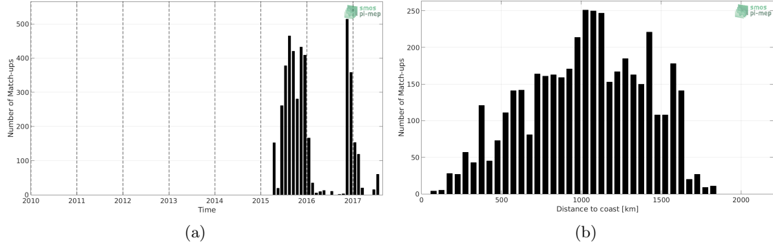
Figure 1: Number of match-ups between Sea mammals and SMAP-L3-RSS-V3-MONTHLY-70KM SSS as a function of time (a) and as function of the distance to coast (b) over the Global Ocean Pi-MEP region and for the full satellite product period.
