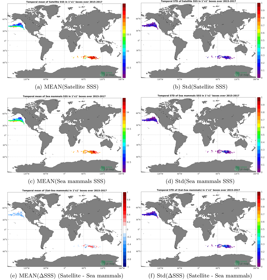
Figure 6: Temporal mean (left) and Std (right) of SSS from SMAP-L3-RSS-V3-MONTHLY-70KM (top), Sea mammals (middle), and of \Delta SSS (Satellite - Sea mammals). Only match-up pairs are used to generate these maps.
