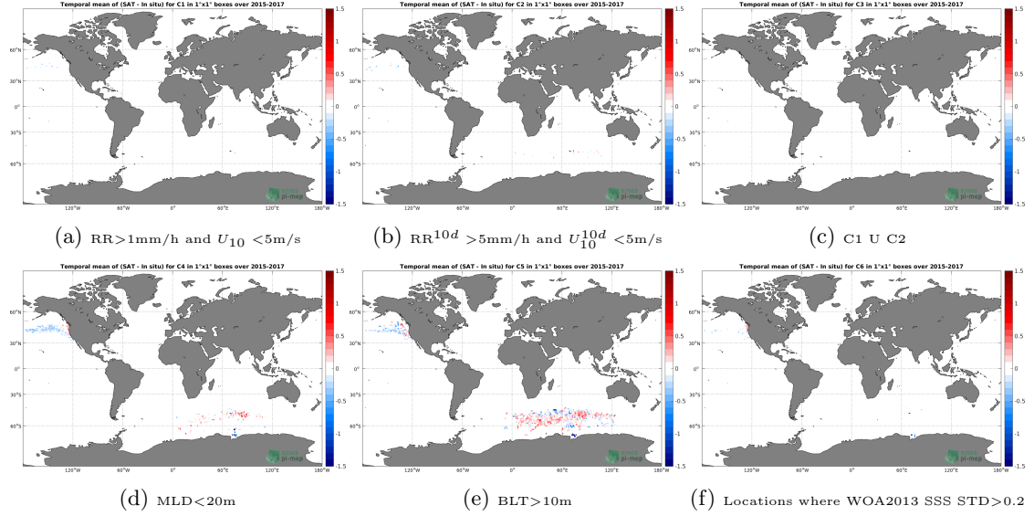
Figure 12: Temporal mean gridded over spatial boxes of size 1^\circ \times 1^\circ of \Delta\text{SSS} (SMAP-L3-RSS-V3-MONTHLY-70KM - Sea mammals) for 6 different subdatasets corresponding to: RR > 1\text{mm/h} and U_{10} < 5\text{m/s} (a), RR^{10d} > 5\text{mm/h} and U_{10}^{10d} < 5\text{m/s} (b), C1 U C2 (c), MLD < 20\text{m} (d), BLT > 10\text{m} (e), Locations where WOA2013 SSS STD > 0.2 (f).
