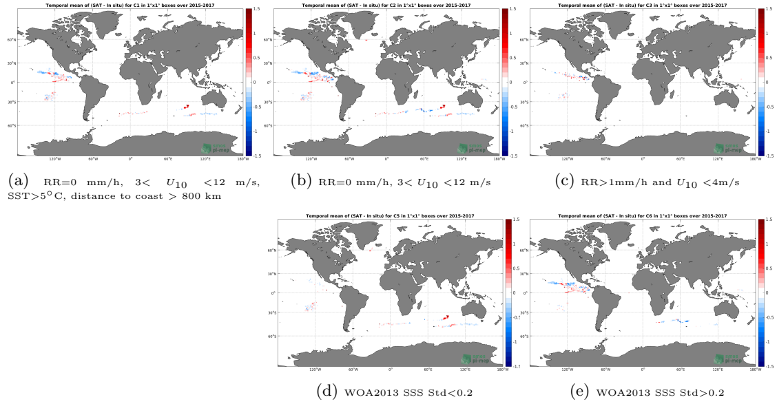
Figure 11: Temporal mean gridded over spatial boxes of size 1^\circ \times 1^\circ of \Delta SSS (SMAP-L3-RSS-V3-MONTHLY-70KM - Surface drifters) for 5 different subdatasets corresponding to:RR=0 mm/h, 3 < U_{10} < 12 m/s, SST >5^\circ\text{C} , distance to coast > 800 km (a), RR=0 mm/h, 3 < U_{10} < 12 m/s (b), RR >1 mm/h and U_{10} < 4 m/s (c), WOA2013 SSS Std <0.2 (d), WOA2013 SSS Std >0.2 (e).
