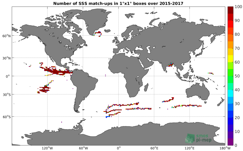
Figure 3: Number of SSS match-ups between Surface drifters SSS and the SMAP-L3-RSS-V3-MONTHLY-70KM SSS product for the Global Ocean Pi-MEP region over 1°x1° boxes and for the full satellite product period.
