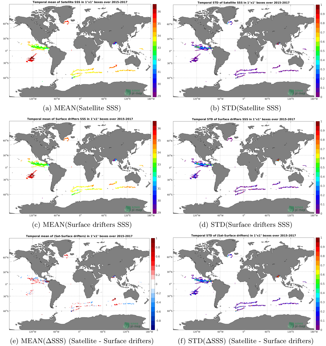
Figure 5: Temporal mean (left) and STD (right) of SSS from SMAP-L3-RSS-V3-MONTHLY-70KM (top), Surface drifters (middle), and of \Delta SSS (Satellite - Surface drifters). Only match-up pairs are used to generate these maps.
