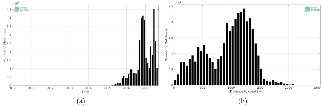
Figure 1: Number of match-ups between Surface drifters and SMAP-L3-RSS-V3-MONTHLY-70KM SSS as a function of time (a) and as function of the distance to coast (b) over the Global Ocean Pi-MEP region and for the full satellite product period.
