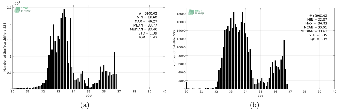
Figure 2: Histograms of SSS from Surface drifters (a) and SMAP-L3-RSS-V3-MONTHLY-70KM (b) considering all match-up pairs per bins of 0.1 over the Global Ocean Pi-MEP region and for the full satellite product period.
