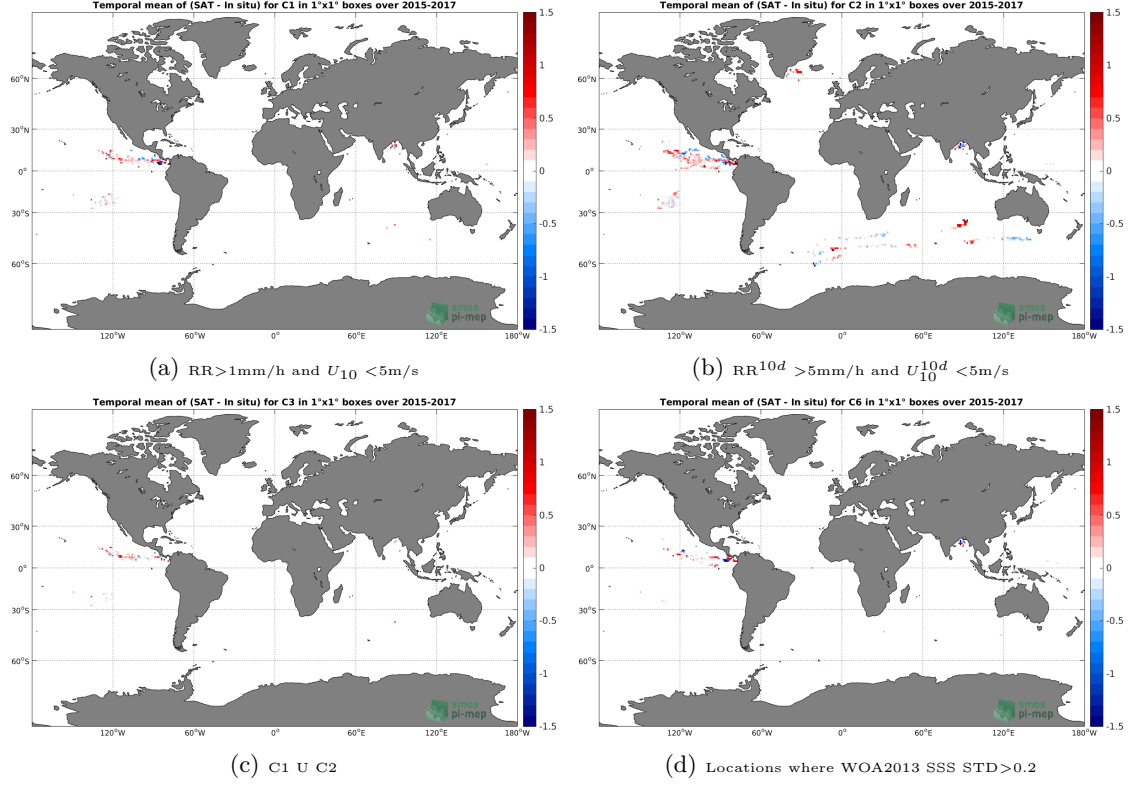
Figure 11: Temporal mean gridded over spatial boxes of size 1^\circ \times 1^\circ of \Delta SSS (SMAP-L3-RSS-V3-MONTHLY-70KM - Surface drifters) for 4 different subdatasets corresponding to: RR > 1\text{mm/h} and U_{10} < 5\text{m/s} (a), RR^{10d} > 5\text{mm/h} and U_{10}^{10d} < 5\text{m/s} (b), C1 \cup C2 (c), Locations where WOA2013 SSS STD > 0.2 (d).
