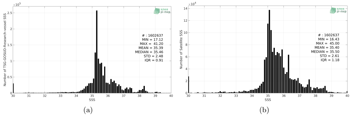
Figure 2: Histograms of SSS from TSG-GOSUD-Research-vessel (a) and SMAP-L3-RSS-V3-MONTHLY-0.25DEG-40KM (b) considering all match-up pairs per bins of 0.1 over the Global Ocean Pi-MEP region and for the full satellite product period.
