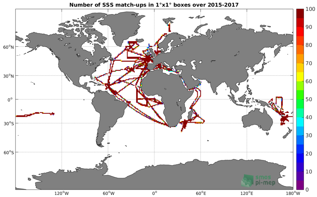
Figure 4: Number of SSS match-ups between TSG-GOSUD-Research-vessel SSS and the SMAP-L3-RSS-V3-MONTHLY-0.25DEG-40KM SSS product for the Global Ocean Pi-MEP region over 1^\circ \times 1^\circ boxes and for the full satellite product period.
