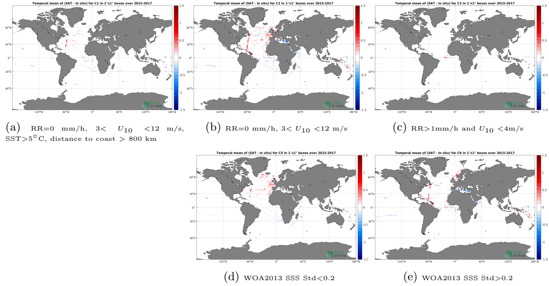
Figure 12: Temporal mean gridded over spatial boxes of size 1^\circ \times 1^\circ of \Delta SSS (SMAP-L3-RSS-V3-MONTHLY-0.25DEG-40KM - TSG-GOSUD-Research-vessel) for 5 different subdatasets corresponding to: RR=0 mm/h, 3 < U_{10} < 12 m/s, SST > 5^\circ C , distance to coast > 800 km (a), RR=0 mm/h, 3 < U_{10} < 12 m/s (b), RR > 1 mm/h and U_{10} < 4 m/s (c), WOA2013 SSS Std < 0.2 (d), WOA2013 SSS Std > 0.2 (e).
