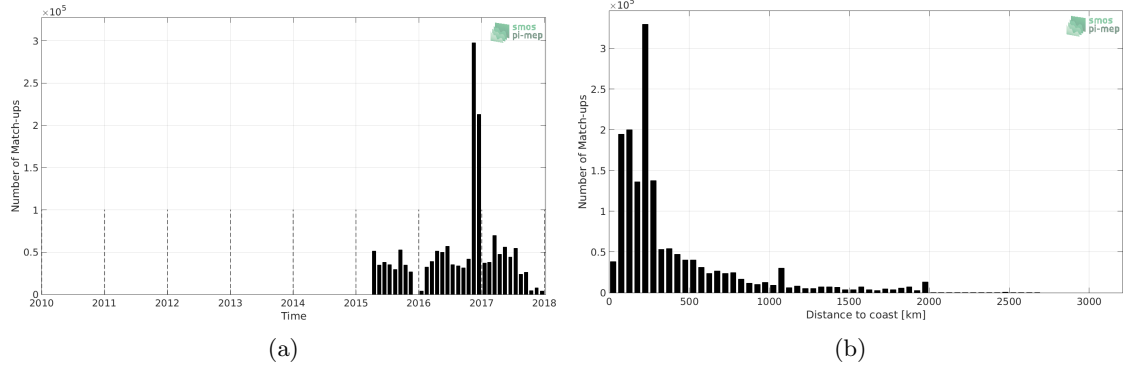
Figure 1: Number of match-ups between TSG-GOSUD-Research-vessel and SMAP-L3-RSS-V3-MONTHLY-0.25DEG-40KM SSS as a function of time (a) and as function of the distance to coast (b) over the Global Ocean Pi-MEP region and for the full satellite product period.
