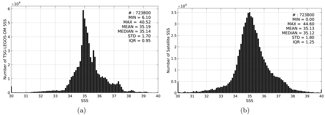
Figure 2: Histograms of SSS from TSG-LEGOS-DM (a) and SMAP-L3-RSS-V2-8DAY-RUNNING-40KM (b) considering all match-up pairs per bins of 0.1 over the Global Ocean Pi-MEP region and for the full satellite product period.
