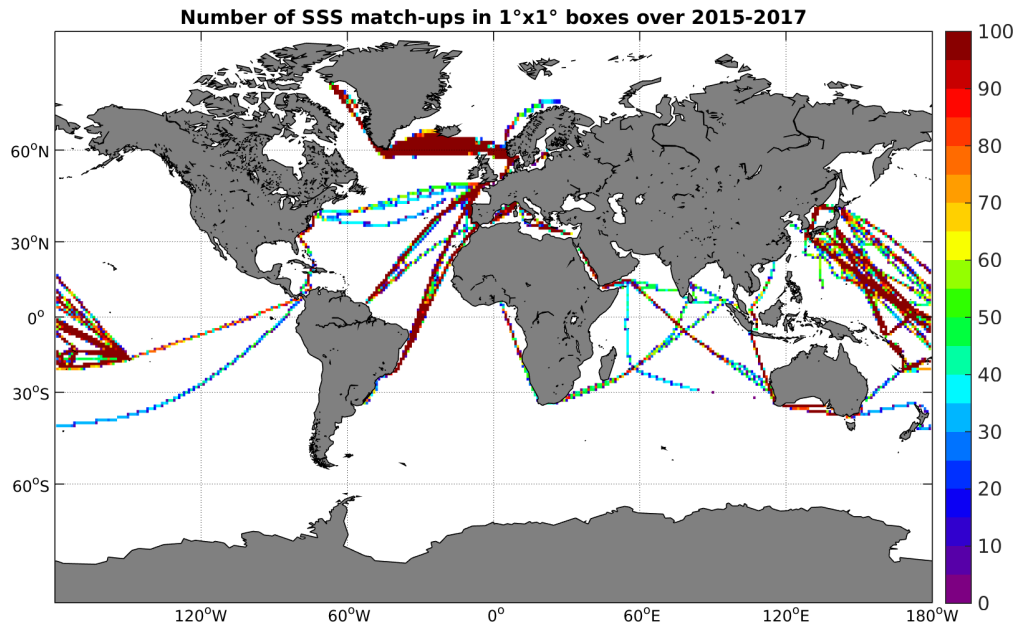
Figure 4: Number of SSS match-ups between TSG-LEGOS-DM SSS and the SMAP-L3-RSS-V2-8DAY-RUNNING-40KM SSS product for the Global Ocean Pi-MEP region over 1°x1° boxes and for the full satellite product period.
