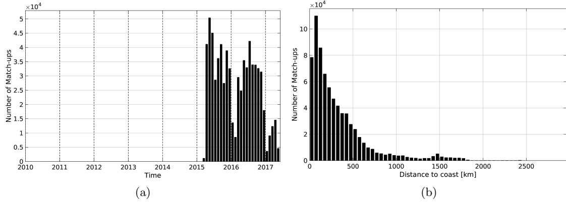
Figure 1: Number of match-ups between TSG-LEGOS-DM and SMAP-L3-RSS-V2-8DAY-RUNNING-40KM SSS as a function of time (a) and as function of the distance to coast (b) over the Global Ocean Pi-MEP region and for the full satellite product period.
