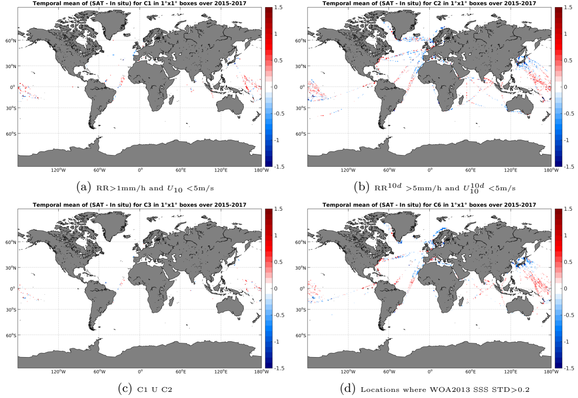
Figure 12: Temporal mean gridded over spatial boxes of size 1^\circ \times 1^\circ of \Delta SSS (SMAP-L3-RSS-V2-8DAY-RUNNING-40KM - TSG-LEGOS-DM) for 4 different subdatasets corresponding to: RR > 1\text{mm/h} and U_{10} < 5\text{m/s} (a), RR^{10d} > 5\text{mm/h} and U_{10}^{10d} < 5\text{m/s} (b), C1 U C2 (c), Locations where WOA2013 SSS STD > 0.2 (d).
