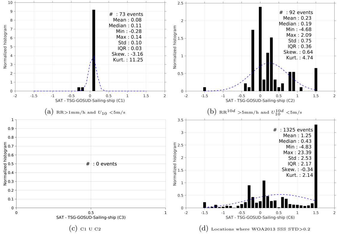
Figure 13: Normalized histogram of \Delta SSS (SMAP-L3-RSS-V2-8DAY-RUNNING-40KM - TSG-GOSUD-Sailing-ship) for 6 different subdatasets corresponding to: RR > 1\text{mm/h} and U_{10} < 5\text{m/s} (a), RR^{10d} > 5\text{mm/h} and U_{10}^{10d} < 5\text{m/s} (b), C1 U C2 (c), Locations where WOA2013 SSS STD > 0.2 (d).
