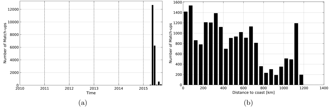
Figure 1: Number of match-ups between TSG-GOSUD-Sailing-ship and SMAP-L3-RSS-V2-8DAY-RUNNING-40KM SSS as a function of time (a) and as function of the distance to coast (b) over the Global Ocean Pi-MEP region and for the full satellite product period.
