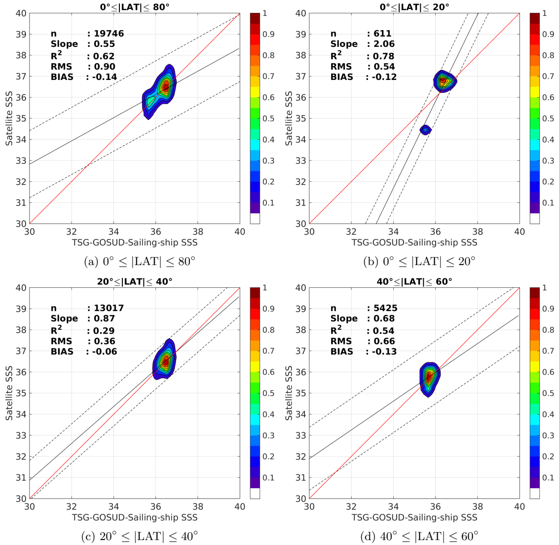
Figure 9: Contour maps of the concentration of SMAP-L3-RSS-V2-8DAY-RUNNING-40KM SSS (y-axis) versus TSG-GOSUD-Sailing-ship SSS (x-axis) at match-up pairs for different latitude bands. For each plot, the red line shows x=y . The black thin and dashed lines indicate a linear fit through the data cloud and the \pm 95\% confidence levels, respectively. The number match-up pairs n , the slope and R^2 coefficient of the linear fit, the root mean square (RMS) and the mean bias between satellite and in situ data are indicated for each latitude band in each plots.
