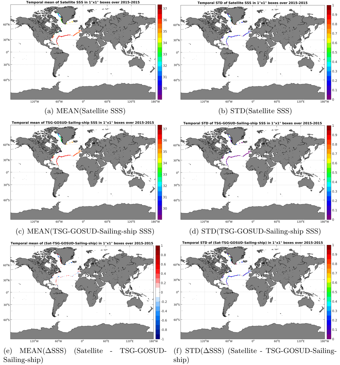
Figure 6: Temporal mean (left) and STD (right) of SSS from SMAP-L3-RSS-V2-8DAY-RUNNING-40KM (top), TSG-GOSUD-Sailing-ship (middle), and of \Delta SSS (Satellite - TSG-GOSUD-Sailing-ship). Only match-up pairs are used to generate these maps.
