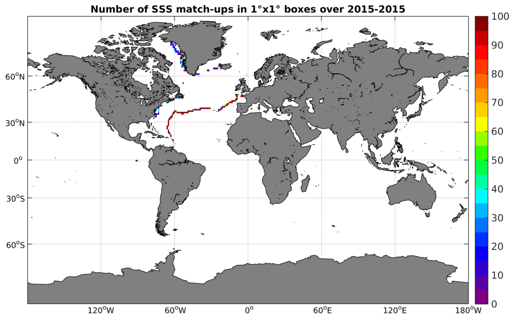
Figure 4: Number of SSS match-ups between TSG-GOSUD-Sailing-ship SSS and the SMAP-L3-RSS-V2-8DAY-RUNNING-40KM SSS product for the Global Ocean Pi-MEP region over 1°x1° boxes and for the full satellite product period.
