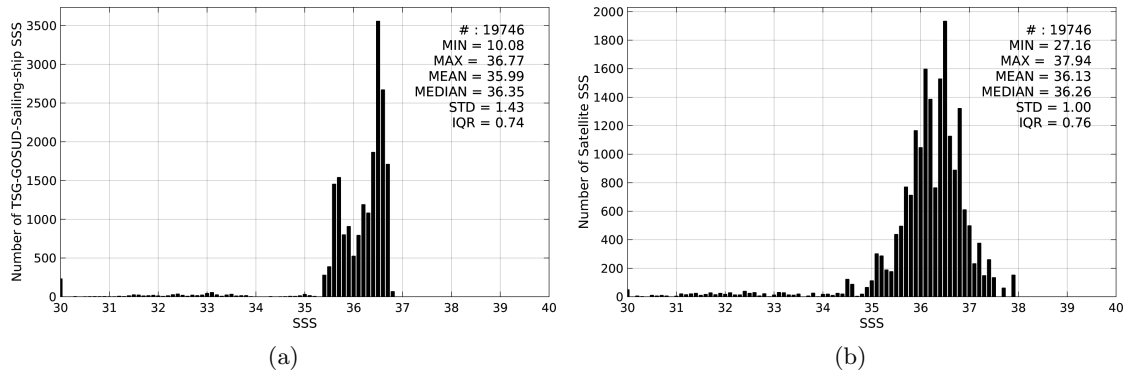
Figure 2: Histograms of SSS from TSG-GOSUD-Sailing-ship (a) and SMAP-L3-RSS-V2-8DAY-RUNNING-40KM (b) considering all match-up pairs per bins of 0.1 over the Global Ocean Pi-MEP region and for the full satellite product period.
