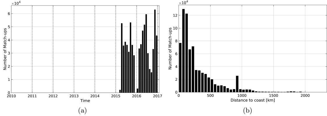
Figure 1: Number of match-ups between TSG-GOSUD-Research-vessel and SMAP-L3-RSS-V2-8DAY-RUNNING-40KM SSS as a function of time (a) and as function of the distance to coast (b) over the Global Ocean Pi-MEP region and for the full satellite product period.
