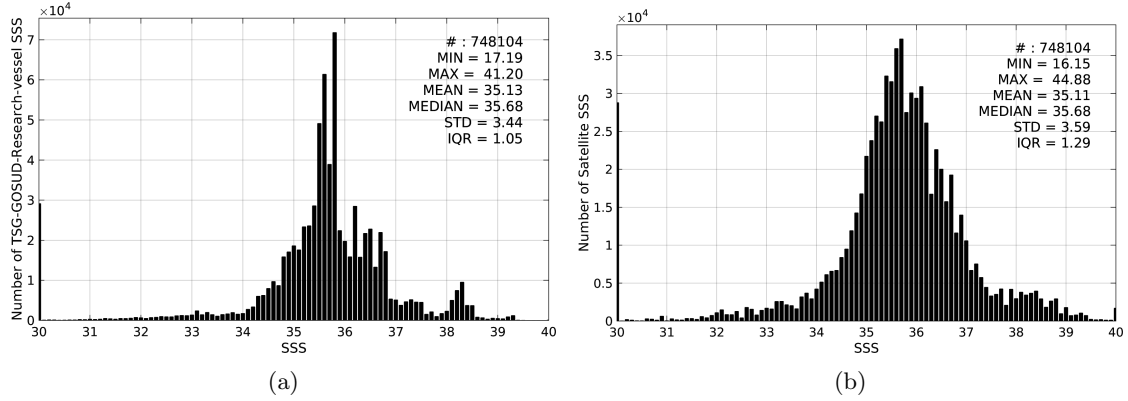
Figure 2: Histograms of SSS from TSG-GOSUD-Research-vessel (a) and SMAP-L3-RSS-V2-8DAY-RUNNING-40KM (b) considering all match-up pairs per bins of 0.1 over the Global Ocean Pi-MEP region and for the full satellite product period.
