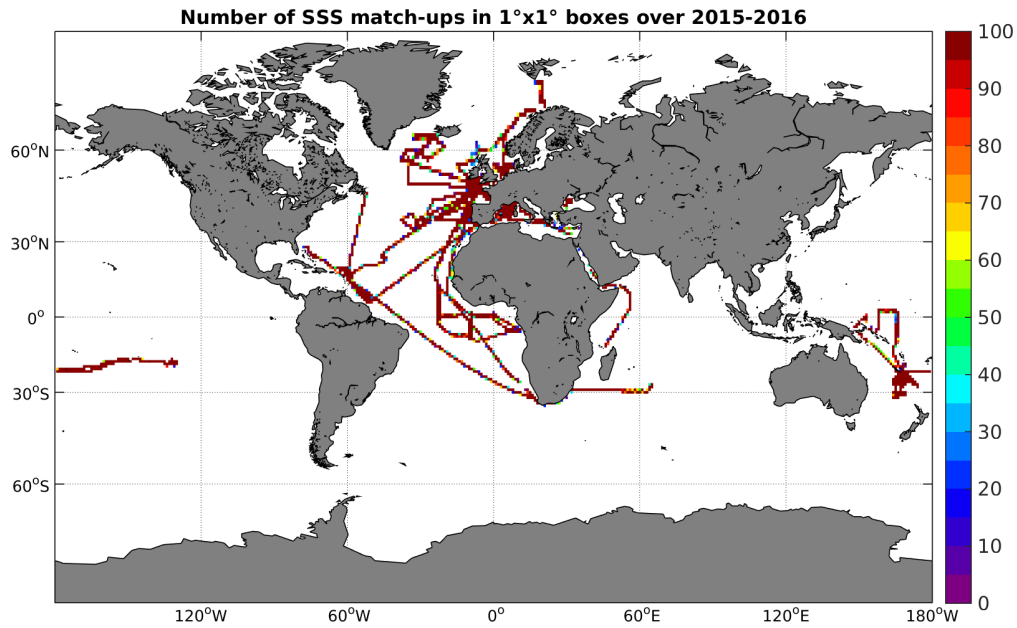
Figure 4: Number of SSS match-ups between TSG-GOSUD-Research-vessel SSS and the SMAP-L3-RSS-V2-8DAY-RUNNING-40KM SSS product for the Global Ocean Pi-MEP region over 1^\circ \times 1^\circ boxes and for the full satellite product period.
