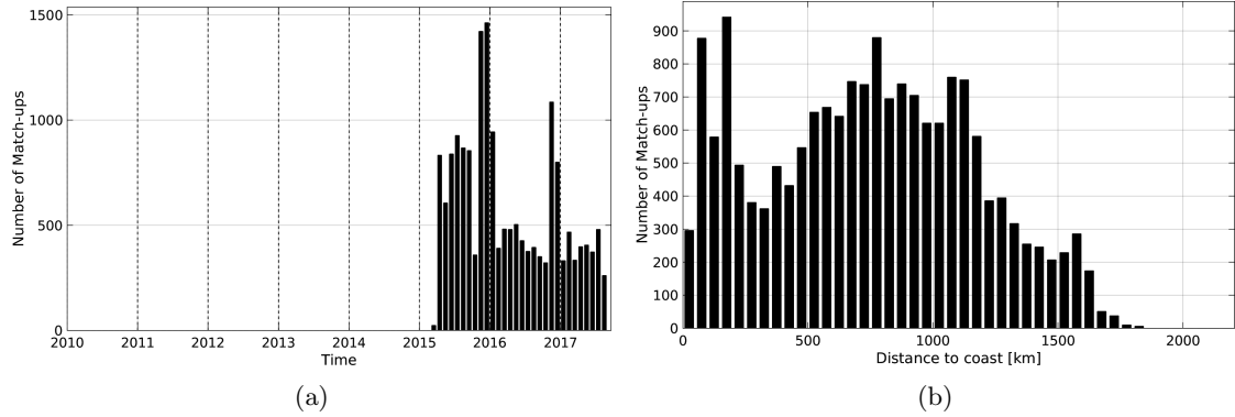
Figure 1: Number of match-ups between Sea mammals and SMAP-L3-RSS-V2-8DAY-RUNNING-40KM SSS as a function of time (a) and as function of the distance to coast (b) over the Global Ocean Pi-MEP region and for the full satellite product period.
