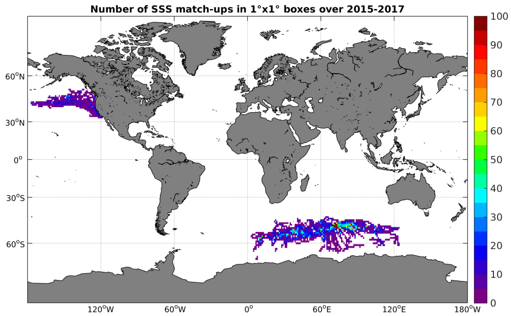
Figure 4: Number of SSS match-ups between Sea mammals SSS and the SMAP-L3-RSS-V2-8DAY-RUNNING-40KM SSS product for the Global Ocean Pi-MEP region over 1^\circ \times 1^\circ boxes and for the full satellite product period.
