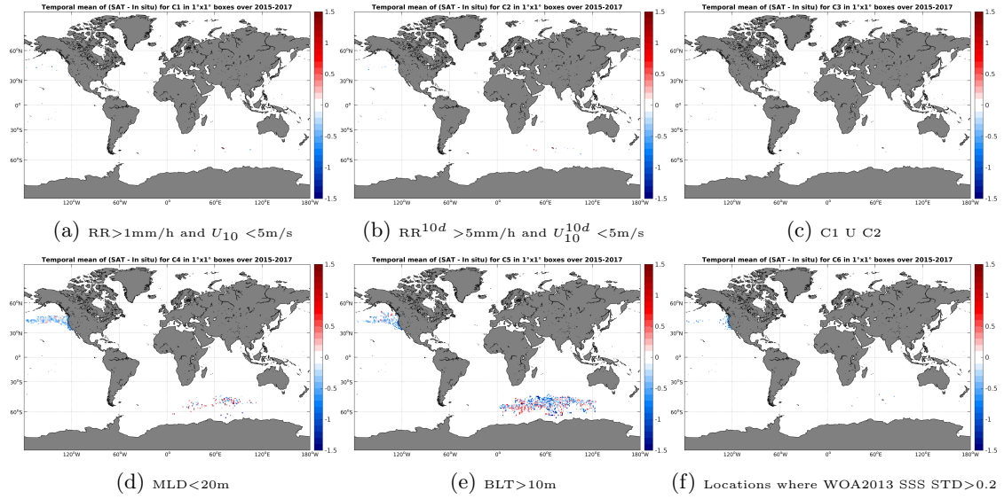
Figure 12: Temporal mean gridded over spatial boxes of size 1^\circ \times 1^\circ of \Delta SSS (SMAP-L3-RSS-V2-8DAY-RUNNING-40KM - Sea mammals) for 6 different subdatasets corresponding to: RR > 1\text{mm/h} and U_{10} < 5\text{m/s} (a), RR^{10d} > 5\text{mm/h} and U_{10}^{10d} < 5\text{m/s} (b), C1 U C2 (c), MLD < 20\text{m} (d), BLT > 10\text{m} (e), Locations where WOA2013 SSS STD > 0.2 (f).
