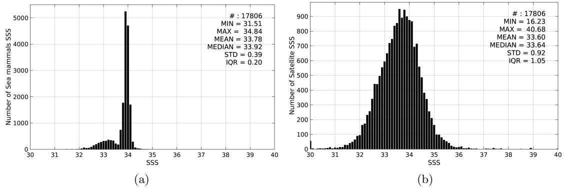
Figure 2: Histograms of SSS from Sea mammals (a) and SMAP-L3-RSS-V2-8DAY-RUNNING-40KM (b) considering all match-up pairs per bins of 0.1 over the Global Ocean Pi-MEP region and for the full satellite product period.
