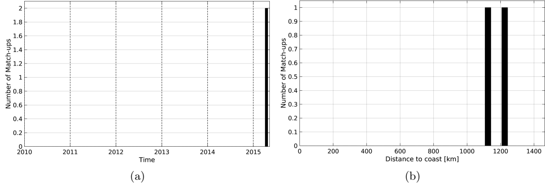
Figure 1: Number of match-ups between Surface drifters and SMAP-L3-RSS-V2-8DAY-RUNNING-40KM SSS as a function of time (a) and as function of the distance to coast (b) over the Global Ocean Pi-MEP region and for the full satellite product period.
