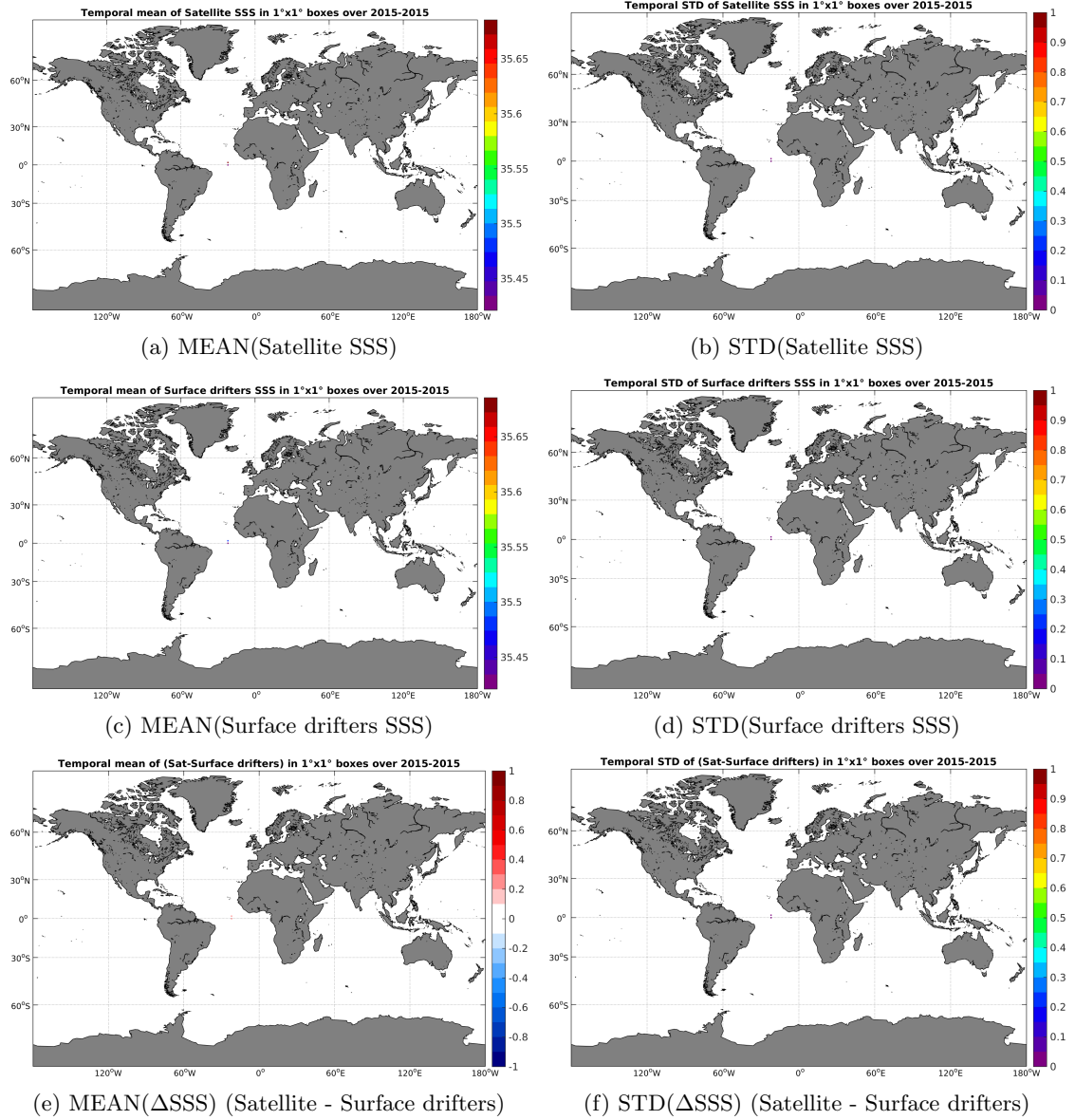
Figure 5: Temporal mean (left) and STD (right) of SSS from SMAP-L3-RSS-V2-8DAY-RUNNING-40KM (top), Surface drifters (middle), and of \Delta SSS (Satellite - Surface drifters). Only match-up pairs are used to generate these maps.
