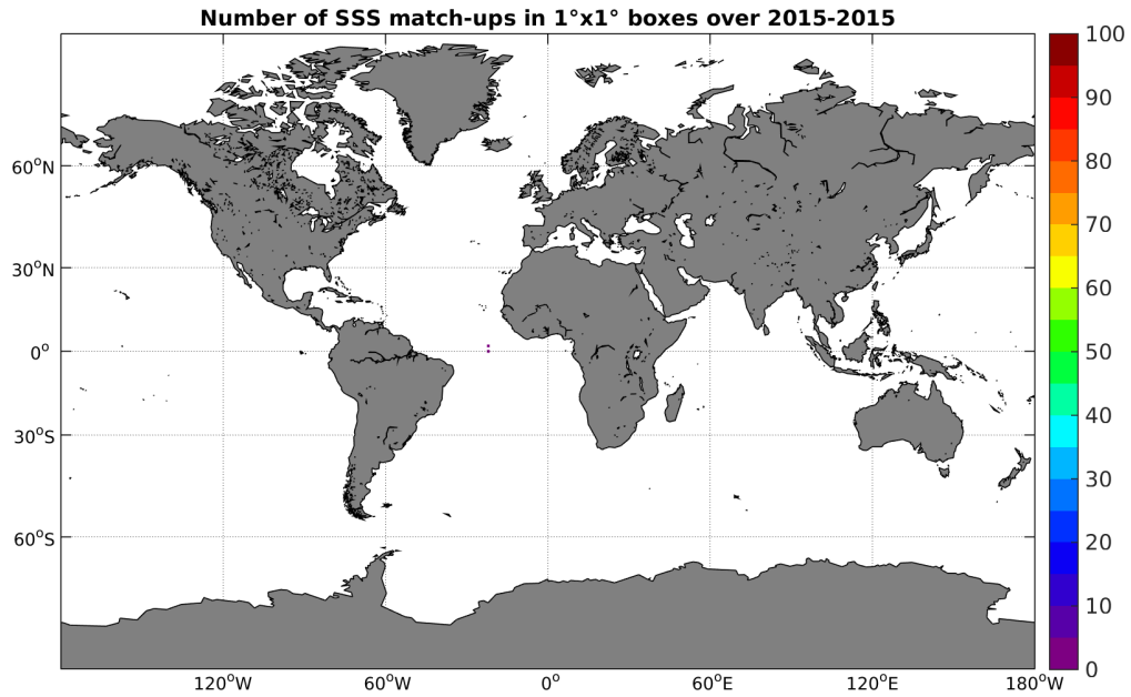
Figure 3: Number of SSS match-ups between Surface drifters SSS and the SMAP-L3-RSS-V2-8DAY-RUNNING-40KM SSS product for the Global Ocean Pi-MEP region over 1°x1° boxes and for the full satellite product period.
