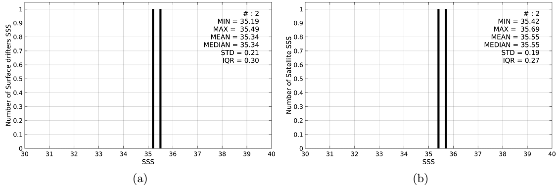
Figure 2: Histograms of SSS from Surface drifters (a) and SMAP-L3-RSS-V2-8DAY-RUNNING-40KM (b) considering all match-up pairs per bins of 0.1 over the Global Ocean Pi-MEP region and for the full satellite product period.
