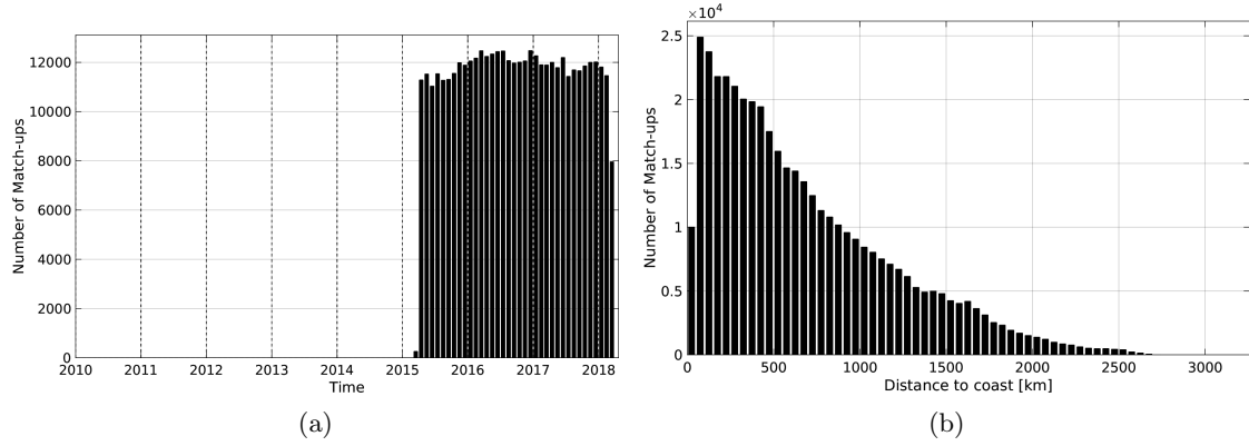
Figure 1: Number of match-ups between Argo and SMAP-L3-RSS-V2-8DAY-RUNNING-40KM SSS as a function of time (a) and as function of the distance to coast (b) over the Global Ocean Pi-MEP region and for the full satellite product period.
