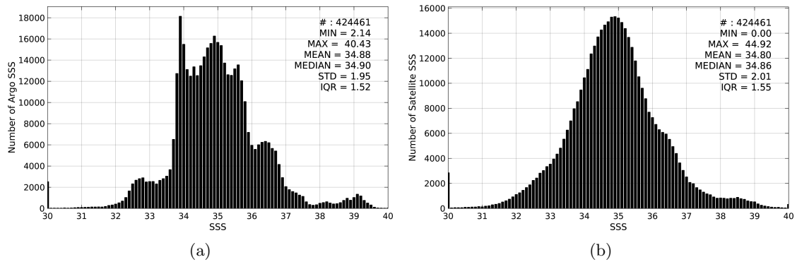
Figure 2: Histograms of SSS from Argo (a) and SMAP-L3-RSS-V2-8DAY-RUNNING-40KM (b) considering all match-up pairs per bins of 0.1 over the Global Ocean Pi-MEP region and for the full satellite product period.
