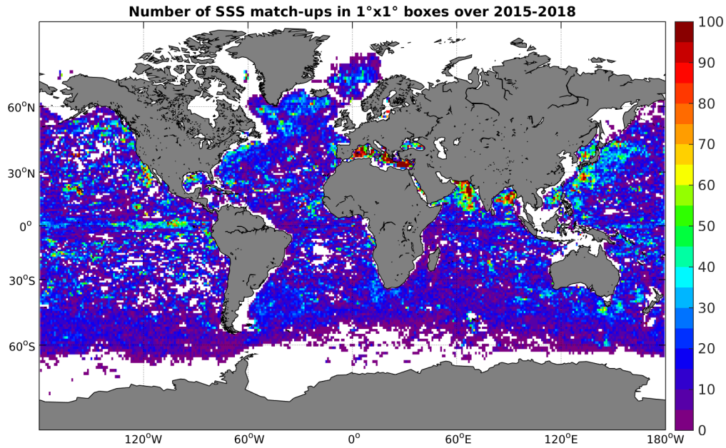
Figure 4: Number of SSS match-ups between Argo SSS and the SMAP-L3-RSS-V2-8DAY-RUNNING-40KM SSS product for the Global Ocean Pi-MEP region over 1^\circ \times 1^\circ boxes and for the full satellite product period.
