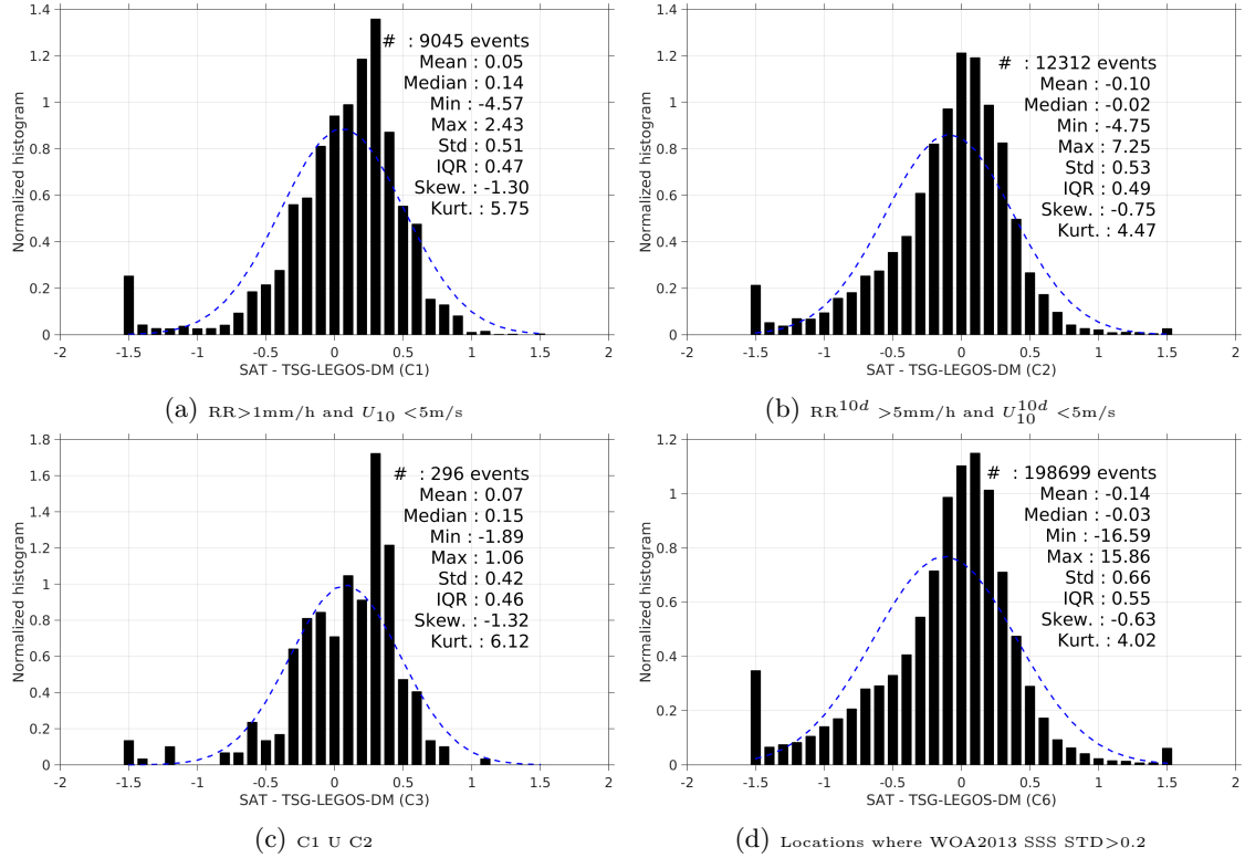
Figure 13: Normalized histogram of \Delta SSS (SMAP-L3-RSS-V2-8DAY-RUNNING-70KM - TSG-LEGOS-DM) for 6 different subdatasets corresponding to: RR > 1mm/h and U_{10} < 5 m/s (a), RR^{10d} > 5 mm/h and U_{10}^{10d} < 5 m/s (b), C1 U C2 (c), Locations where WOA2013 SSS STD > 0.2 (d).
