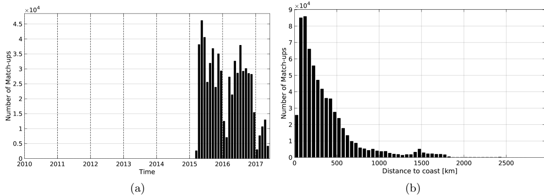
Figure 1: Number of match-ups between TSG-LEGOS-DM and SMAP-L3-RSS-V2-8DAY-RUNNING-70KM SSS as a function of time (a) and as function of the distance to coast (b) over the Global Ocean Pi-MEP region and for the full satellite product period.
