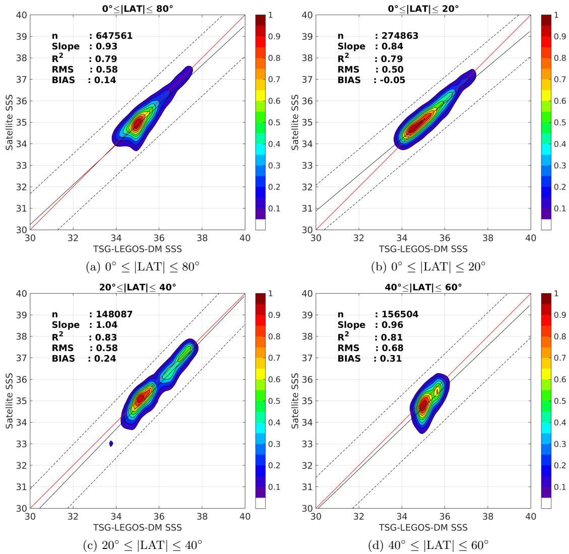
Figure 9: Contour maps of the concentration of SMAP-L3-RSS-V2-8DAY-RUNNING-70KM SSS (y-axis) versus TSG-LEGOS-DM SSS (x-axis) at match-up pairs for different latitude bands. For each plot, the red line shows x=y . The black thin and dashed lines indicate a linear fit through the data cloud and the \pm 95\% confidence levels, respectively. The number match-up pairs n , the slope and R^2 coefficient of the linear fit, the root mean square (RMS) and the mean bias between satellite and in situ data are indicated for each latitude band in each plots.
