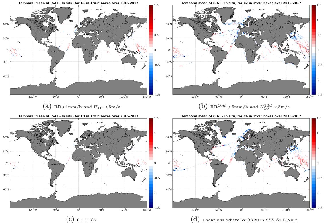
Figure 12: Temporal mean gridded over spatial boxes of size 1^\circ \times 1^\circ of \Delta SSS (SMAP-L3-RSS-V2-8DAY-RUNNING-70KM - TSG-LEGOS-DM) for 4 different subdatasets corresponding to: RR > 1\text{mm/h} and U_{10} < 5\text{m/s} (a), RR^{10d} > 5\text{mm/h} and U_{10}^{10d} < 5\text{m/s} (b), C1 U C2 (c), Locations where WOA2013 SSS STD > 0.2 (d).
