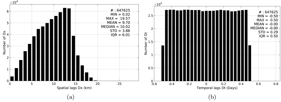
Figure 5: Histograms of the spatial (a) and temporal (b) lags between the time of the TSG-LEGOS-DM measurements and the date of the corresponding SMAP-L3-RSS-V2-8DAY-RUNNING-70KM SSS product.
