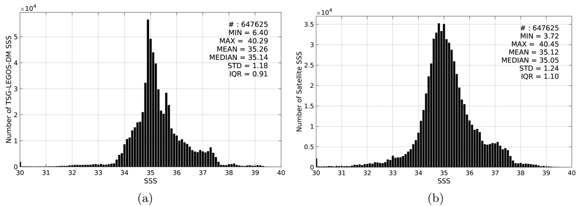
Figure 2: Histograms of SSS from TSG-LEGOS-DM (a) and SMAP-L3-RSS-V2-8DAY-RUNNING-70KM (b) considering all match-up pairs per bins of 0.1 over the Global Ocean Pi-MEP region and for the full satellite product period.
