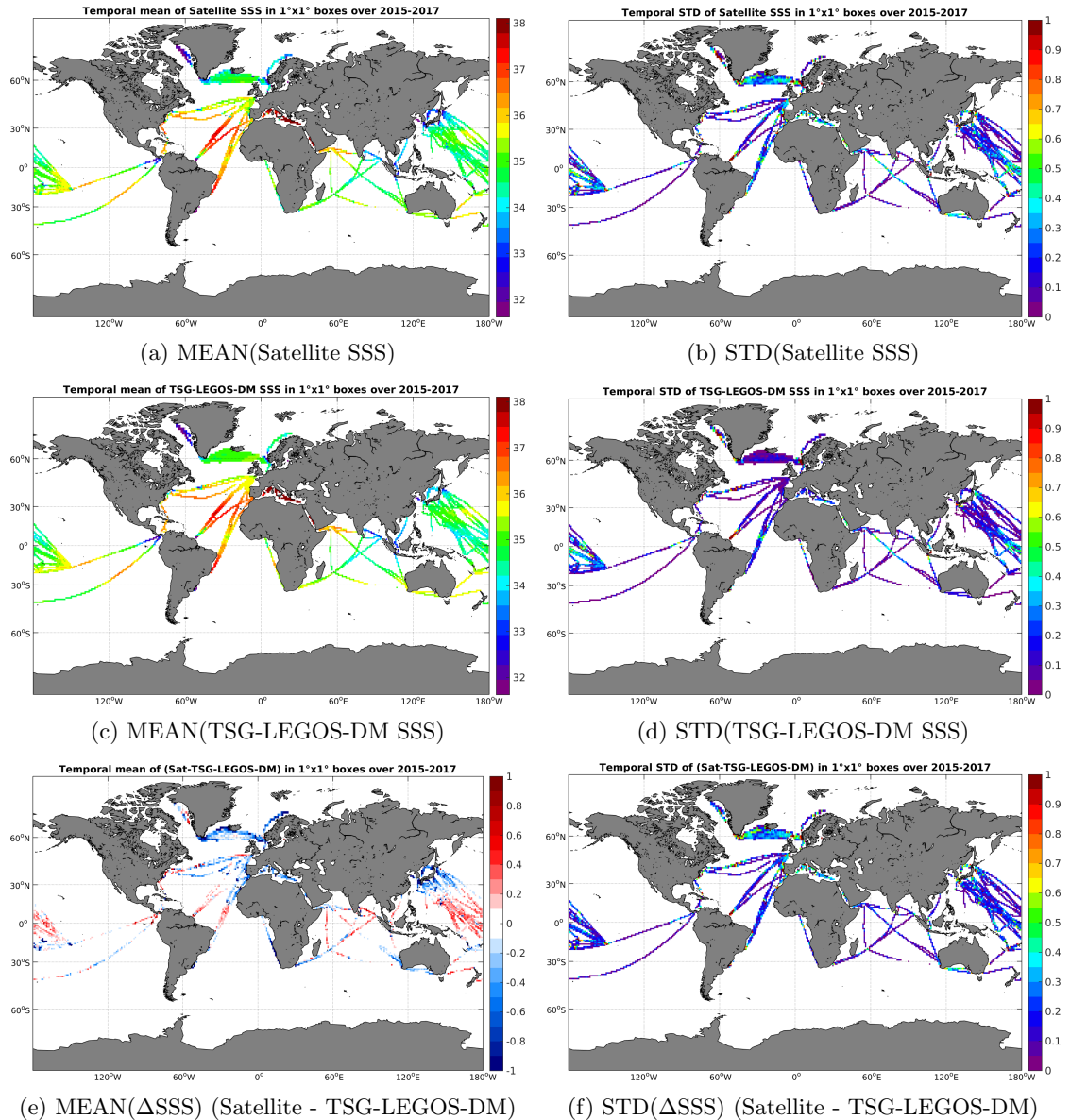
Figure 6: Temporal mean (left) and STD (right) of SSS from SMAP-L3-RSS-V2-8DAY-RUNNING-70KM (top), TSG-LEGOS-DM (middle), and of \Delta SSS (Satellite - TSG-LEGOS-DM). Only match-up pairs are used to generate these maps.
