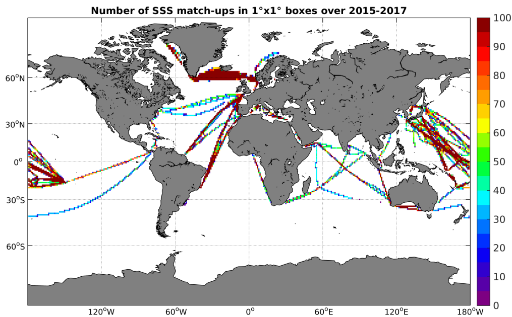
Figure 4: Number of SSS match-ups between TSG-LEGOS-DM SSS and the SMAP-L3-RSS-V2-8DAY-RUNNING-70KM SSS product for the Global Ocean Pi-MEP region over 1°x1° boxes and for the full satellite product period.
