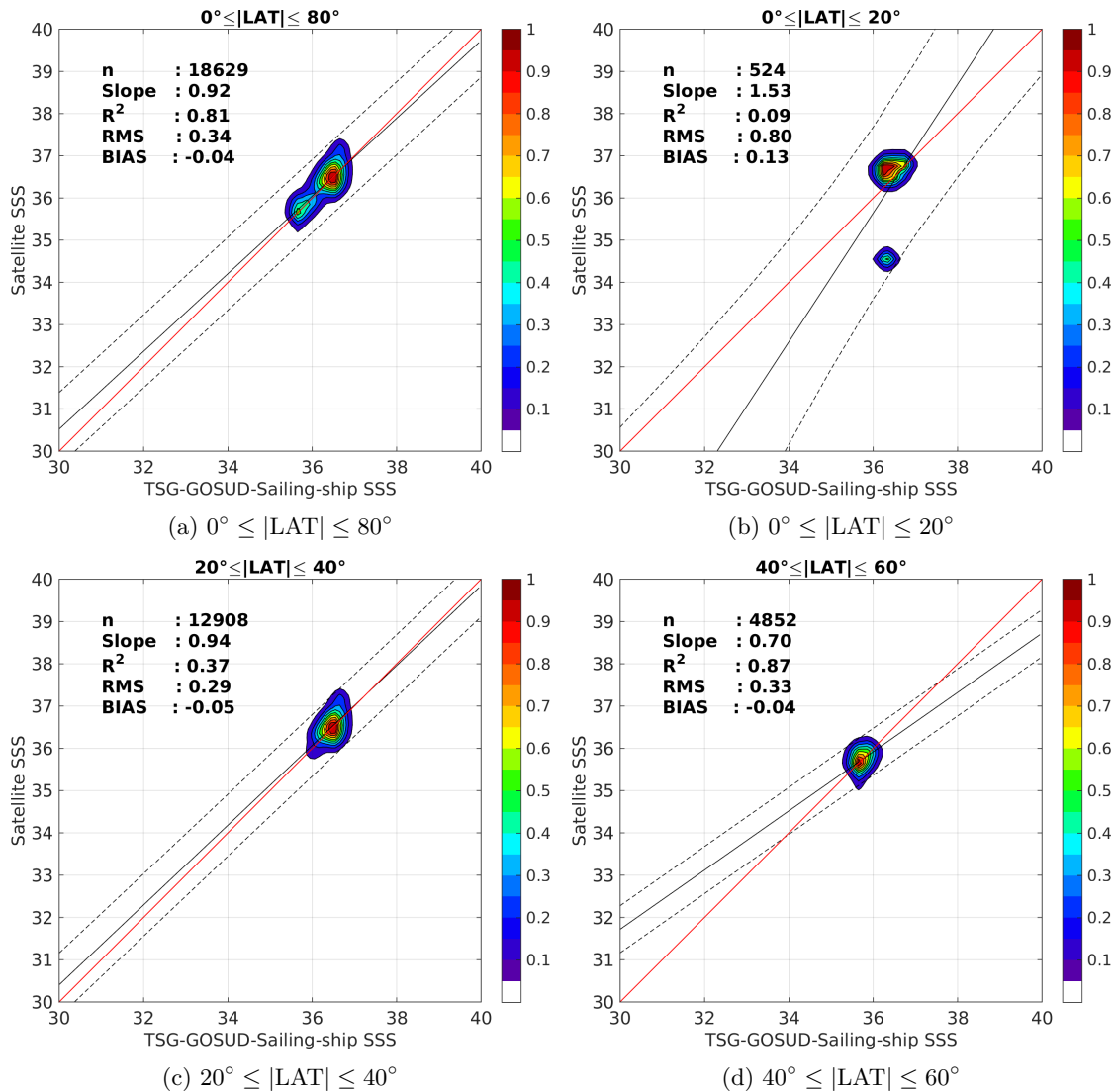
Figure 9: Contour maps of the concentration of SMAP-L3-RSS-V2-8DAY-RUNNING-70KM SSS (y-axis) versus TSG-GOSUD-Sailing-ship SSS (x-axis) at match-up pairs for different latitude bands. For each plot, the red line shows x=y . The black thin and dashed lines indicate a linear fit through the data cloud and the \pm 95\% confidence levels, respectively. The number match-up pairs n , the slope and R^2 coefficient of the linear fit, the root mean square (RMS) and the mean bias between satellite and in situ data are indicated for each latitude band in each plots.
