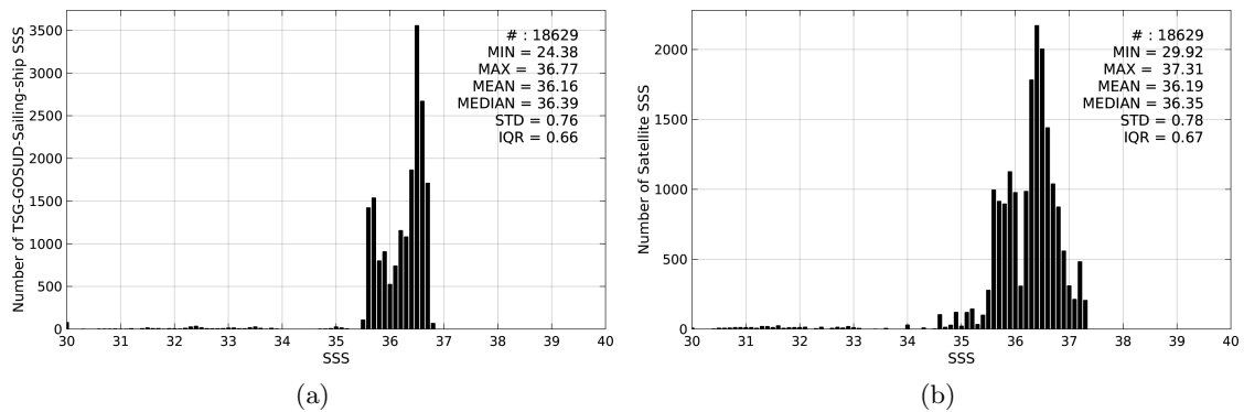
Figure 2: Histograms of SSS from TSG-GOSUD-Sailing-ship (a) and SMAP-L3-RSS-V2-8DAY-RUNNING-70KM (b) considering all match-up pairs per bins of 0.1 over the Global Ocean Pi-MEP region and for the full satellite product period.
