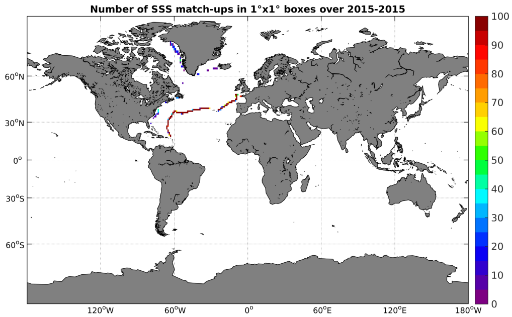
Figure 4: Number of SSS match-ups between TSG-GOSUD-Sailing-ship SSS and the SMAP-L3-RSS-V2-8DAY-RUNNING-70KM SSS product for the Global Ocean Pi-MEP region over 1^\circ \times 1^\circ boxes and for the full satellite product period.
