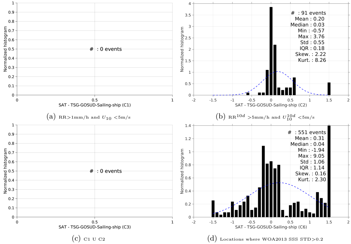
Figure 13: Normalized histogram of \Delta\text{SSS} (SMAP-L3-RSS-V2-8DAY-RUNNING-70KM - TSG-GOSUD-Sailing-ship) for 6 different subdatasets corresponding to: RR > 1\text{mm/h} and U_{10} < 5\text{m/s} (a), RR^{10d} > 5\text{mm/h} and U_{10}^{10d} < 5\text{m/s} (b), C1 U C2 (c), Locations where WOA2013 SSS STD > 0.2 (d).
