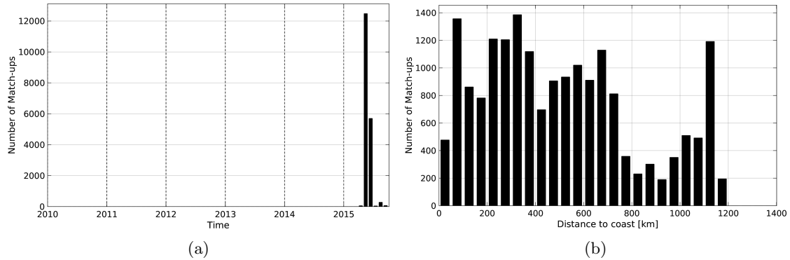
Figure 1: Number of match-ups between TSG-GOSUD-Sailing-ship and SMAP-L3-RSS-V2-8DAY-RUNNING-70KM SSS as a function of time (a) and as function of the distance to coast (b) over the Global Ocean Pi-MEP region and for the full satellite product period.
