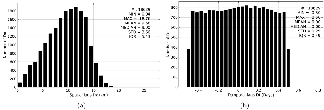
Figure 5: Histograms of the spatial (a) and temporal (b) lags between the time of the TSG-GOSUD-Sailing-ship measurements and the date of the corresponding SMAP-L3-RSS-V2-8DAY-RUNNING-70KM SSS product.
