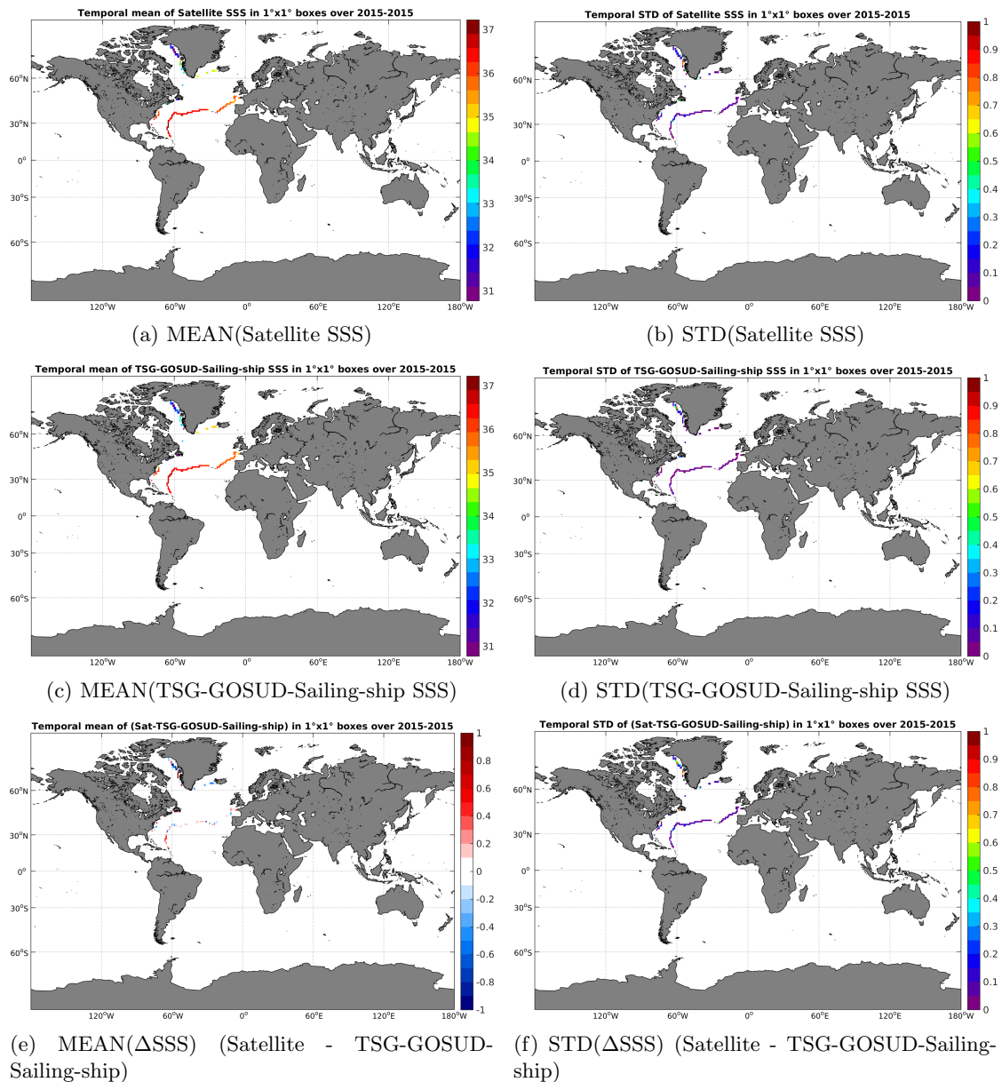
Figure 6: Temporal mean (left) and STD (right) of SSS from SMAP-L3-RSS-V2-8DAY-RUNNING-70KM (top), TSG-GOSUD-Sailing-ship (middle), and of \Delta SSS (Satellite - TSG-GOSUD-Sailing-ship). Only match-up pairs are used to generate these maps.
