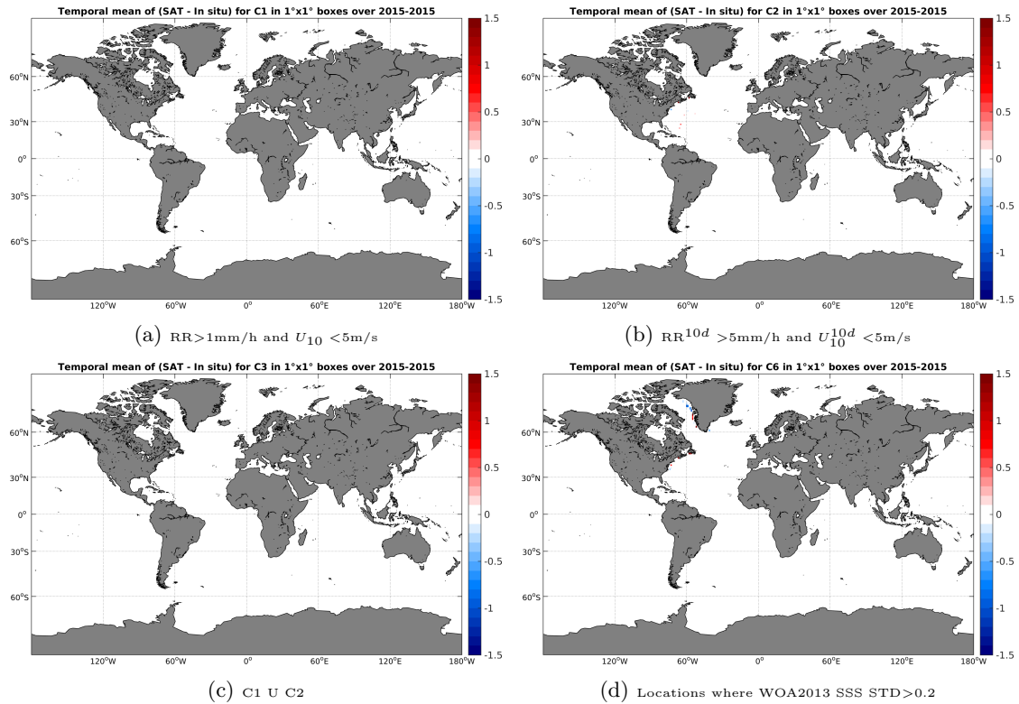
Figure 12: Temporal mean gridded over spatial boxes of size 1^\circ \times 1^\circ of \Delta SSS (SMAP-L3-RSS-V2-8DAY-RUNNING-70KM - TSG-GOSUD-Sailing-ship) for 4 different subdatasets corresponding to: RR > 1\text{mm/h} and U_{10} < 5\text{m/s} (a), RR^{10d} > 5\text{mm/h} and U_{10}^{10d} < 5\text{m/s} (b), C1 U C2 (c), Locations where WOA2013 SSS STD > 0.2 (d).
