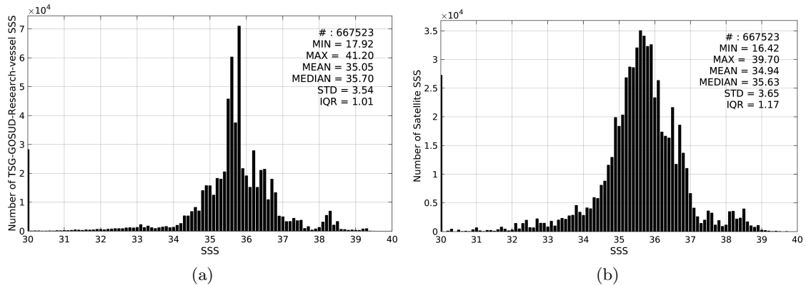
Figure 2: Histograms of SSS from TSG-GOSUD-Research-vessel (a) and SMAP-L3-RSS-V2-8DAY-RUNNING-70KM (b) considering all match-up pairs per bins of 0.1 over the Global Ocean Pi-MEP region and for the full satellite product period.
