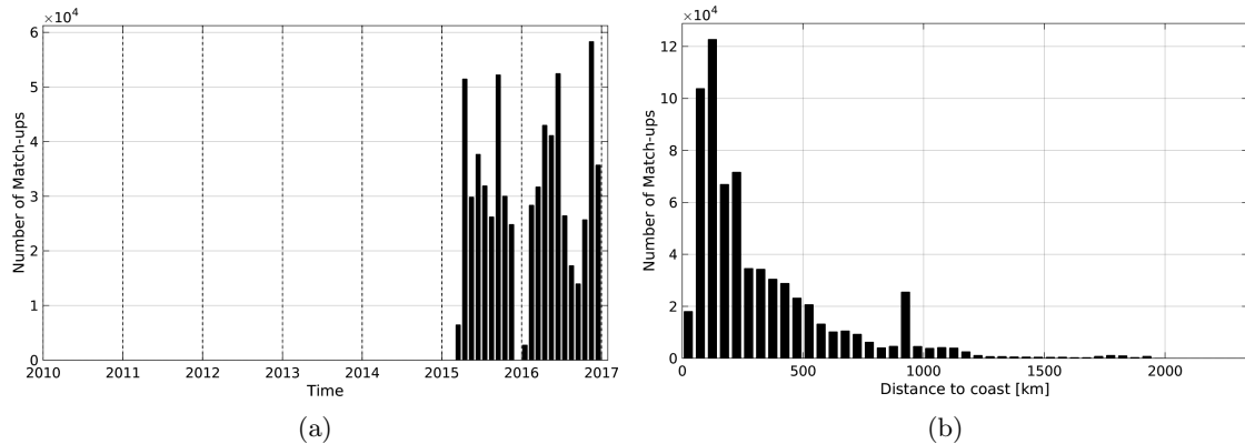
Figure 1: Number of match-ups between TSG-GOSUD-Research-vessel and SMAP-L3-RSS-V2-8DAY-RUNNING-70KM SSS as a function of time (a) and as function of the distance to coast (b) over the Global Ocean Pi-MEP region and for the full satellite product period.
