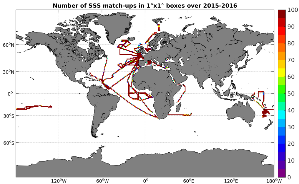
Figure 4: Number of SSS match-ups between TSG-GOSUD-Research-vessel SSS and the SMAP-L3-RSS-V2-8DAY-RUNNING-70KM SSS product for the Global Ocean Pi-MEP region over 1^\circ \times 1^\circ boxes and for the full satellite product period.
