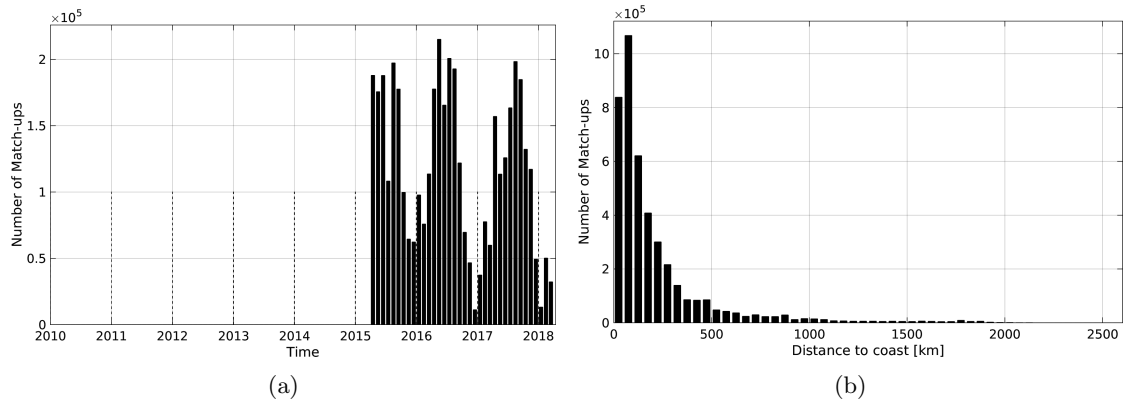
Figure 1: Number of match-ups between TSG-SAMOS and SMAP-L3-RSS-V2-MONTHLY-0.25DEG-40KM SSS as a function of time (a) and as function of the distance to coast (b) over the Global Ocean Pi-MEP region and for the full satellite product period.
