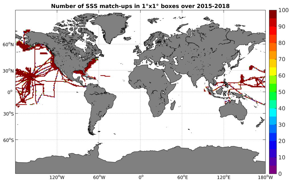
Figure 4: Number of SSS match-ups between TSG-SAMOS SSS and the SMAP-L3-RSS-V2-MONTHLY-0.25DEG-40KM SSS product for the Global Ocean Pi-MEP region over 1^\circ \times 1^\circ boxes and for the full satellite product period.
