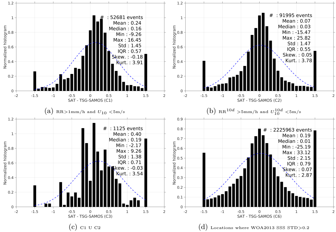
Figure 13: Normalized histogram of \Delta\text{SSS} (SMAP-L3-RSS-V2-MONTHLY-0.25DEG-40KM - TSG-SAMOS) for 6 different subdatasets corresponding to: \text{RR} > 1\text{mm/h} and U_{10} < 5\text{m/s} (a), \text{RR}^{10d} > 5\text{mm/h} and U_{10}^{10d} < 5\text{m/s} (b), C1 \cup C2 (c), Locations where WOA2013 SSS STD > 0.2 (d).
