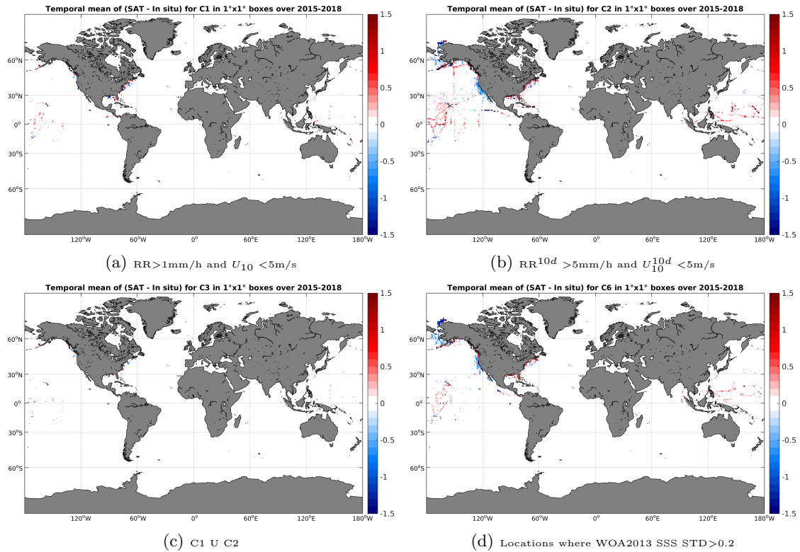
Figure 12: Temporal mean gridded over spatial boxes of size 1^\circ \times 1^\circ of \Delta SSS (SMAP-L3-RSS-V2-MONTHLY-0.25DEG-40KM - TSG-SAMOS) for 4 different subdatasets corresponding to: RR > 1\text{mm/h} and U_{10} < 5\text{m/s} (a), RR^{10d} > 5\text{mm/h} and U_{10}^{10d} < 5\text{m/s} (b), C1 U C2 (c), Locations where WOA2013 SSS STD > 0.2 (d).
