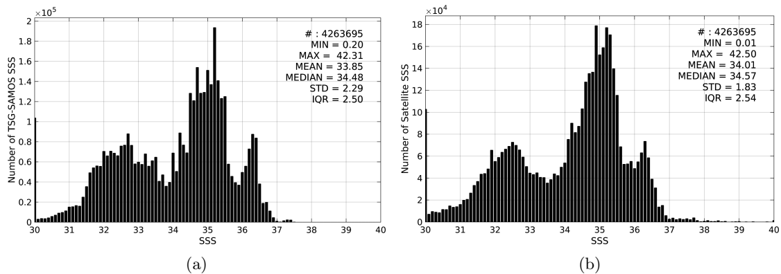
Figure 2: Histograms of SSS from TSG-SAMOS (a) and SMAP-L3-RSS-V2-MONTHLY-0.25DEG-40KM (b) considering all match-up pairs per bins of 0.1 over the Global Ocean Pi-MEP region and for the full satellite product period.
