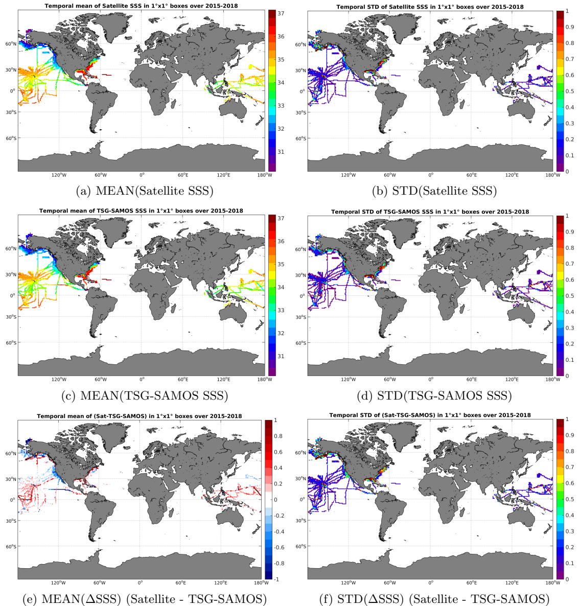
Figure 6: Temporal mean (left) and STD (right) of SSS from SMAP-L3-RSS-V2-MONTHLY-0.25DEG-40KM (top), TSG-SAMOS (middle), and of \Delta SSS (Satellite - TSG-SAMOS). Only match-up pairs are used to generate these maps.
