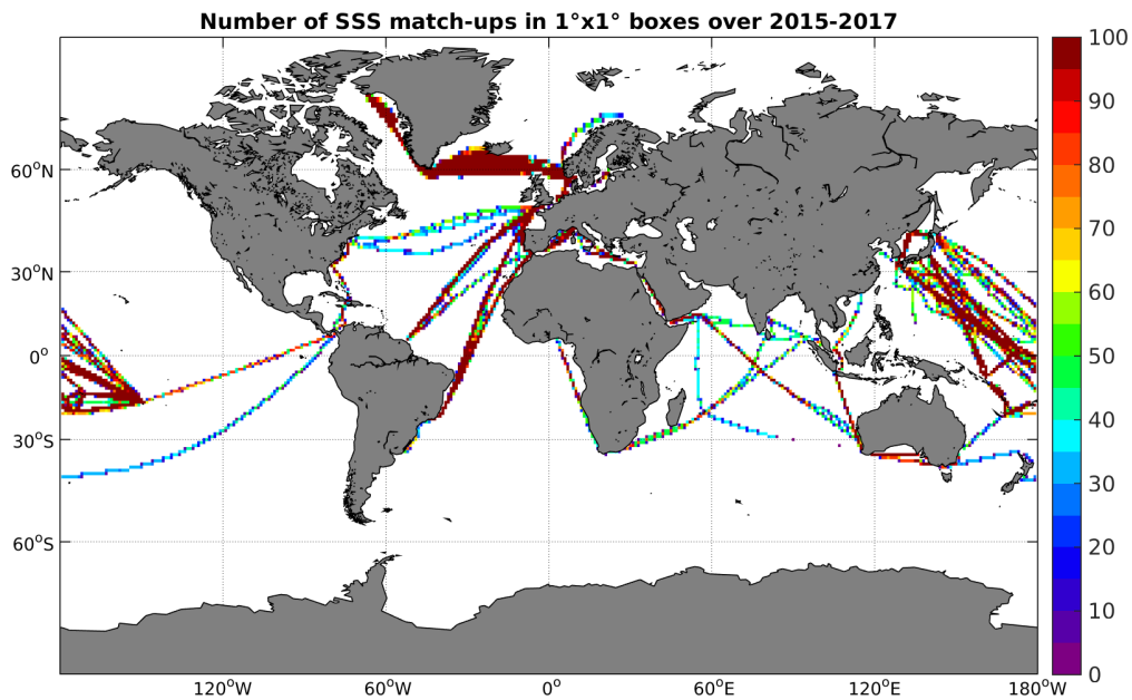
Figure 4: Number of SSS match-ups between TSG-LEGOS-DM SSS and the SMAP-L3-RSS-V2-MONTHLY-0.25DEG-40KM SSS product for the Global Ocean Pi-MEP region over 1^\circ \times 1^\circ boxes and for the full satellite product period.
