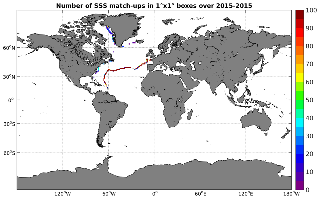
Figure 4: Number of SSS match-ups between TSG-GOSUD-Sailing-ship SSS and the SMAP-L3-RSS-V2-MONTHLY-0.25DEG-40KM SSS product for the Global Ocean Pi-MEP region over 1^\circ \times 1^\circ boxes and for the full satellite product period.
