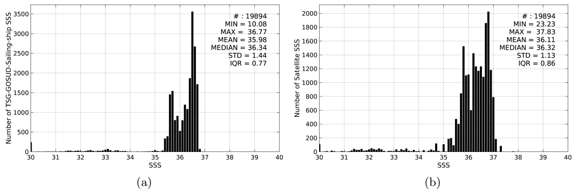
Figure 2: Histograms of SSS from TSG-GOSUD-Sailing-ship (a) and SMAP-L3-RSS-V2-MONTHLY-0.25DEG-40KM (b) considering all match-up pairs per bins of 0.1 over the Global Ocean Pi-MEP region and for the full satellite product period.
