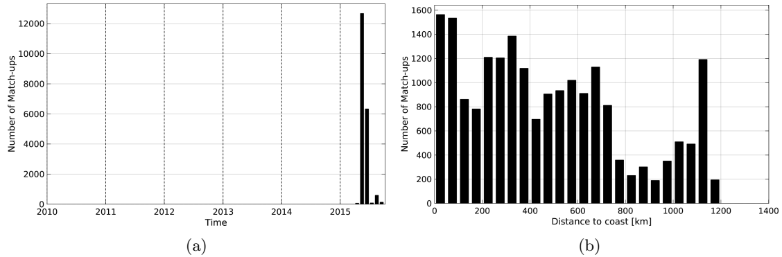
Figure 1: Number of match-ups between TSG-GOSUD-Sailing-ship and SMAP-L3-RSS-V2-MONTHLY-0.25DEG-40KM SSS as a function of time (a) and as function of the distance to coast (b) over the Global Ocean Pi-MEP region and for the full satellite product period.
