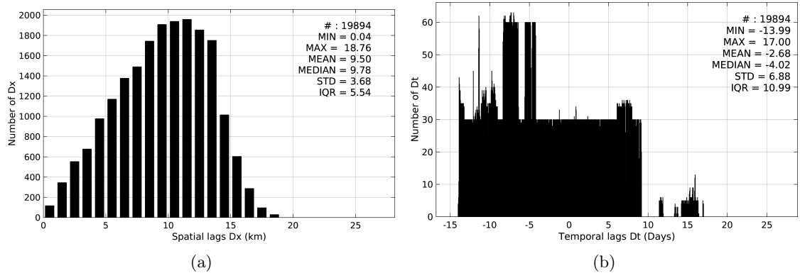
Figure 5: Histograms of the spatial (a) and temporal (b) lags between the time of the TSG-GOSUD-Sailing-ship measurements and the date of the corresponding SMAP-L3-RSS-V2-MONTHLY-0.25DEG-40KM SSS product.
