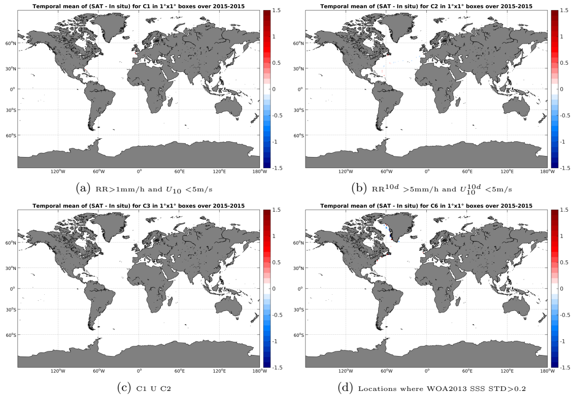
Figure 12: Temporal mean gridded over spatial boxes of size 1^\circ \times 1^\circ of \Delta SSS (SMAP-L3-RSS-V2-MONTHLY-0.25DEG-40KM - TSG-GOSUD-Sailing-ship) for 4 different subdatasets corresponding to: RR > 1\text{mm/h} and U_{10} < 5\text{m/s} (a), RR^{10d} > 5\text{mm/h} and U_{10}^{10d} < 5\text{m/s} (b), C1 U C2 (c), Locations where WOA2013 SSS STD > 0.2 (d).
