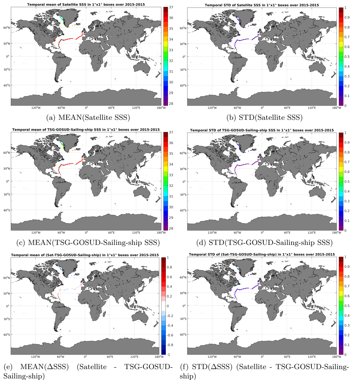
Figure 6: Temporal mean (left) and STD (right) of SSS from SMAP-L3-RSS-V2-MONTHLY-0.25DEG-40KM (top), TSG-GOSUD-Sailing-ship (middle), and of \Delta SSS (Satellite - TSG-GOSUD-Sailing-ship). Only match-up pairs are used to generate these maps.
