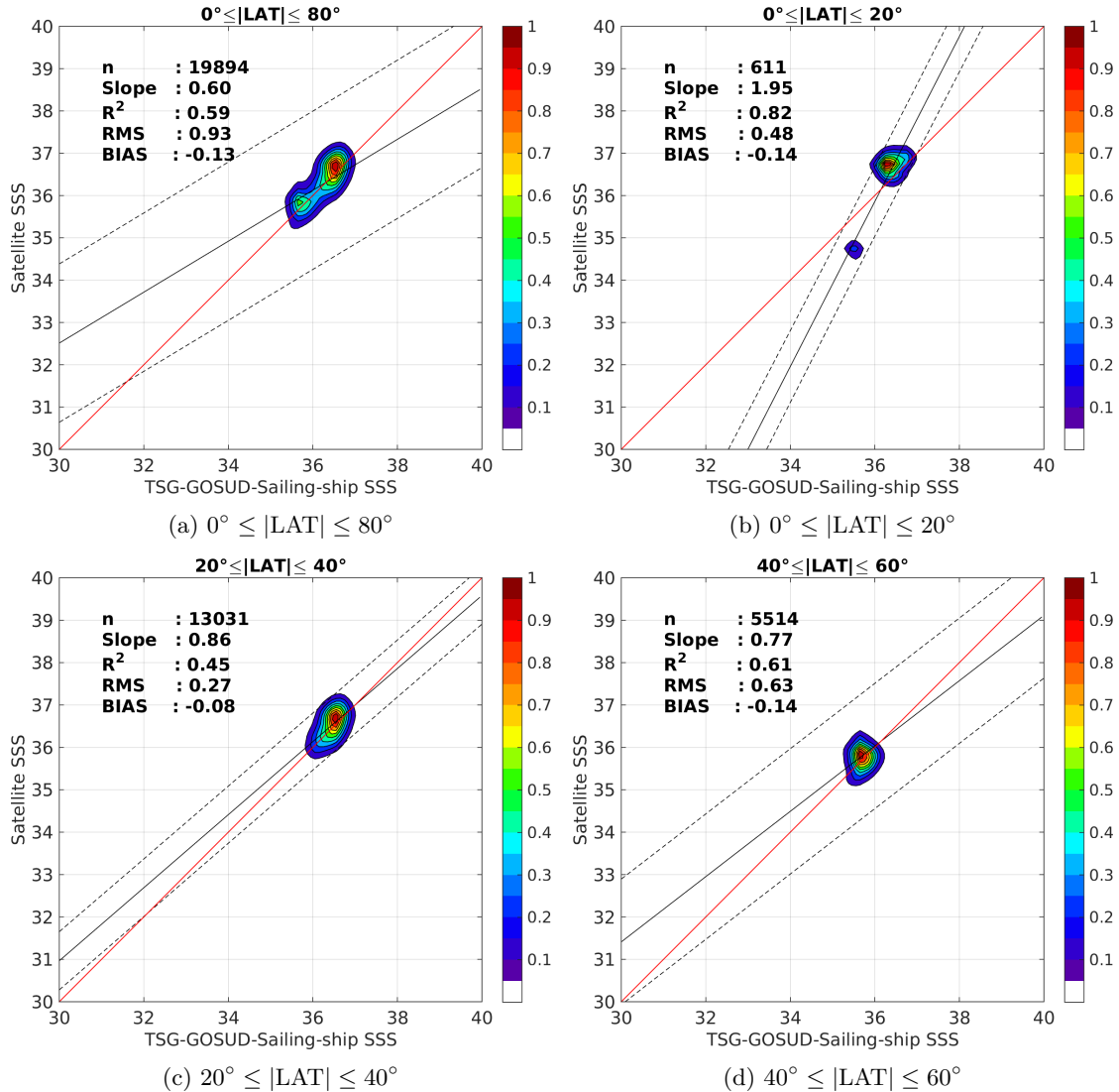
Figure 9: Contour maps of the concentration of SMAP-L3-RSS-V2-MONTHLY-0.25DEG-40KM SSS (y-axis) versus TSG-GOSUD-Sailing-ship SSS (x-axis) at match-up pairs for different latitude bands. For each plot, the red line shows x=y . The black thin and dashed lines indicate a linear fit through the data cloud and the \pm 95\% confidence levels, respectively. The number match-up pairs n , the slope and R^2 coefficient of the linear fit, the root mean square (RMS) and the mean bias between satellite and in situ data are indicated for each latitude band in each plots.
