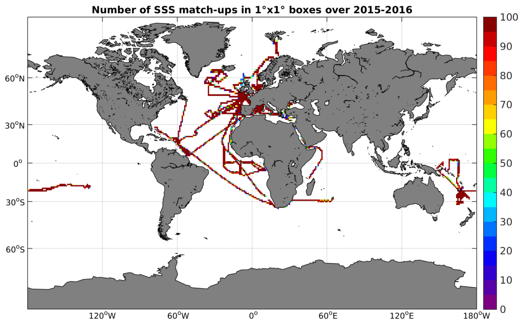
Figure 4: Number of SSS match-ups between TSG-GOSUD-Research-vessel SSS and the SMAP-L3-RSS-V2-MONTHLY-0.25DEG-40KM SSS product for the Global Ocean Pi-MEP region over 1^\circ \times 1^\circ boxes and for the full satellite product period.
