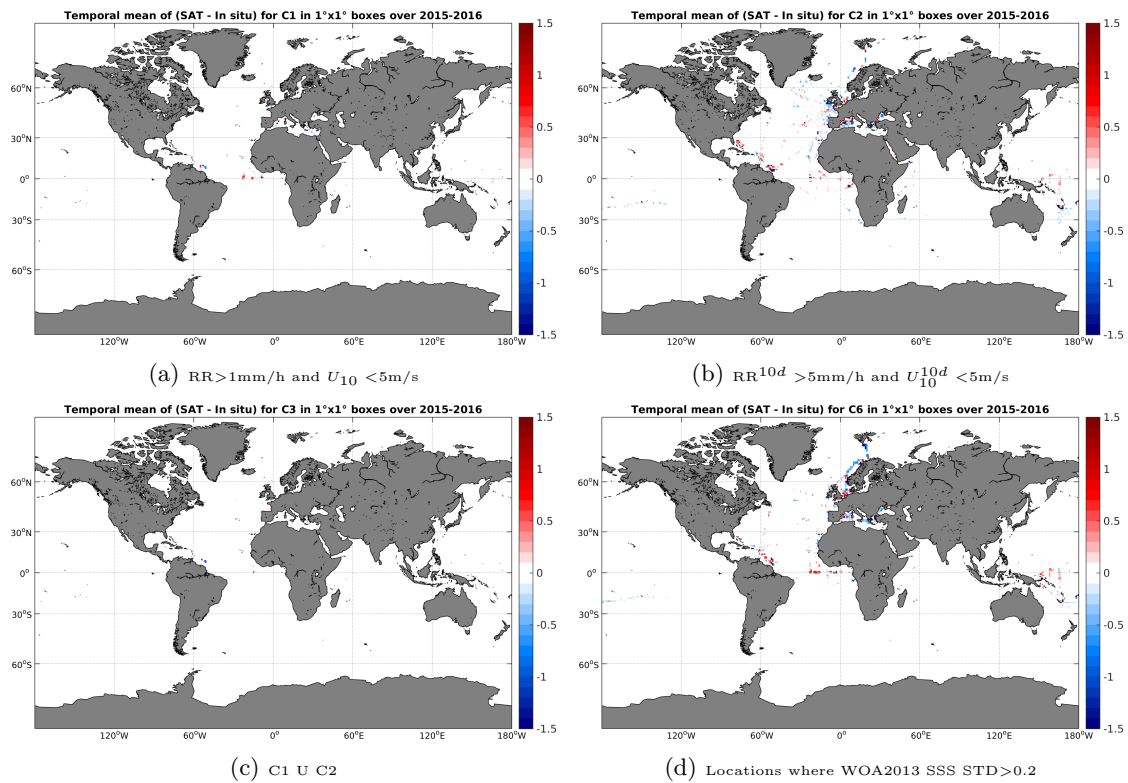
Figure 12: Temporal mean gridded over spatial boxes of size 1^\circ \times 1^\circ of \Delta SSS (SMAP-L3-RSS-V2-MONTHLY-0.25DEG-40KM - TSG-GOSUD-Research-vessel) for 4 different subdatasets corresponding to: RR > 1\text{mm/h} and U_{10} < 5\text{m/s} (a), RR^{10d} > 5\text{mm/h} and U_{10}^{10d} < 5\text{m/s} (b), C1 U C2 (c), Locations where WOA2013 SSS STD > 0.2 (d).
