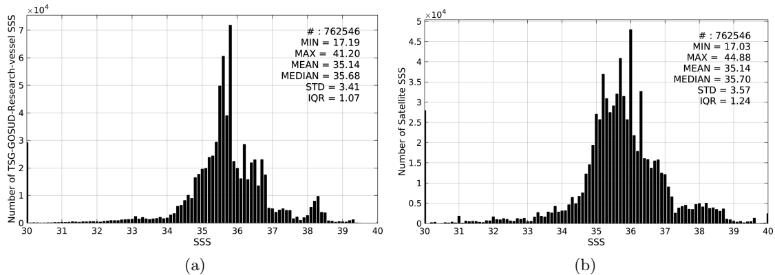
Figure 2: Histograms of SSS from TSG-GOSUD-Research-vessel (a) and SMAP-L3-RSS-V2-MONTHLY-0.25DEG-40KM (b) considering all match-up pairs per bins of 0.1 over the Global Ocean Pi-MEP region and for the full satellite product period.
