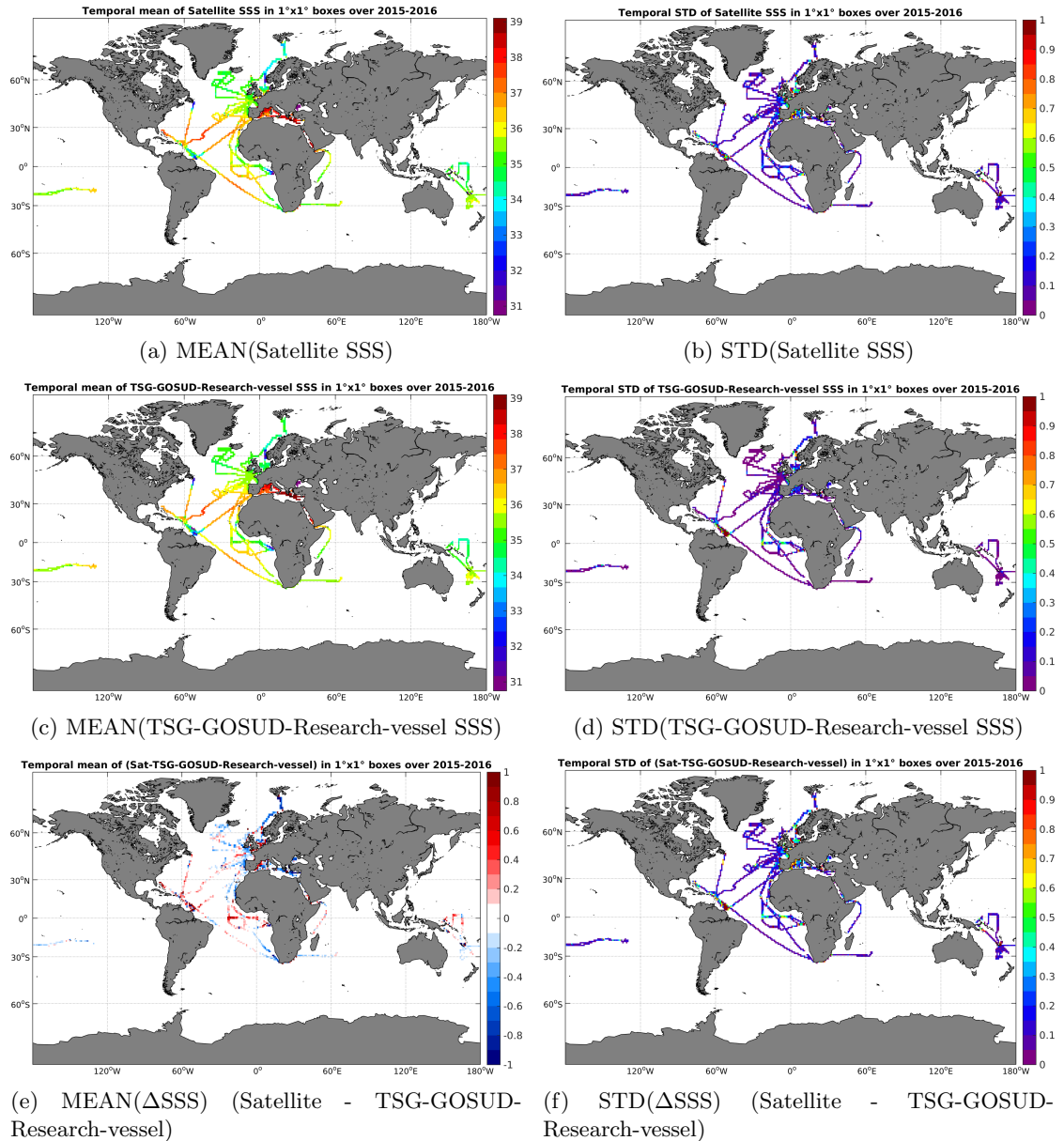
Figure 6: Temporal mean (left) and STD (right) of SSS from SMAP-L3-RSS-V2-MONTHLY-0.25DEG-40KM (top), TSG-GOSUD-Research-vessel (middle), and of \Delta SSS (Satellite - TSG-GOSUD-Research-vessel). Only match-up pairs are used to generate these maps.
