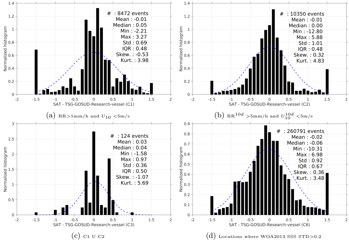
Figure 13: Normalized histogram of \Delta\text{SSS} (SMAP-L3-RSS-V2-MONTHLY-0.25DEG-40KM - TSG-GOSUD-Research-vessel) for 6 different subdatasets corresponding to: RR > 1mm/h and U_{10} < 5\text{m/s} (a), RR^{10d} > 5\text{mm/h} and U_{10}^{10d} < 5\text{m/s} (b), C1 U C2 (c), Locations where WOA2013 SSS STD > 0.2 (d).
