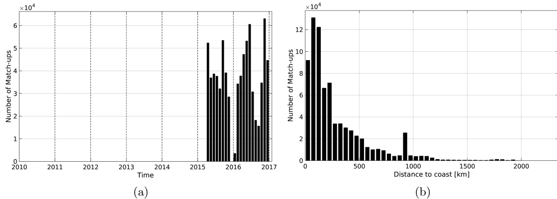
Figure 1: Number of match-ups between TSG-GOSUD-Research-vessel and SMAP-L3-RSS-V2-MONTHLY-0.25DEG-40KM SSS as a function of time (a) and as function of the distance to coast (b) over the Global Ocean Pi-MEP region and for the full satellite product period.
