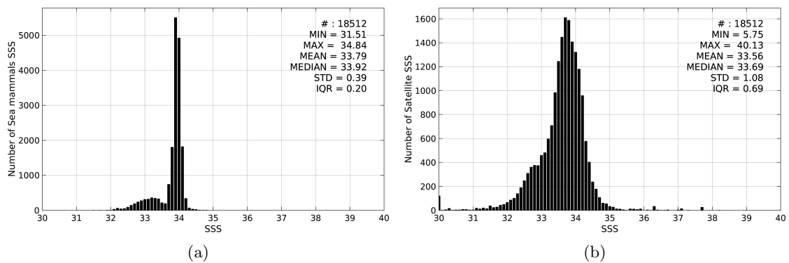
Figure 2: Histograms of SSS from Sea mammals (a) and SMAP-L3-RSS-V2-MONTHLY-0.25DEG-40KM (b) considering all match-up pairs per bins of 0.1 over the Global Ocean Pi-MEP region and for the full satellite product period.
