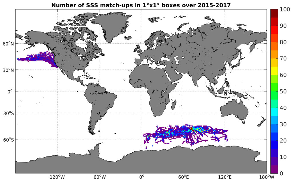
Figure 4: Number of SSS match-ups between Sea mammals SSS and the SMAP-L3-RSS-V2-MONTHLY-0.25DEG-40KM SSS product for the Global Ocean Pi-MEP region over 1^\circ \times 1^\circ boxes and for the full satellite product period.
