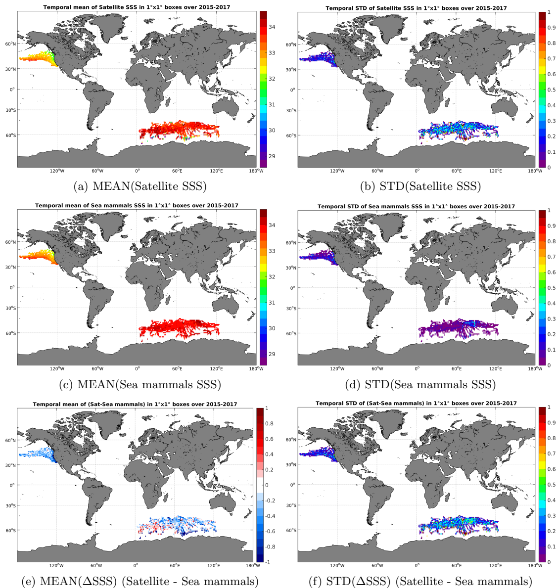
Figure 6: Temporal mean (left) and STD (right) of SSS from SMAP-L3-RSS-V2-MONTHLY-0.25DEG-40KM (top), Sea mammals (middle), and of \Delta SSS (Satellite - Sea mammals). Only match-up pairs are used to generate these maps.
