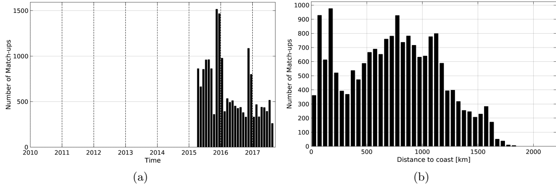
Figure 1: Number of match-ups between Sea mammals and SMAP-L3-RSS-V2-MONTHLY-0.25DEG-40KM SSS as a function of time (a) and as function of the distance to coast (b) over the Global Ocean Pi-MEP region and for the full satellite product period.
