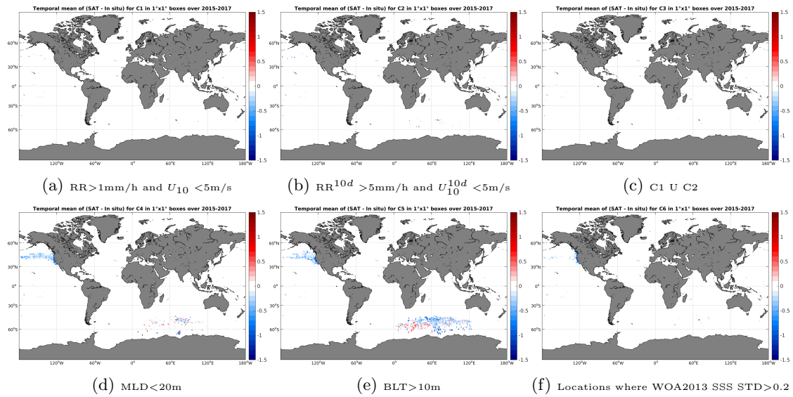
Figure 12: Temporal mean gridded over spatial boxes of size 1^\circ \times 1^\circ of \Delta SSS (SMAP-L3-RSS-V2-MONTHLY-0.25DEG-40KM - Sea mammals) for 6 different subdatasets corresponding to: RR > 1\text{mm/h} and U_{10} < 5\text{m/s} (a), RR^{10d} > 5\text{mm/h} and U_{10}^{10d} < 5\text{m/s} (b), C1 U C2 (c), MLD < 20\text{m} (d), BLT > 10\text{m} (e), Locations where WOA2013 SSS STD > 0.2 (f).
