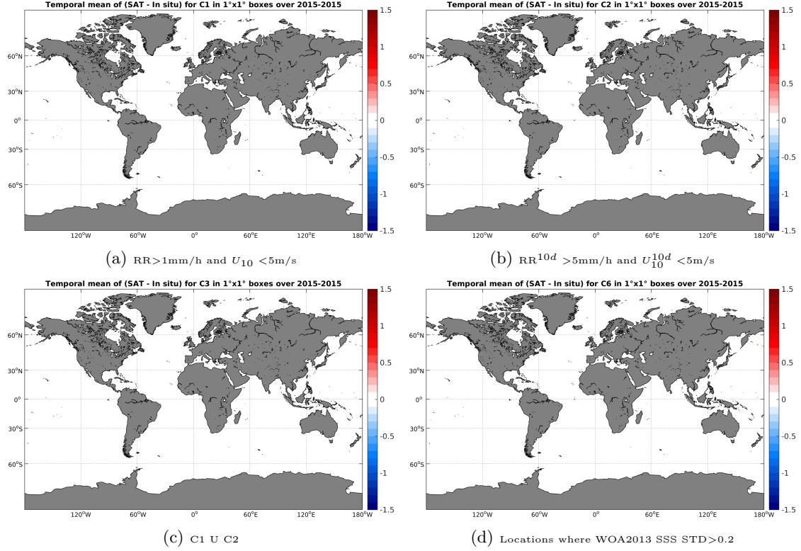
Figure 11: Temporal mean gridded over spatial boxes of size 1^\circ \times 1^\circ of \Delta SSS (SMAP-L3-RSS-V2-MONTHLY-0.25DEG-40KM - Surface drifters) for 4 different subdatasets corresponding to: RR > 1 mm/h and U_{10} < 5 m/s (a), RR^{10d} > 5 mm/h and U_{10}^{10d} < 5 m/s (b), C1 U C2 (c), Locations where WOA2013 SSS STD > 0.2 (d).
