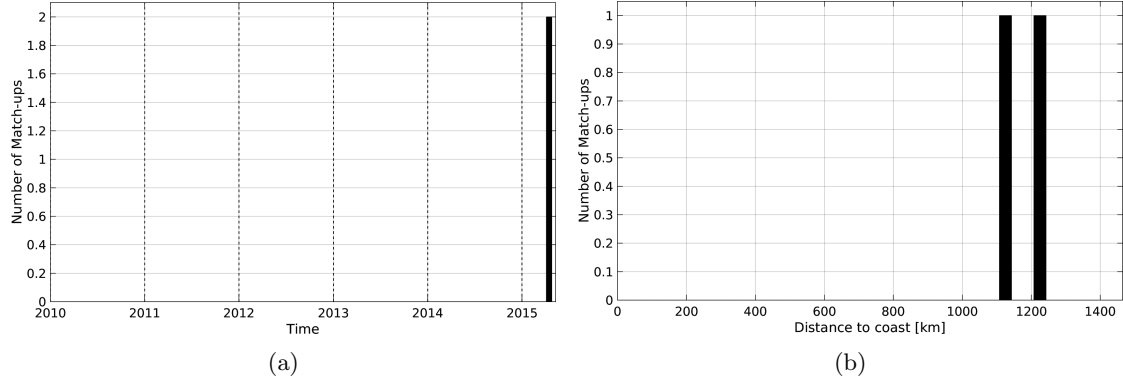
Figure 1: Number of match-ups between Surface drifters and SMAP-L3-RSS-V2-MONTHLY-0.25DEG-40KM SSS as a function of time (a) and as function of the distance to coast (b) over the Global Ocean Pi-MEP region and for the full satellite product period.
