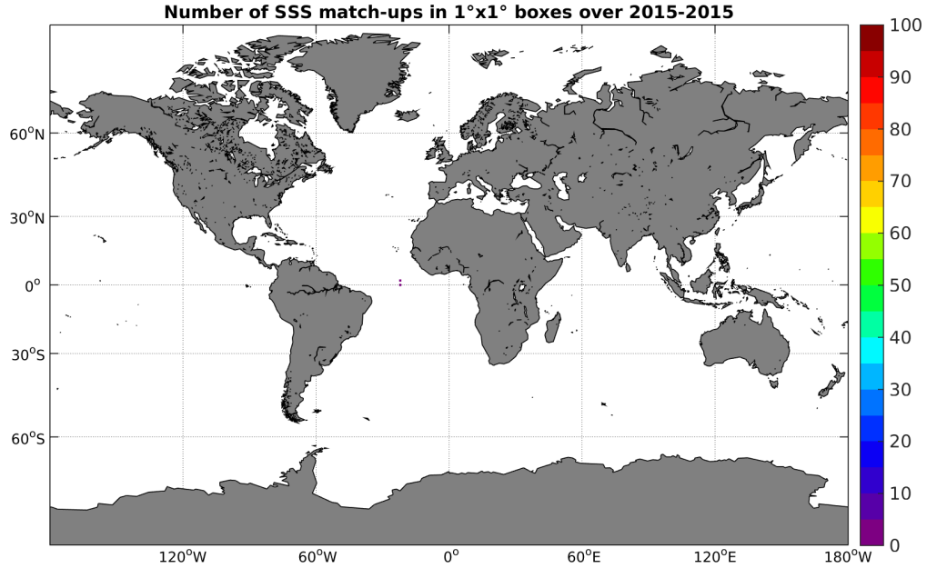
Figure 3: Number of SSS match-ups between Surface drifters SSS and the SMAP-L3-RSS-V2-MONTHLY-0.25DEG-40KM SSS product for the Global Ocean Pi-MEP region over 1°x1° boxes and for the full satellite product period.
