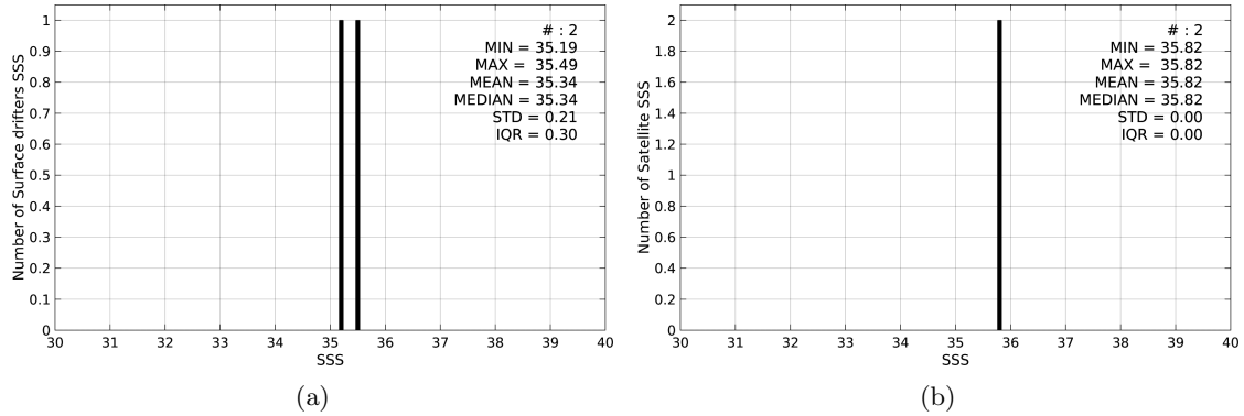
Figure 2: Histograms of SSS from Surface drifters (a) and SMAP-L3-RSS-V2-MONTHLY-0.25DEG-40KM (b) considering all match-up pairs per bins of 0.1 over the Global Ocean Pi-MEP region and for the full satellite product period.
