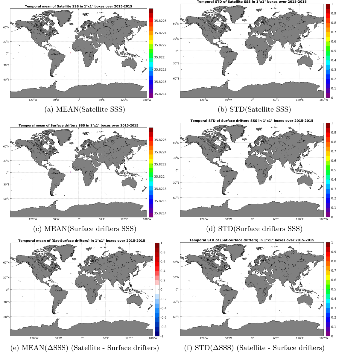
Figure 5: Temporal mean (left) and STD (right) of SSS from SMAP-L3-RSS-V2-MONTHLY-0.25DEG-40KM (top), Surface drifters (middle), and of \Delta SSS (Satellite - Surface drifters). Only match-up pairs are used to generate these maps.
