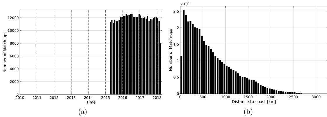
Figure 1: Number of match-ups between Argo and SMAP-L3-RSS-V2-MONTHLY-0.25DEG-40KM SSS as a function of time (a) and as function of the distance to coast (b) over the Global Ocean Pi-MEP region and for the full satellite product period.
