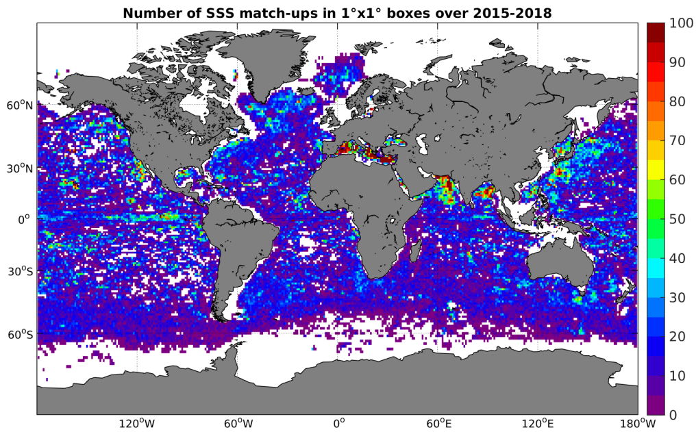
Figure 4: Number of SSS match-ups between Argo SSS and the SMAP-L3-RSS-V2-MONTHLY-0.25DEG-40KM SSS product for the Global Ocean Pi-MEP region over 1^\circ \times 1^\circ boxes and for the full satellite product period.
