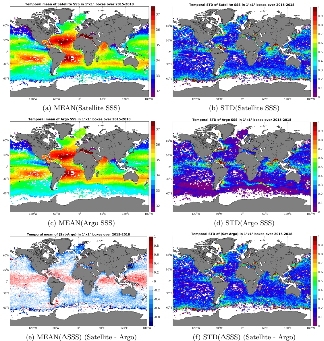
Figure 6: Temporal mean (left) and STD (right) of SSS from SMAP-L3-RSS-V2-MONTHLY-0.25DEG-40KM (top), Argo (middle), and of \Delta SSS (Satellite - Argo). Only match-up pairs are used to generate these maps.
