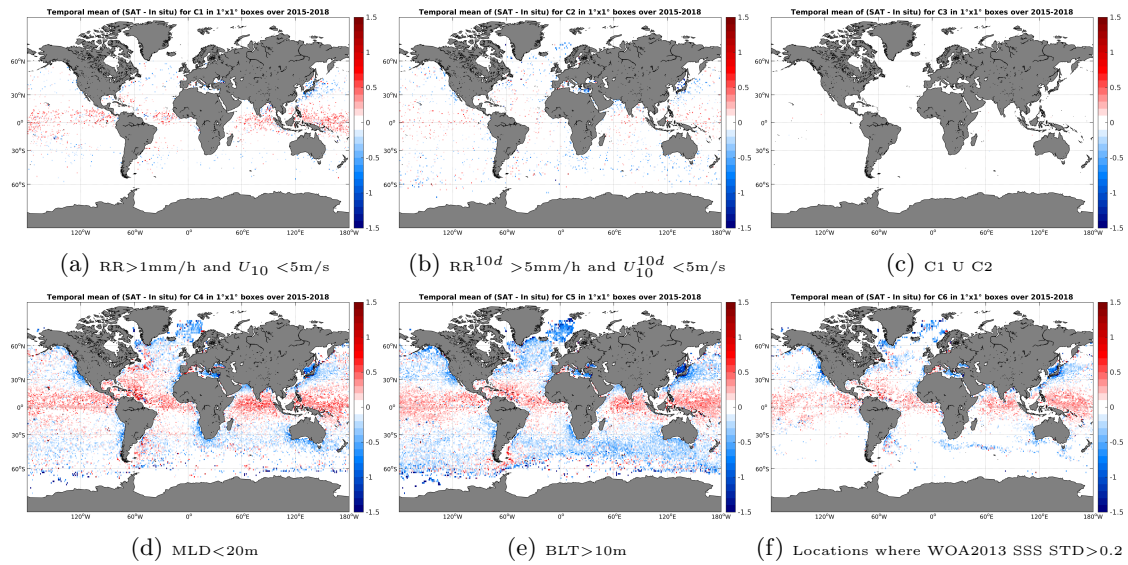
Figure 12: Temporal mean gridded over spatial boxes of size 1^\circ \times 1^\circ of \Delta SSS (SMAP-L3-RSS-V2-MONTHLY-0.25DEG-40KM - Argo) for 6 different subdatasets corresponding to: RR > 1mm/h and U_{10} < 5\text{m/s} (a), RR^{10d} > 5\text{mm/h} and U_{10}^{10d} < 5\text{m/s} (b), C1 U C2 (c), MLD < 20\text{m} (d), BLT > 10\text{m} (e), Locations where WOA2013 SSS STD > 0.2 (f).
