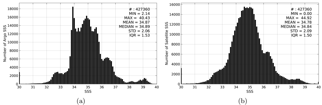
Figure 2: Histograms of SSS from Argo (a) and SMAP-L3-RSS-V2-MONTHLY-0.25DEG-40KM (b) considering all match-up pairs per bins of 0.1 over the Global Ocean Pi-MEP region and for the full satellite product period.
