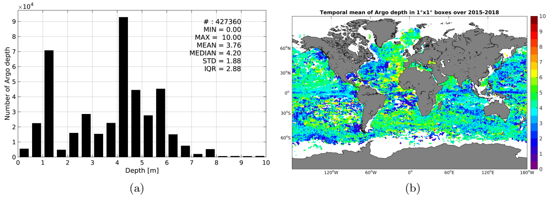
Figure 3: Histograms of the depth of the upper level SSS measurements from Argo in the Match-up DataBase for the Global Ocean Pi-MEP region (a) and temporal mean spatial distribution of pressure of the in situ SSS data over 1^\circ \times 1^\circ boxes and for the full satellite product period (b).
