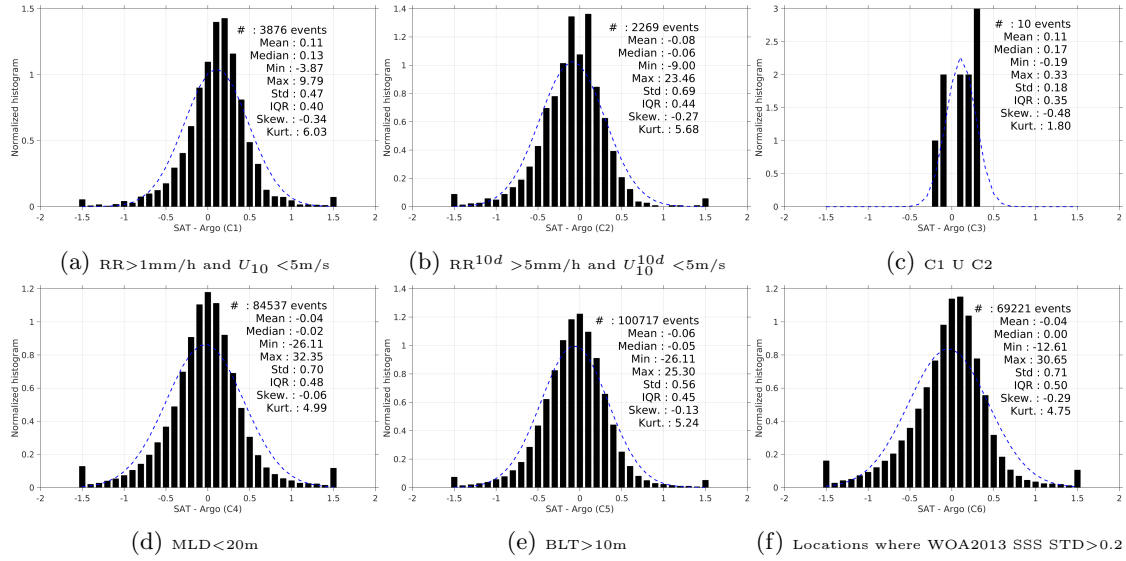
Figure 13: Normalized histogram of \Delta SSS (SMAP-L3-RSS-V2-MONTHLY-0.25DEG-40KM - Argo) for 6 different subdatasets corresponding to: RR>1mm/h and U_{10} <5m/s (a), RR 10d >5mm/h and U_{10}^{10d} <5m/s (b), C1 U C2 (c),MLD<20m (d),BLT>10m (e),Locations where WOA2013 SSS STD>0.2 (f).
