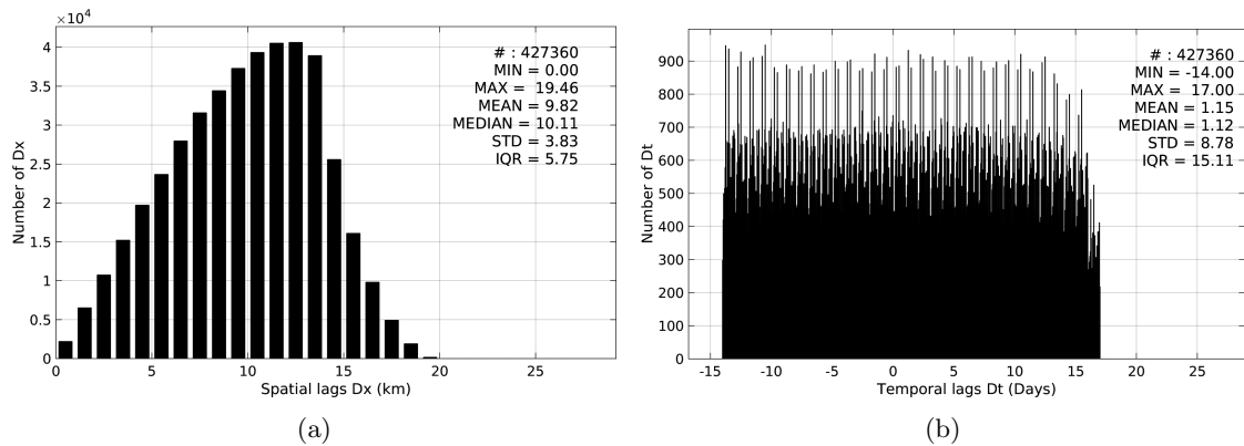
Figure 5: Histograms of the spatial (a) and temporal (b) lags between the time of the Argo measurements and the date of the corresponding SMAP-L3-RSS-V2-MONTHLY-0.25DEG-40KM SSS product.
