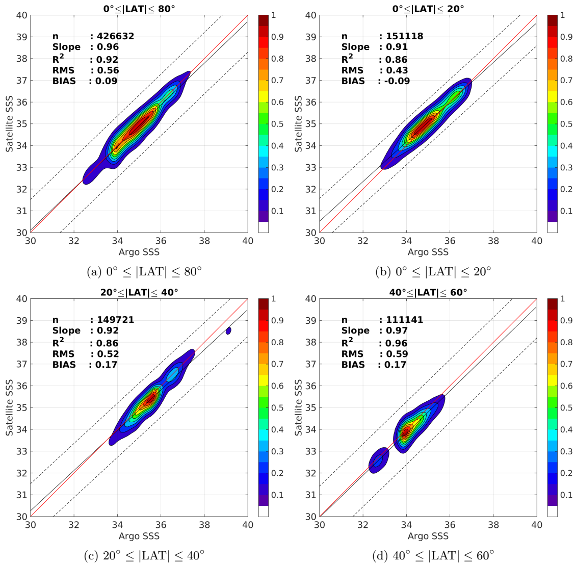
Figure 9: Contour maps of the concentration of SMAP-L3-RSS-V2-MONTHLY-0.25DEG-40KM SSS (y-axis) versus Argo SSS (x-axis) at match-up pairs for different latitude bands. For each plot, the red line shows x=y . The black thin and dashed lines indicate a linear fit through the data cloud and the \pm 95\% confidence levels, respectively. The number match-up pairs n , the slope and R^2 coefficient of the linear fit, the root mean square (RMS) and the mean bias between satellite and in situ data are indicated for each latitude band in each plots.
