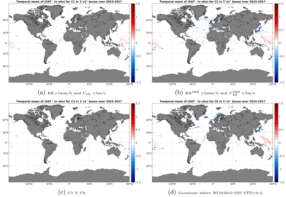
Figure 12: Temporal mean gridded over spatial boxes of size 1^\circ \times 1^\circ of \Delta SSS (SMAP-L3-RSS-V2-MONTHLY-70KM - TSG-LEGOS-DM) for 4 different subdatasets corresponding to: RR > 1\text{mm/h} and U_{10} < 5\text{m/s} (a), RR^{10d} > 5\text{mm/h} and U_{10}^{10d} < 5\text{m/s} (b), C1 U C2 (c), Locations where WOA2013 SSS STD > 0.2 (d).
