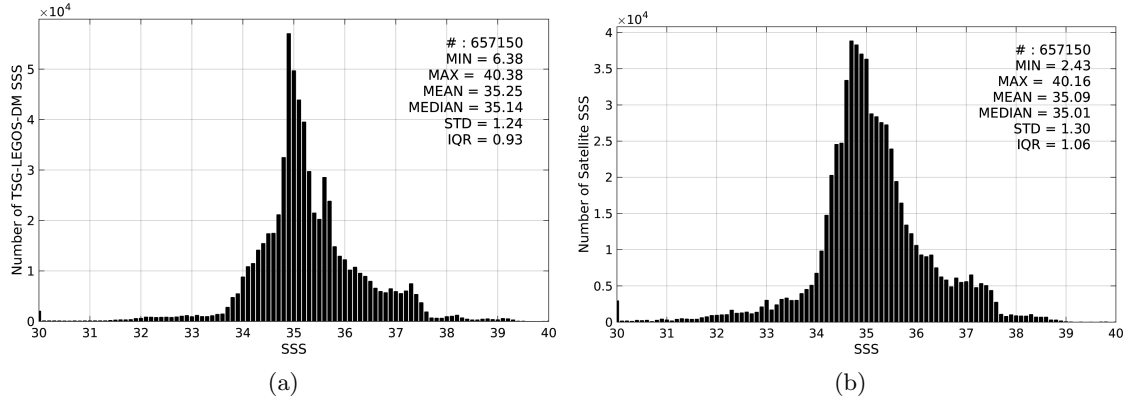
Figure 2: Histograms of SSS from TSG-LEGOS-DM (a) and SMAP-L3-RSS-V2-MONTHLY-70KM (b) considering all match-up pairs per bins of 0.1 over the Global Ocean Pi-MEP region and for the full satellite product period.
