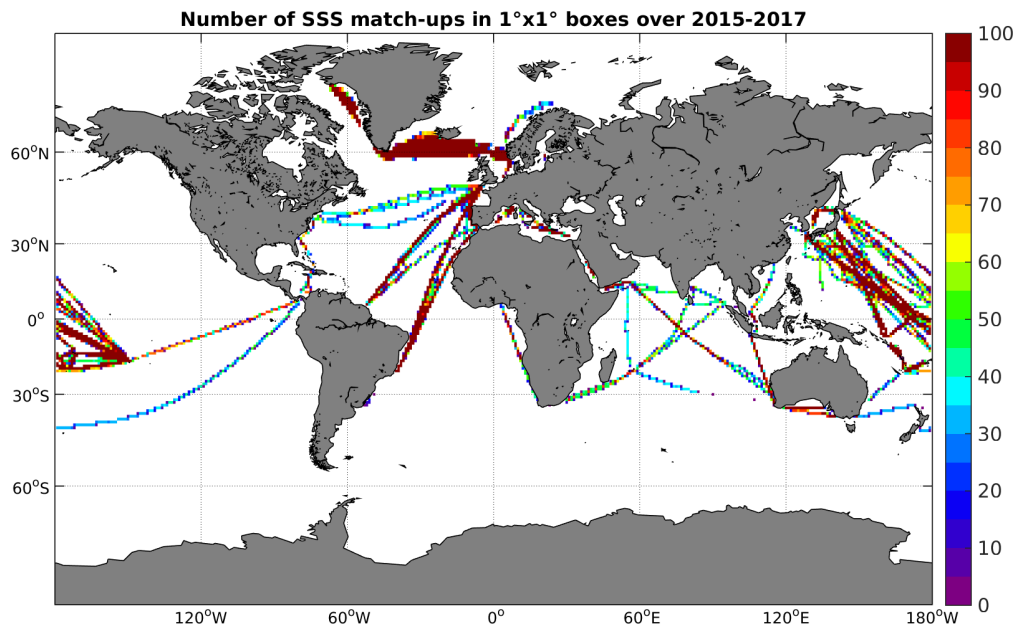
Figure 4: Number of SSS match-ups between TSG-LEGOS-DM SSS and the SMAP-L3-RSS-V2-MONTHLY-70KM SSS product for the Global Ocean Pi-MEP region over 1^\circ \times 1^\circ boxes and for the full satellite product period.
