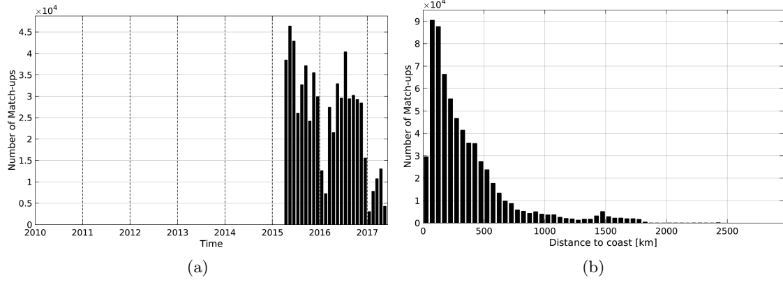
Figure 1: Number of match-ups between TSG-LEGOS-DM and SMAP-L3-RSS-V2-MONTHLY-70KM SSS as a function of time (a) and as function of the distance to coast (b) over the Global Ocean Pi-MEP region and for the full satellite product period.
