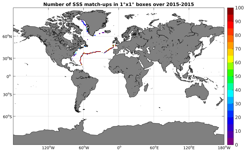
Figure 4: Number of SSS match-ups between TSG-GOSUD-Sailing-ship SSS and the SMAP-L3-RSS-V2-MONTHLY-70KM SSS product for the Global Ocean Pi-MEP region over 1°x1° boxes and for the full satellite product period.
