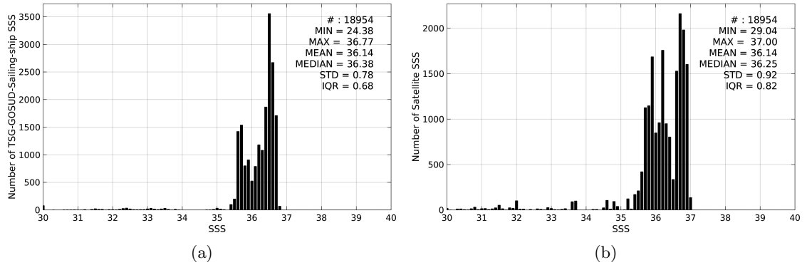
Figure 2: Histograms of SSS from TSG-GOSUD-Sailing-ship (a) and SMAP-L3-RSS-V2-MONTHLY-70KM (b) considering all match-up pairs per bins of 0.1 over the Global Ocean Pi-MEP region and for the full satellite product period.
