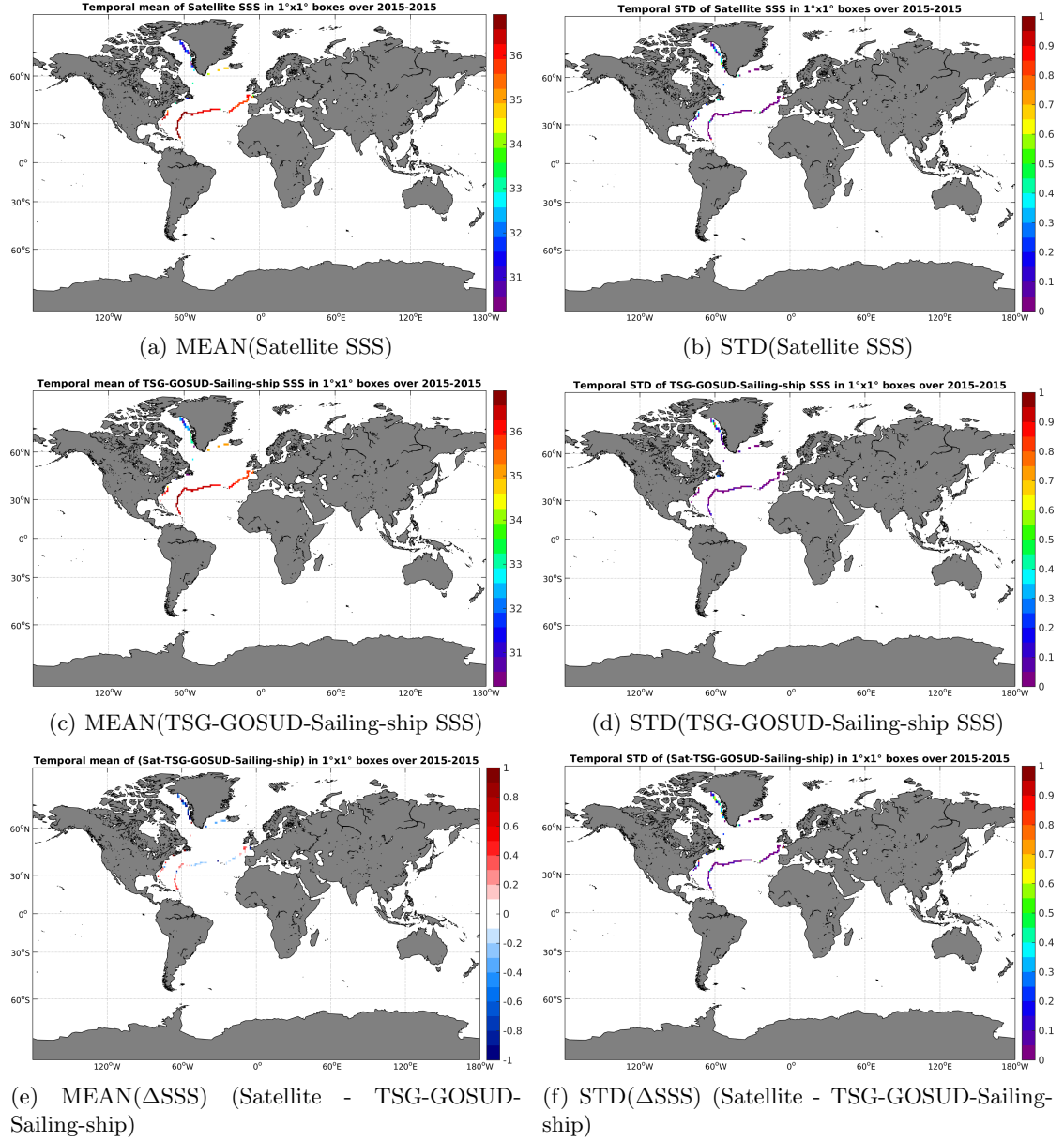
Figure 6: Temporal mean (left) and STD (right) of SSS from SMAP-L3-RSS-V2-MONTHLY-70KM (top), TSG-GOSUD-Sailing-ship (middle), and of \Delta SSS (Satellite - TSG-GOSUD-Sailing-ship). Only match-up pairs are used to generate these maps.
