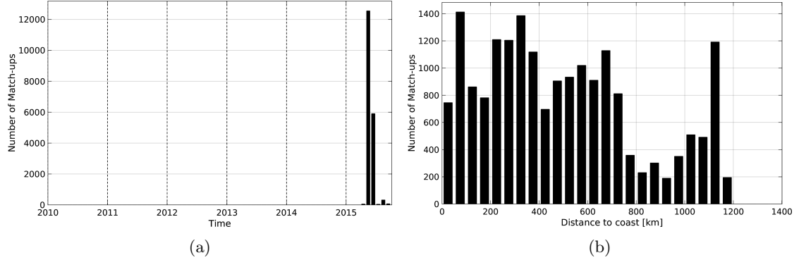
Figure 1: Number of match-ups between TSG-GOSUD-Sailing-ship and SMAP-L3-RSS-V2-MONTHLY-70KM SSS as a function of time (a) and as function of the distance to coast (b) over the Global Ocean Pi-MEP region and for the full satellite product period.
