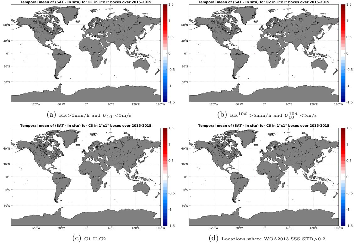
Figure 11: Temporal mean gridded over spatial boxes of size 1^\circ \times 1^\circ of \Delta SSS (SMAP-L3-RSS-V2-MONTHLY-70KM - Surface drifters) for 4 different subdatasets corresponding to: RR > 1\text{mm/h} and U_{10} < 5\text{m/s} (a), RR^{10d} > 5\text{mm/h} and U_{10}^{10d} < 5\text{m/s} (b), C1 U C2 (c), Locations where WOA2013 SSS STD > 0.2 (d).
