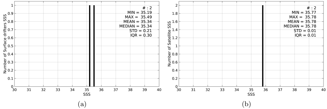
Figure 2: Histograms of SSS from Surface drifters (a) and SMAP-L3-RSS-V2-MONTHLY-70KM (b) considering all match-up pairs per bins of 0.1 over the Global Ocean Pi-MEP region and for the full satellite product period.
