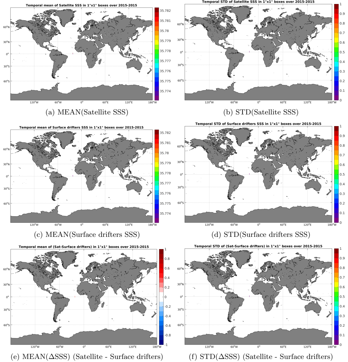
Figure 5: Temporal mean (left) and STD (right) of SSS from SMAP-L3-RSS-V2-MONTHLY-70KM (top), Surface drifters (middle), and of \Delta SSS (Satellite - Surface drifters). Only match-up pairs are used to generate these maps.
