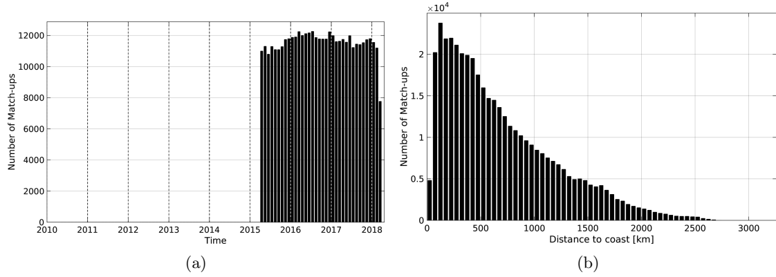
Figure 1: Number of match-ups between Argo and SMAP-L3-RSS-V2-MONTHLY-70KM SSS as a function of time (a) and as function of the distance to coast (b) over the Global Ocean Pi-MEP region and for the full satellite product period.
