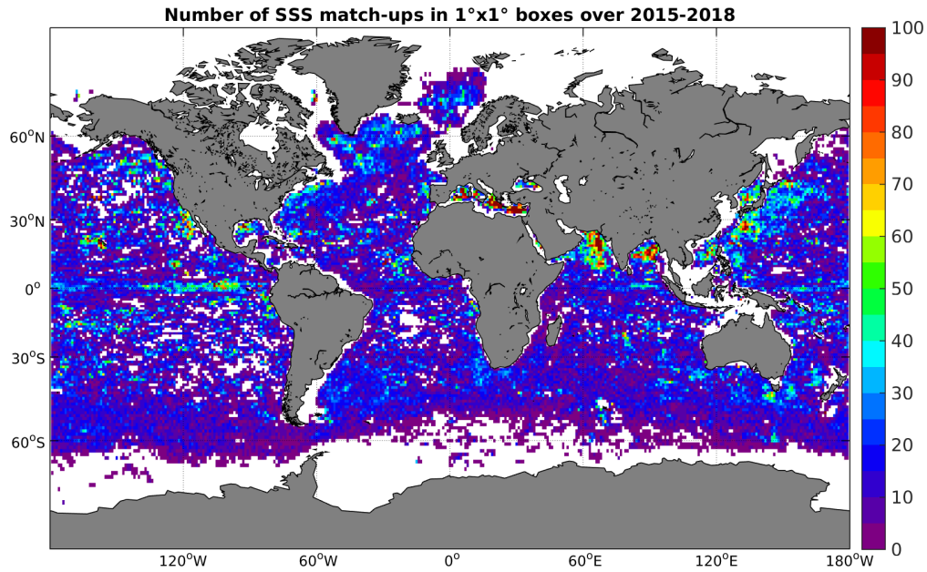
Figure 4: Number of SSS match-ups between Argo SSS and the SMAP-L3-RSS-V2-MONTHLY-70KM SSS product for the Global Ocean Pi-MEP region over 1^\circ \times 1^\circ boxes and for the full satellite product period.
