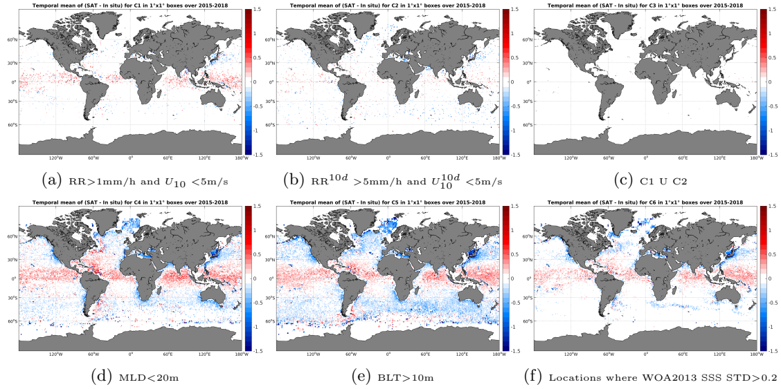
Figure 12: Temporal mean gridded over spatial boxes of size 1^\circ \times 1^\circ of \Delta SSS (SMAP-L3-RSS-V2-MONTHLY-70KM - Argo) for 6 different subdatasets corresponding to: RR > 1\text{mm/h} and U_{10} < 5\text{m/s} (a), RR^{10d} > 5\text{mm/h} and U_{10}^{10d} < 5\text{m/s} (b), C1 U C2 (c), MLD < 20\text{m} (d), BLT > 10\text{m} (e), Locations where WOA2013 SSS STD > 0.2 (f).
