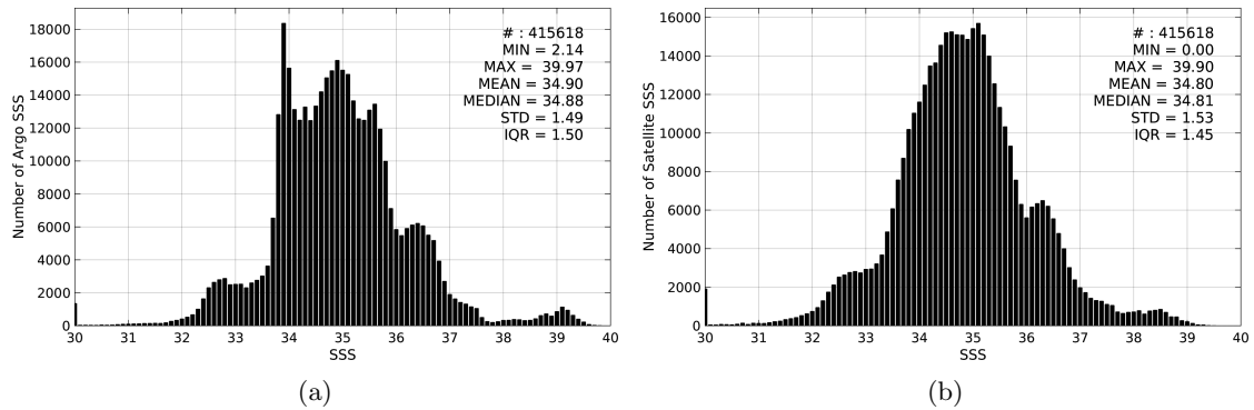
Figure 2: Histograms of SSS from Argo (a) and SMAP-L3-RSS-V2-MONTHLY-70KM (b) considering all match-up pairs per bins of 0.1 over the Global Ocean Pi-MEP region and for the full satellite product period.
