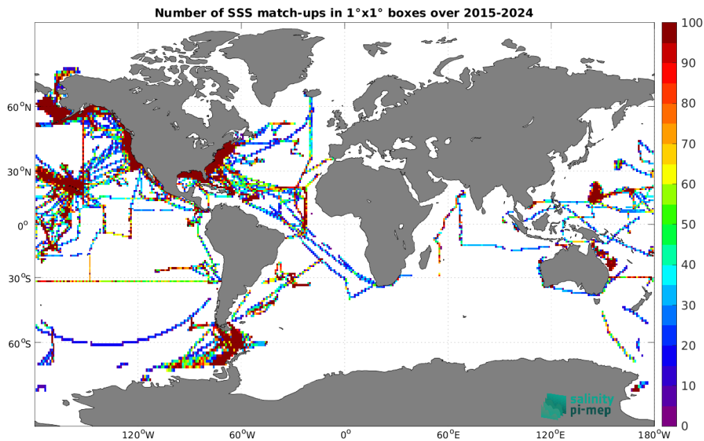
Figure 5: Number of SSS match-ups between TSG (SAMOS) SSS and the SMAP SSS L3 v5.0 - 8-Day running (JPL) SSS product for the Global Ocean Pi-MEP region over 1^\circ \times 1^\circ boxes and for the full satellite product period.
