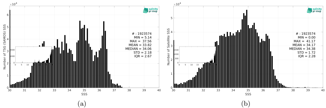
Figure 3: Histograms of SSS from TSG (SAMOS) (a) and SMAP SSS L3 v5.0 - 8-Day running (JPL) (b) considering all match-up pairs per bins of 0.1 over the Global Ocean Pi-MEP region and for the full satellite product period.
