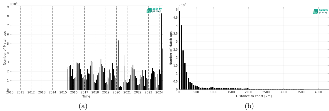
Figure 2: Number of match-ups between TSG (SAMOS) and SMAP SSS L3 v5.0 - 8-Day running (JPL) SSS as a function of time (a) and as function of the distance to coast (b) over the Global Ocean Pi-MEP region and for the full satellite product period.
