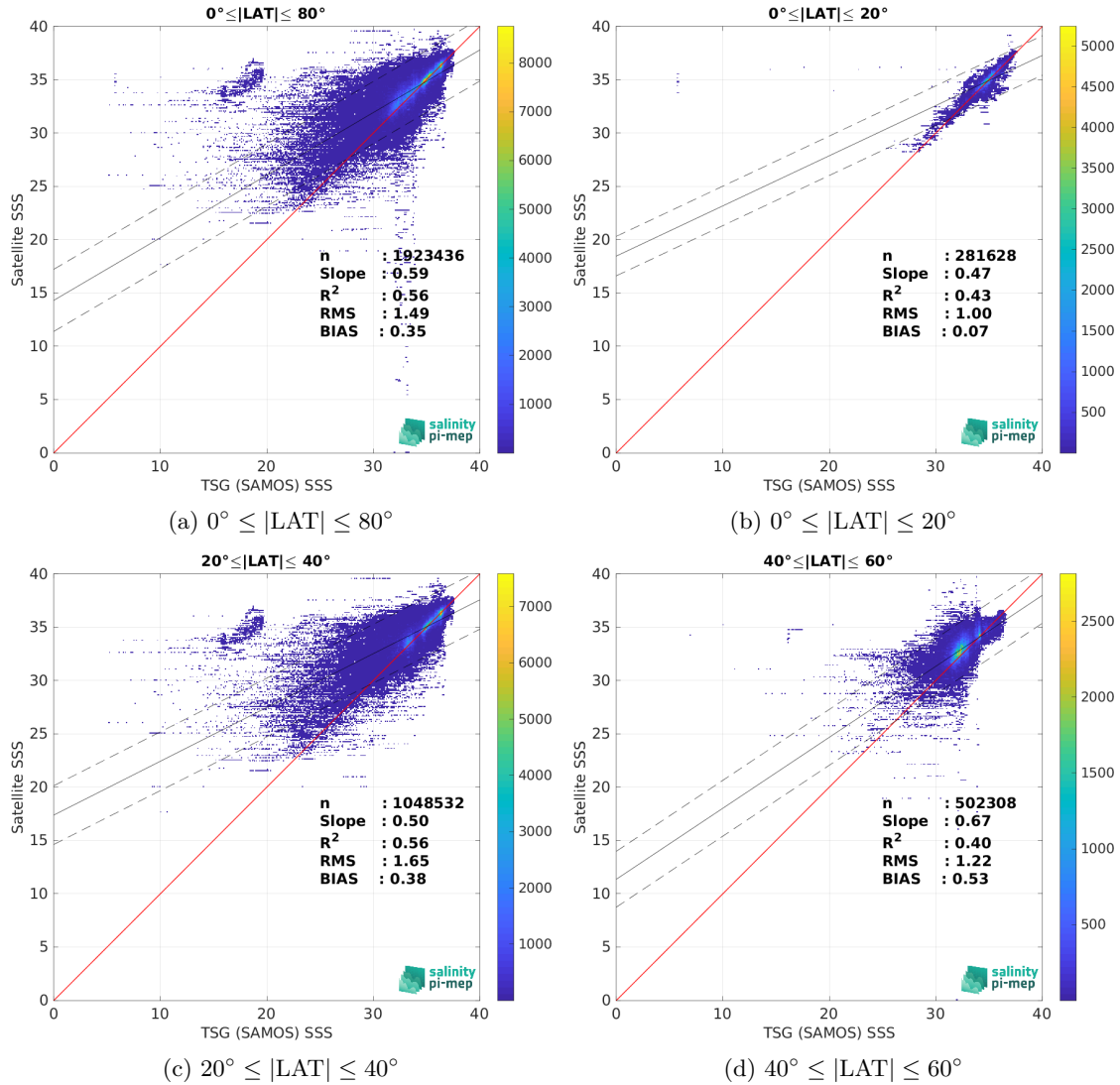
Figure 10: Contour maps of the concentration of SMAP SSS L3 v5.0 - 8-Day running (JPL) SSS (y-axis) versus TSG (SAMOS) SSS (x-axis) at match-up pairs for different latitude bands. For each plot, the red line shows x=y . The black thin and dashed lines indicate a linear fit through the data cloud and the \pm 95\% confidence levels, respectively. The number match-up pairs n , the slope and R^2 coefficient of the linear fit, the root mean square (RMS) and the mean bias between satellite and in situ data are indicated for each latitude band in each plots.
