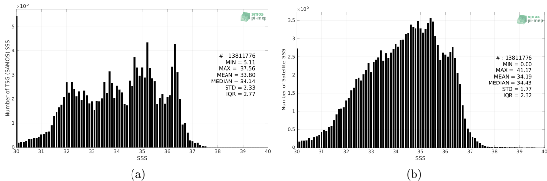
Figure 2: Histograms of SSS from TSG (SAMOS) (a) and SMAP SSS L3 v5.0 - 8-Day running (JPL) (b) considering all match-up pairs per bins of 0.1 over the Global Ocean Pi-MEP region and for the full satellite product period.
