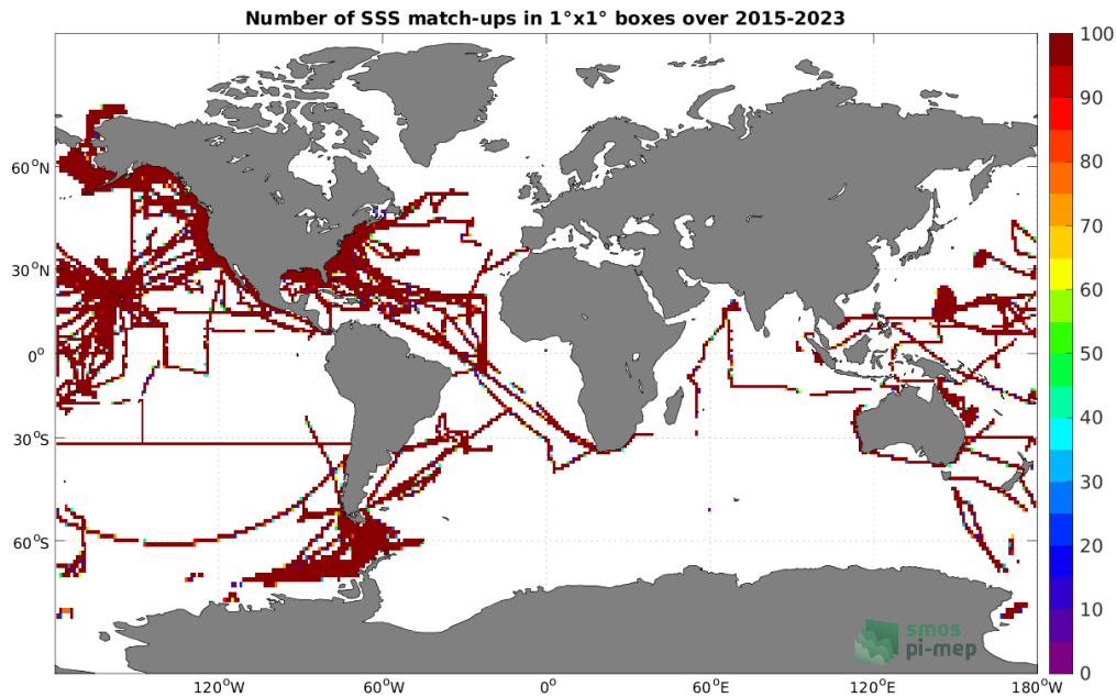
Figure 4: Number of SSS match-ups between TSG (SAMOS) SSS and the SMAP SSS L3 v5.0 - 8-Day running (JPL) SSS product for the Global Ocean Pi-MEP region over 1^\circ \times 1^\circ boxes and for the full satellite product period.
