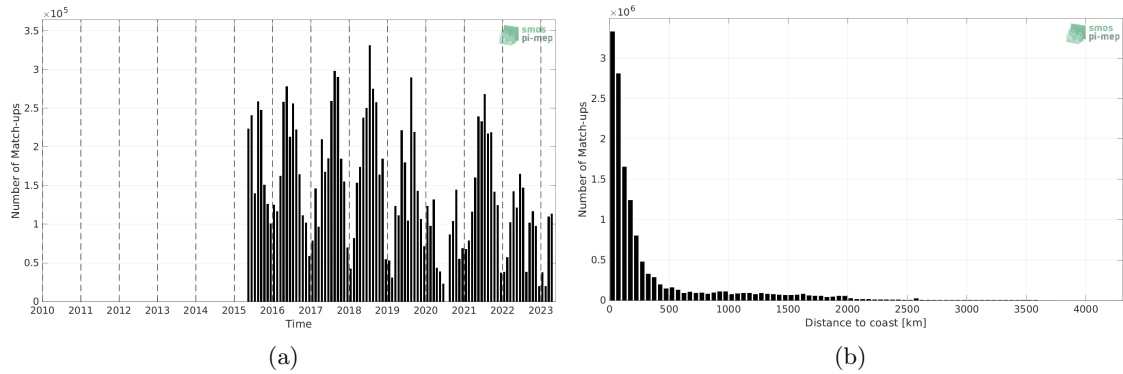
Figure 1: Number of match-ups between TSG (SAMOS) and SMAP SSS L3 v5.0 - 8-Day running (JPL) SSS as a function of time (a) and as function of the distance to coast (b) over the Global Ocean Pi-MEP region and for the full satellite product period.
