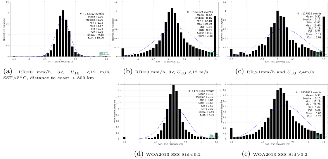
Figure 13: Normalized histogram of \Delta\text{SSS} (SMAP SSS L3 v5.0 - 8-Day running (JPL) - TSG (SAMOS)) for 5 different subdatasets corresponding to: RR=0 mm/h, 3 < U_{10} < 12 m/s, SST>5°C, distance to coast > 800 km (a), RR=0 mm/h, 3 < U_{10} < 12 m/s (b), RR>1mm/h and U_{10} < 4 m/s (c), WOA2013 SSS Std<0.2 (d), WOA2013 SSS Std>0.2 (e).
