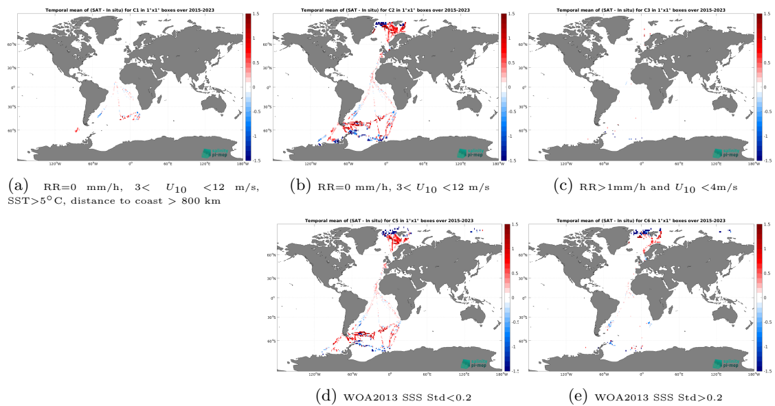
Figure 14: Temporal mean gridded over spatial boxes of size 1^\circ \times 1^\circ of \Delta SSS (SMAP SSS L3 v5.0 - 8-Day running (JPL) - TSG (Polarstern)) for 5 different subdatasets corresponding to: RR=0 mm/h, 3 < U_{10} < 12 m/s, SST > 5^\circ\text{C} , distance to coast > 800 km (a), RR=0 mm/h, 3 < U_{10} < 12 m/s (b), RR > 1 mm/h and U_{10} < 4 m/s (c), WOA2013 SSS Std < 0.2 (d), WOA2013 SSS Std > 0.2 (e).
