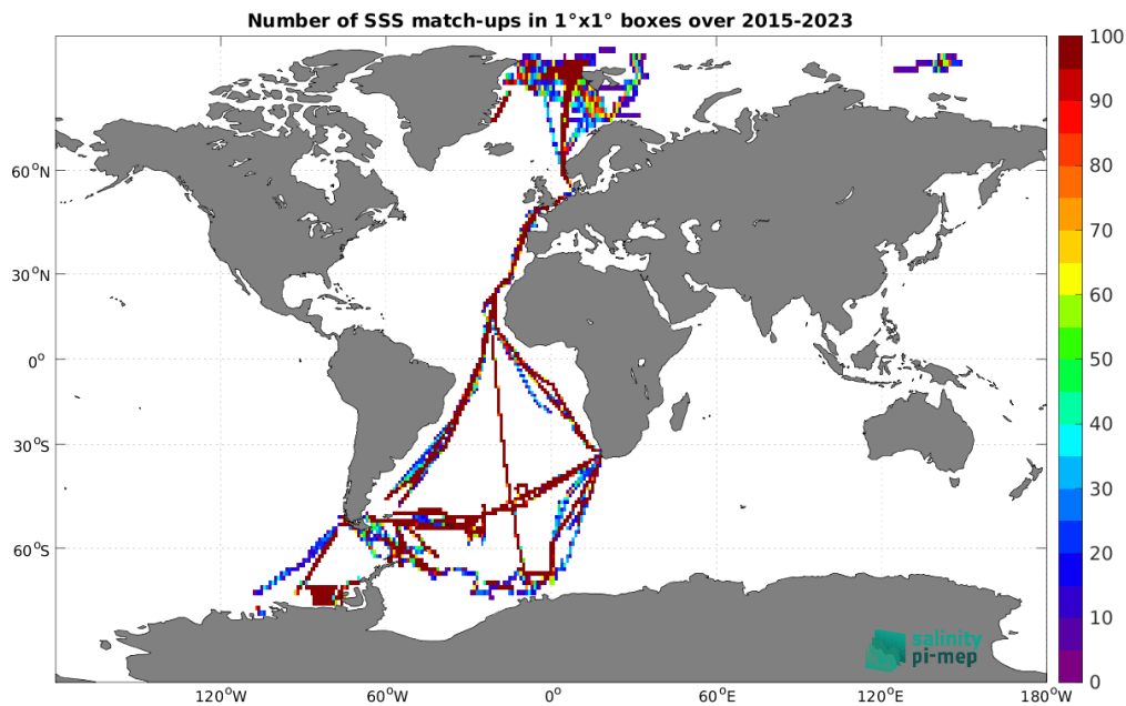
Figure 5: Number of SSS match-ups between TSG (Polarstern) SSS and the SMAP SSS L3 v5.0 - 8-Day running (JPL) SSS product for the Global Ocean Pi-MEP region over 1^\circ \times 1^\circ boxes and for the full satellite product period.
