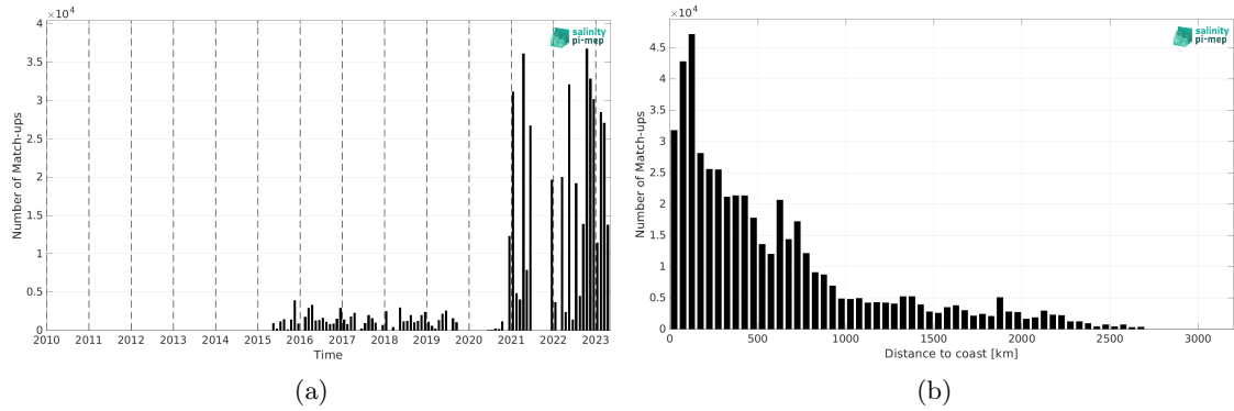
Figure 2: Number of match-ups between TSG (Polarstern) and SMAP SSS L3 v5.0 - 8-Day running (JPL) SSS as a function of time (a) and as function of the distance to coast (b) over the Global Ocean Pi-MEP region and for the full satellite product period.
