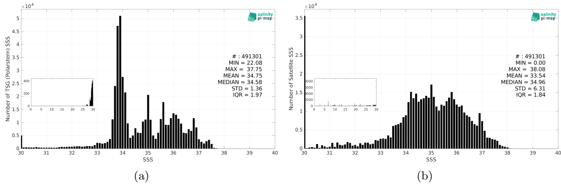
Figure 3: Histograms of SSS from TSG (Polarstern) (a) and SMAP SSS L3 v5.0 - 8-Day running (JPL) (b) considering all match-up pairs per bins of 0.1 over the Global Ocean Pi-MEP region and for the full satellite product period.
