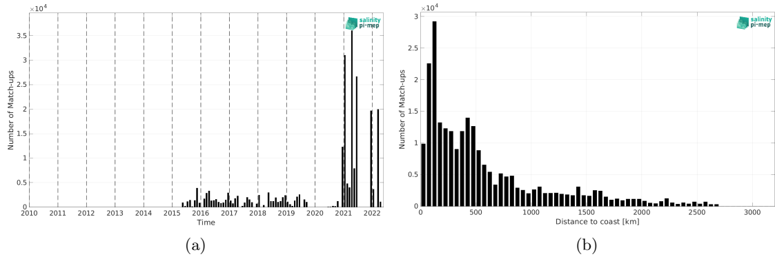
Figure 1: Number of match-ups between TSG (Polarstern) and SMAP SSS L3 v5.0 - 8-Day running (JPL) SSS as a function of time (a) and as function of the distance to coast (b) over the Global Ocean Pi-MEP region and for the full satellite product period.
