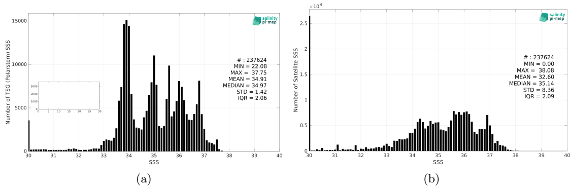
Figure 2: Histograms of SSS from TSG (Polarstern) (a) and SMAP SSS L3 v5.0 - 8-Day running (JPL) (b) considering all match-up pairs per bins of 0.1 over the Global Ocean Pi-MEP region and for the full satellite product period.
