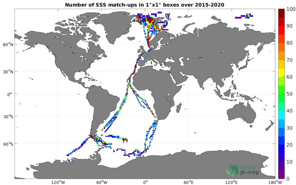
Figure 4: Number of SSS match-ups between TSG (Polarstern) SSS and the SMAP SSS L3 v5.0 - 8-Day running (JPL) SSS product for the Global Ocean Pi-MEP region over 1^\circ \times 1^\circ boxes and for the full satellite product period.
