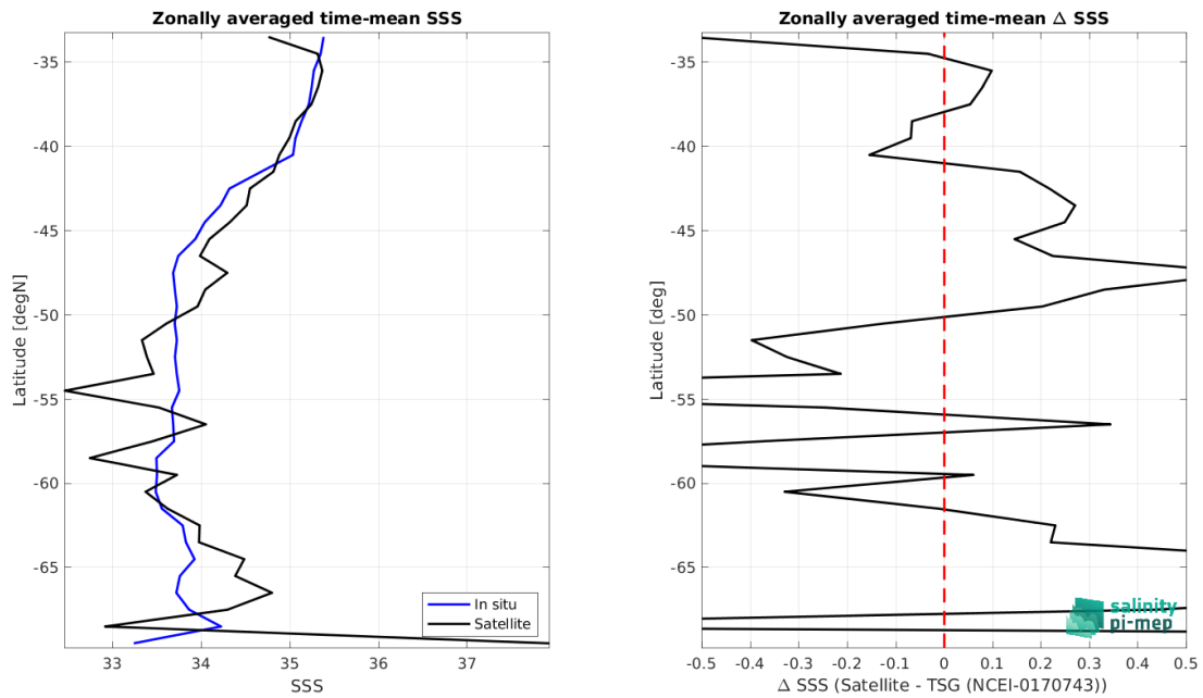
Figure 9: Left panel: Zonal mean SSS from SMAP SSS L3 v5.0 - 8-Day running (JPL) satellite product (black) and from TSG (NCEI-0170743) (blue). Right panel: Zonal mean of \Delta SSS (Satellite - TSG (NCEI-0170743)) for all the collected Pi-MEP match-up pairs estimated over the full satellite product period.
