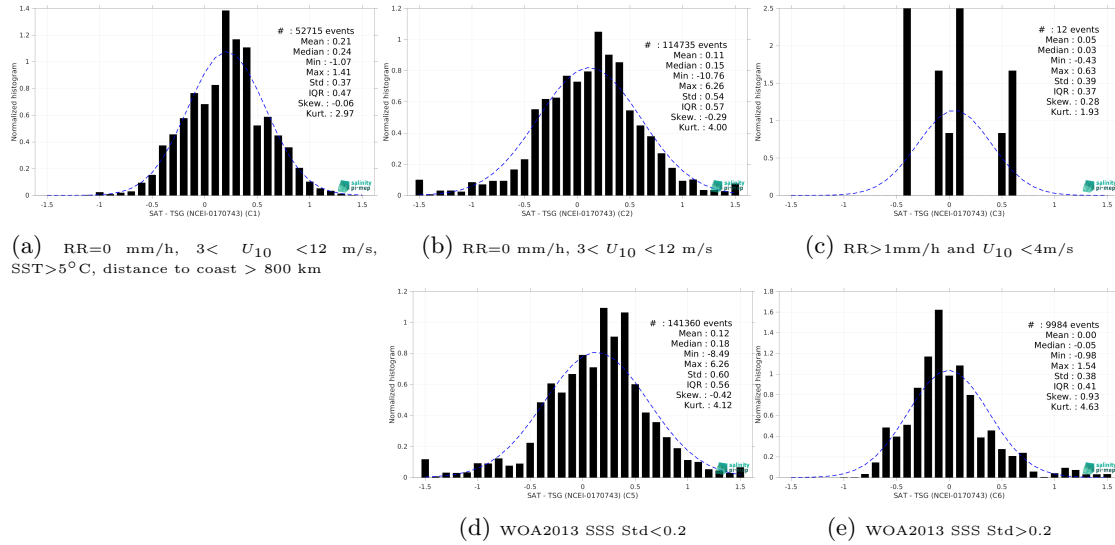
Figure 15: Normalized histogram of \Delta SSS (SMAP SSS L3 v5.0 - 8-Day running (JPL) - TSG (NCEI-0170743)) for 5 different subdatasets corresponding to: RR=0 mm/h, 3 < U_{10} < 12 m/s, SST > 5°C, distance to coast > 800 km (a), RR=0 mm/h, 3 < U_{10} < 12 m/s (b), RR > 1mm/h and U_{10} < 4 m/s (c), WOA2013 SSS Std < 0.2 (d), WOA2013 SSS Std > 0.2 (e).
