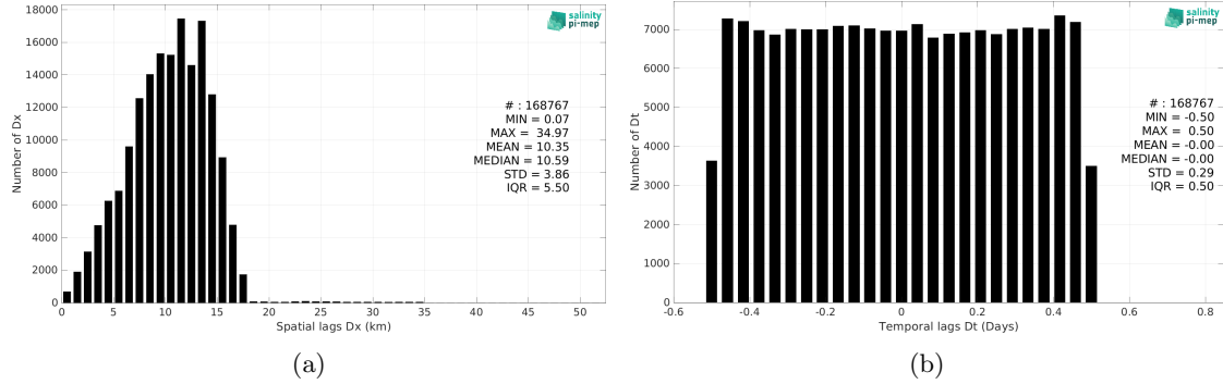
Figure 6: Histograms of the spatial (a) and temporal (b) lags between the location/time of the TSG (NCEI-0170743) measurement and the date of the corresponding SMAP SSS L3 v5.0 - 8-Day running (JPL) SSS pixel.
