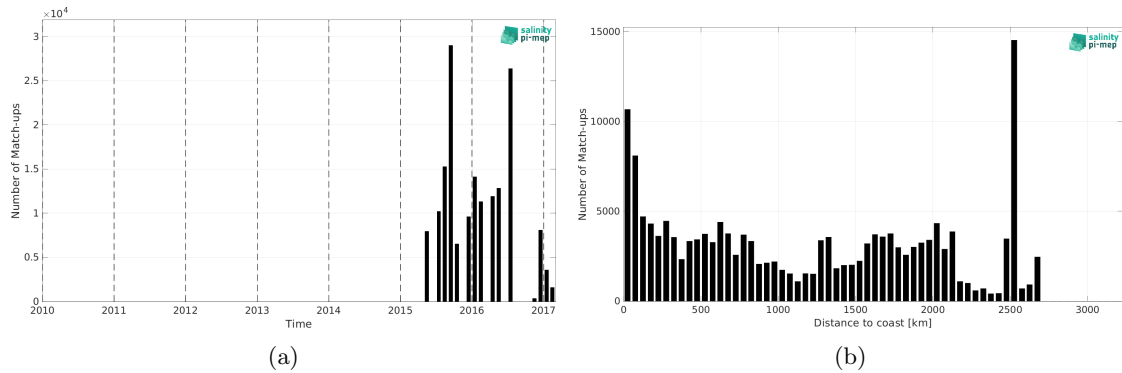
Figure 2: Number of match-ups between TSG (NCEI-0170743) and SMAP SSS L3 v5.0 - 8-Day running (JPL) SSS as a function of time (a) and as function of the distance to coast (b) over the Global Ocean Pi-MEP region and for the full satellite product period.
