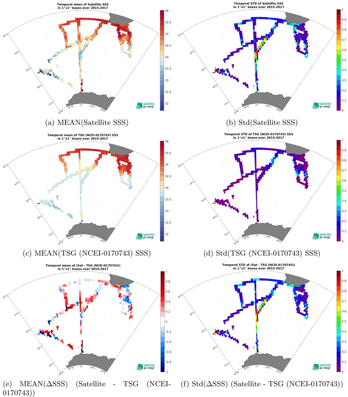
Figure 7: Temporal mean (left) and Std (right) of SSS from SMAP SSS L3 v5.0 - 8-Day running (JPL) (top), TSG (NCEI-0170743) (middle), and of \Delta SSS (Satellite - TSG (NCEI-0170743)). Only match-up pairs are used to generate these maps.
