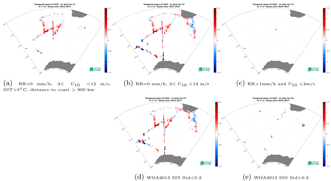
Figure 14: Temporal mean gridded over spatial boxes of size 1^\circ \times 1^\circ of \Delta SSS (SMAP SSS L3 v5.0 - 8-Day running (JPL) - TSG (NCEI-0170743)) for 5 different subdatasets corresponding to:RR=0 mm/h, 3 < U_{10} < 12 m/s, SST >5^\circ\text{C} , distance to coast > 800 km (a), RR=0 mm/h, 3 < U_{10} < 12 m/s (b), RR >1 mm/h and U_{10} < 4 m/s (c), WOA2013 SSS Std <0.2 (d), WOA2013 SSS Std >0.2 (e).
