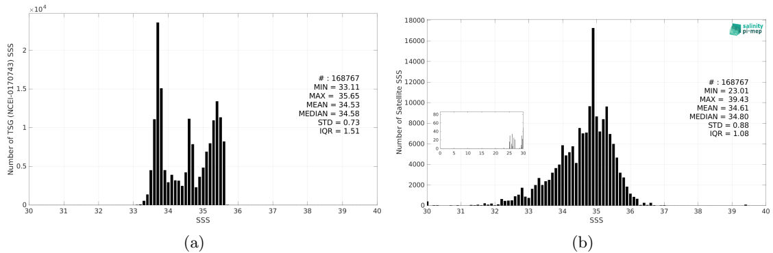
Figure 3: Histograms of SSS from TSG (NCEI-0170743) (a) and SMAP SSS L3 v5.0 - 8-Day running (JPL) (b) considering all match-up pairs per bins of 0.1 over the Global Ocean Pi-MEP region and for the full satellite product period.
