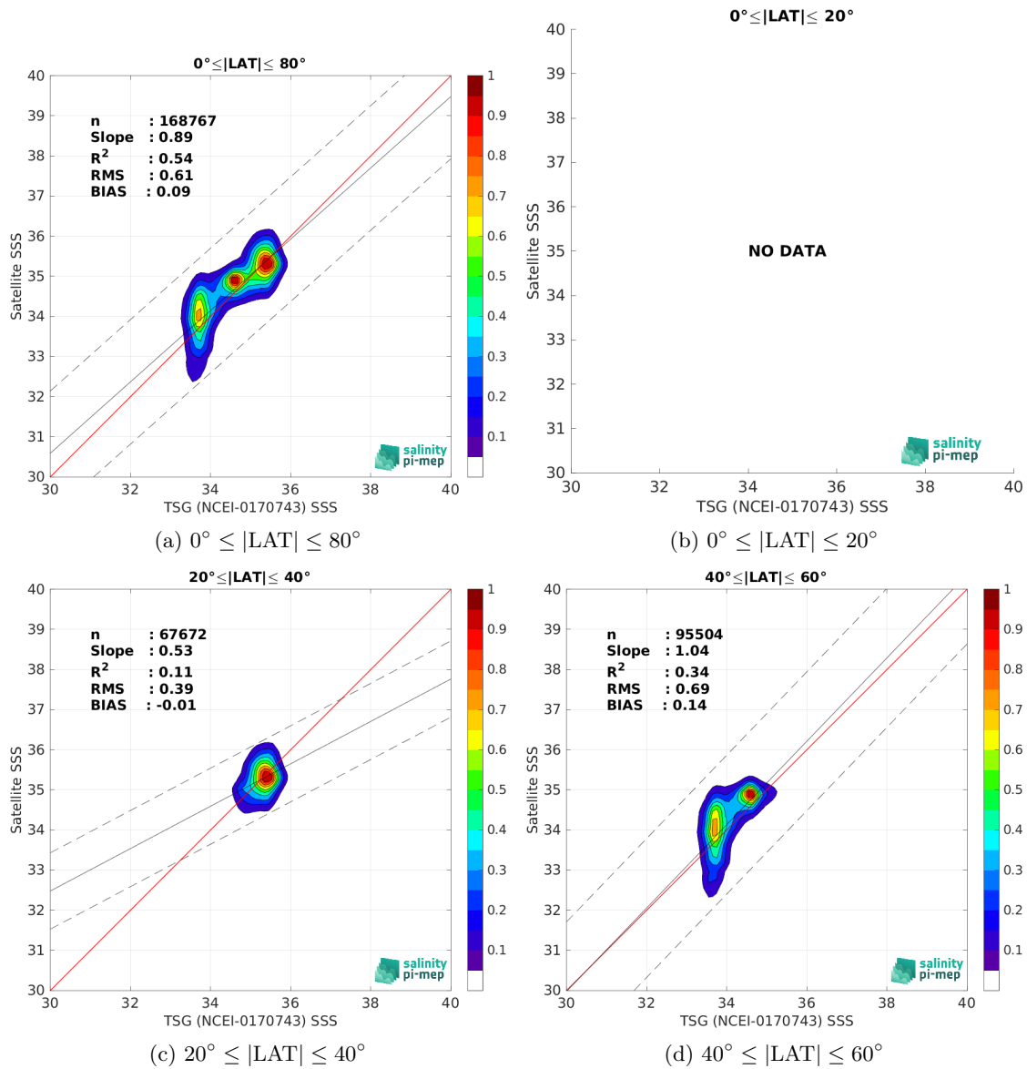
Figure 10: Contour maps of the concentration of SMAP SSS L3 v5.0 - 8-Day running (JPL) SSS (y-axis) versus TSG (NCEI-0170743) SSS (x-axis) at match-up pairs for different latitude bands. For each plot, the red line shows x=y . The black thin and dashed lines indicate a linear fit through the data cloud and the \pm 95\% confidence levels, respectively. The number match-up pairs n , the slope and R^2 coefficient of the linear fit, the root mean square (RMS) and the mean bias between satellite and in situ data are indicated for each latitude band in each plots.
